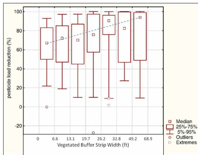
Figure 35. Effect of filter strip width on pesticide load reduction of moderately adsorbed compounds ( K_{oc} < 1000 ) in surface runoff. Data summarizes results of 217 studies. Adapted from Reichenberger et al., 1997.
