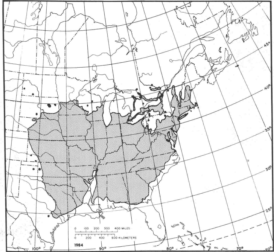
Figure 1—Natural range of eastern redcedar.
