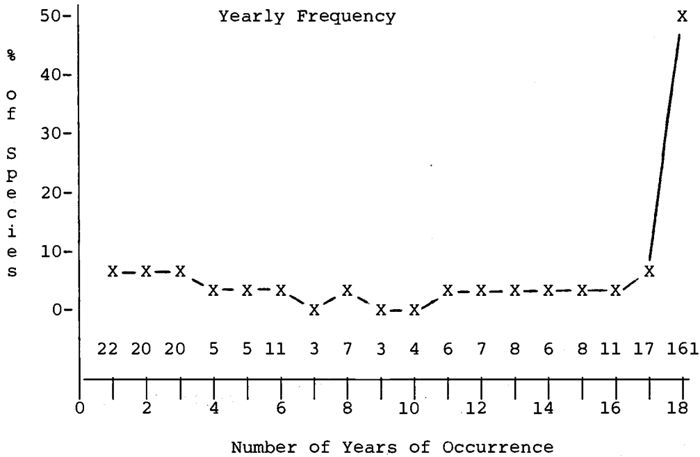
FIGURE 4.1. Percentage of 324 species seen live on or from land during 1973-1990 for each number of years of occurrence. The number of species is along the baseline. For example, about 50% (161) of the species were recorded each year, and less than 10% (6) were reported during 14 of the 18 years. This Figure is Fig. 1 in Bayer (1993b).
