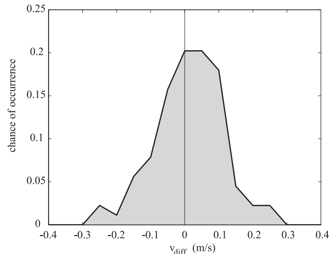
Figure 17. Probability density plot of the difference between mean surface and interior longshore currents, v_{diff} .
