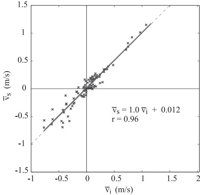
Figure 16. In situ longshore current means, \bar{v}_i , versus surface longshore current means, \bar{v}_s . A linear least squares regression is shown as the thick line, and a perfect fit 1:1 line is shown as the dashed line.
