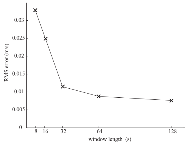
Figure 8. Total root mean square error for each window length, T_i , over all mean velocities and maximum orbital velocities.
