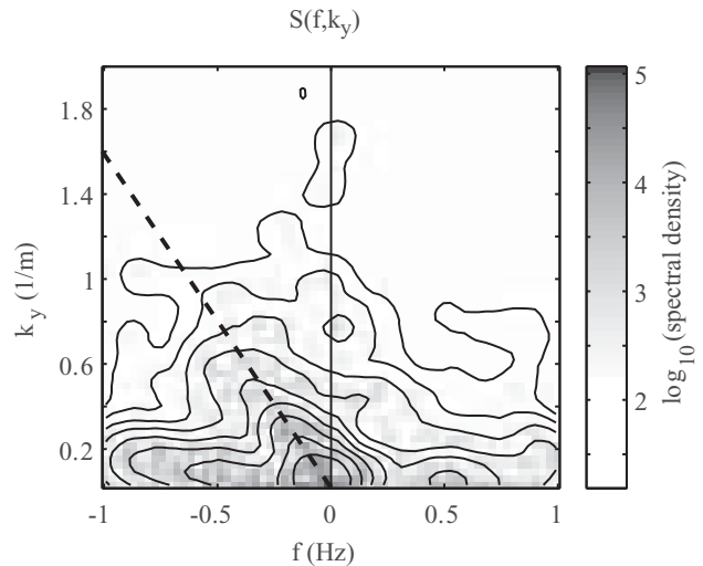
Figure 3. Frequency-wave number spectrum of the timestack in Figure 2. Note the concentration of energy along the dashed line corresponding to a constant velocity of -0.6 m/s.
