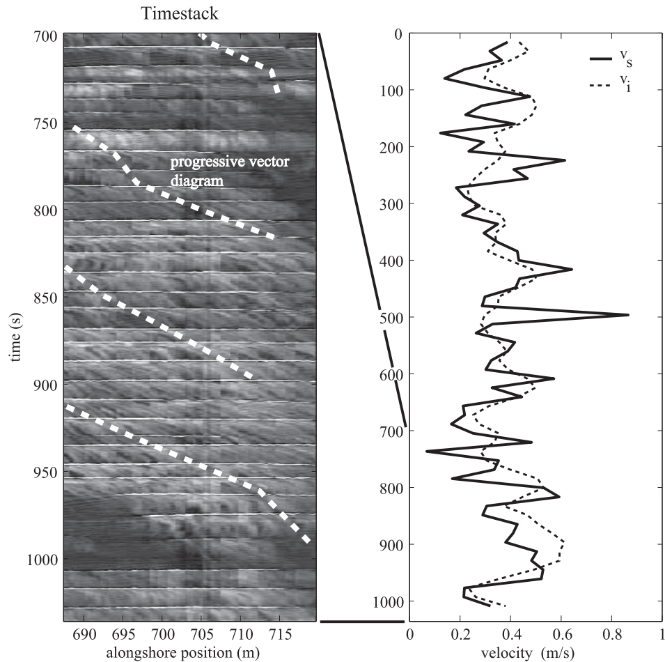
Figure 11. (left) Sample timestack with superimposed progressive vector diagram (PVD) and (right) alongshore current time series. The PVD is the stepwise-integrated surface velocity time series and shows good alignment with foam streaks. Note that the timestack and PVD are only a portion of the full 1024-s timestack. The data were taken on 4 November at 2034 GMT.
