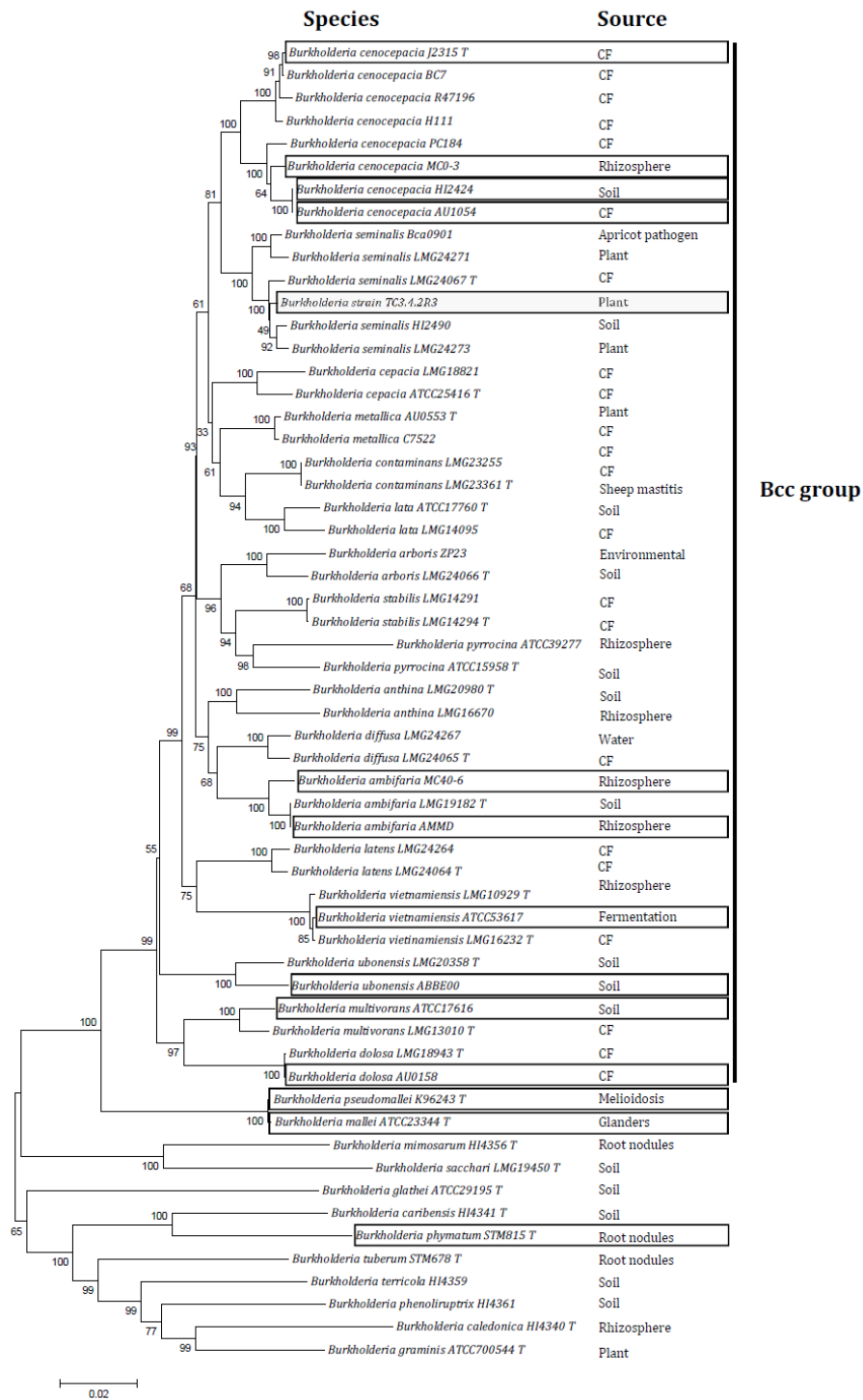
Figure S2. Multilocus sequence typing (MLST) of sugarcane endophytic Burkholderia sp. TC3.4.2R3. Unrooted neighbor-joining tree (Jukes & Kantor, 1969) based on MLST ( atpD , gltB , gyrB , recA , lepA , phaC trpB ) data of Burkholderia species. Type strains are designed with T after the name. The numbers in the branches indicate the bootstrap values, which were calculated after 1000 replications. The scale bar indicates 0.02 substitutions per nucleotide position.
