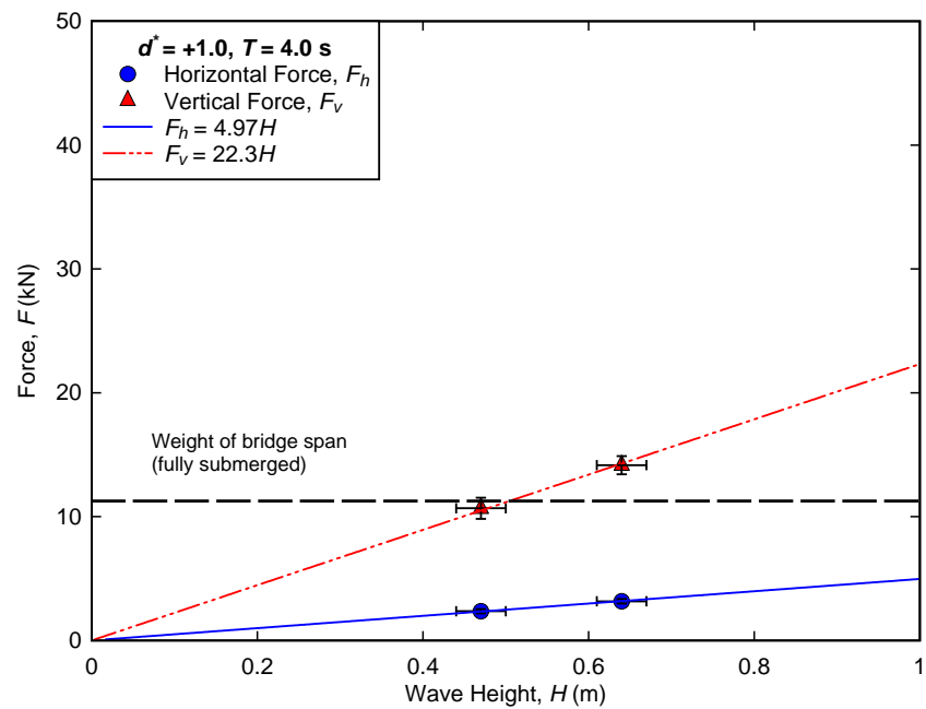
Figure B-29. Measured forces for regular wave trials conducted at d^* = +1.0 , T = 4.0\text{s} .
