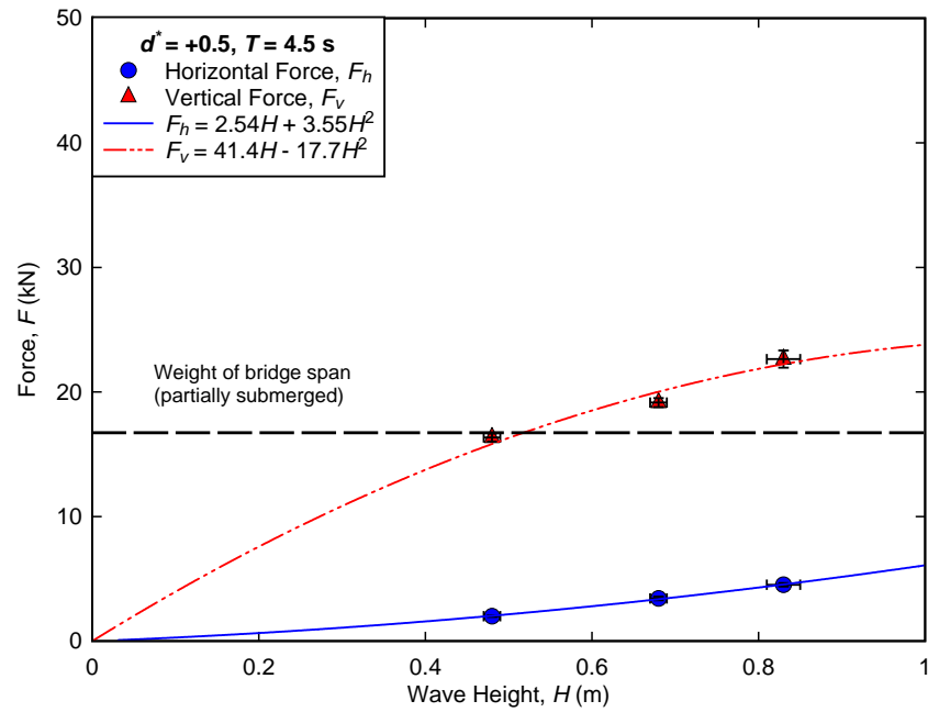
Figure B-24. Measured forces for regular wave trials conducted at d^* = +0.5 , T = 4.5\text{s} .
