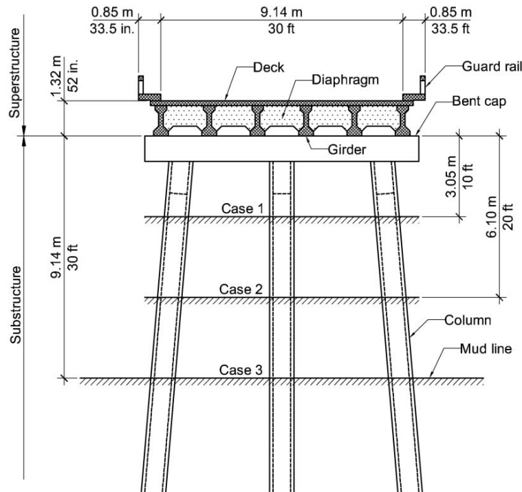
Figure 3-2. Elevation view of typical prototype bridge (courtesy of Thomas Schumacher, Oregon State University).
