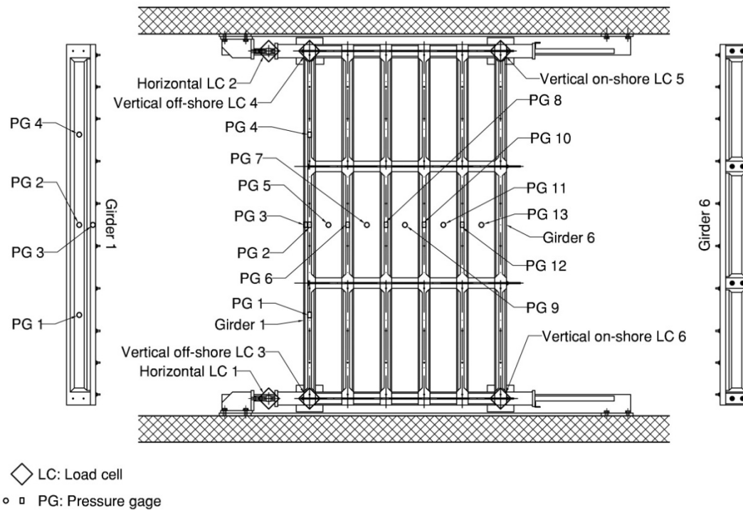
Figure 3-10. Instrumentation plan for pressure gages and load cells; plan view (deck not shown for clarity). Courtesy of Thomas Schumacher, Oregon State University.
