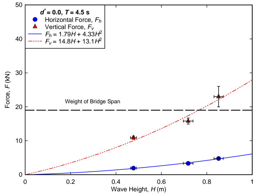
Figure B-18. Measured forces for regular wave trials conducted at d^* = 0.0, T = 4.5 \text{ s} .
