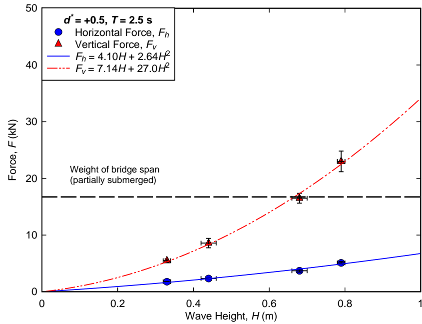
Figure B-20. Measured forces for regular wave trials conducted at d^* = +0.5 , T = 2.5 s.
