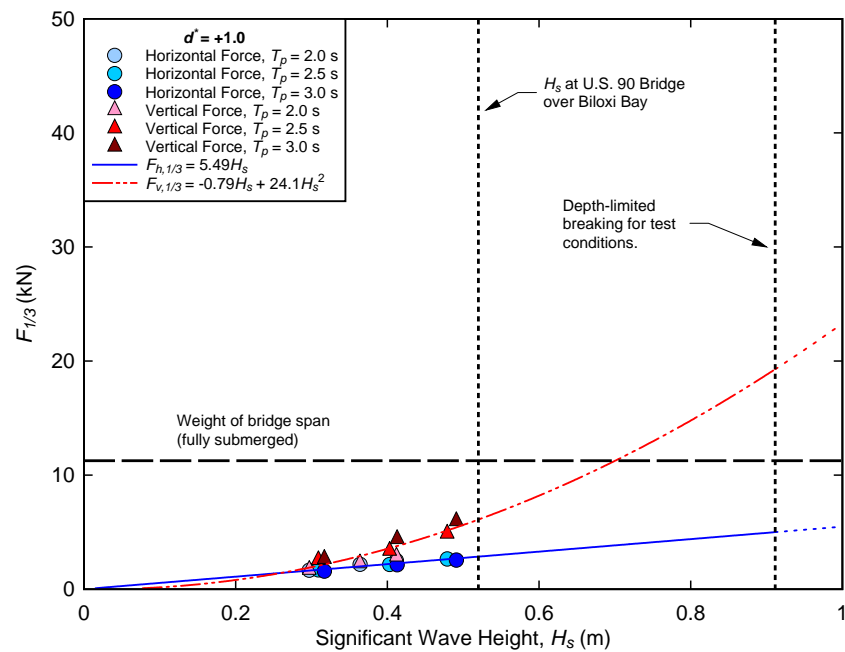
Figure F-5. Force vs. wave height for random wave trials, d^* = +1.0 .
