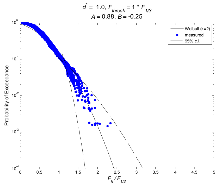
Figure H-17. Exceedance probability for normalized horizontal forces, d^* = +1.0
