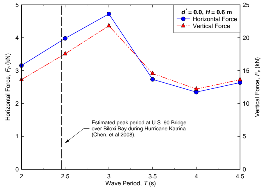
Figure E-3. Effect of wave period on forces for regular waves, d^* = 0.0 .
