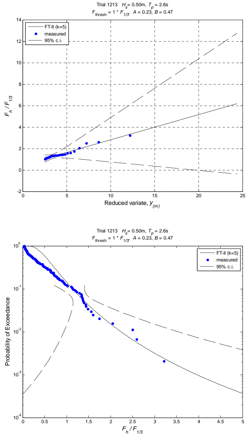
Figure H-1. Exceedance probabilities for normalized horizontal forces, d^* = -0.5 , H_s = 0.50\text{ m} , T_p = 2.6\text{ s} .
