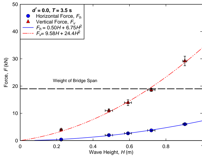
Figure 5-7. Measured forces for regular wave trials conducted at d^* = 0.0 , T = 3.5 s.
