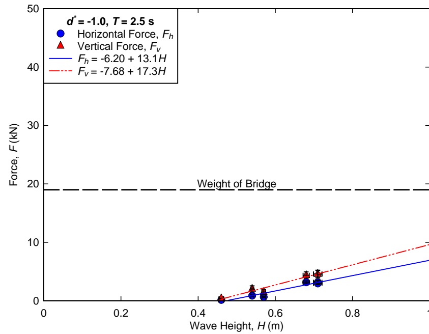
Figure B-2. Measured forces for regular wave trials conducted at d^* = -1.0 , T = 2.5 s.
