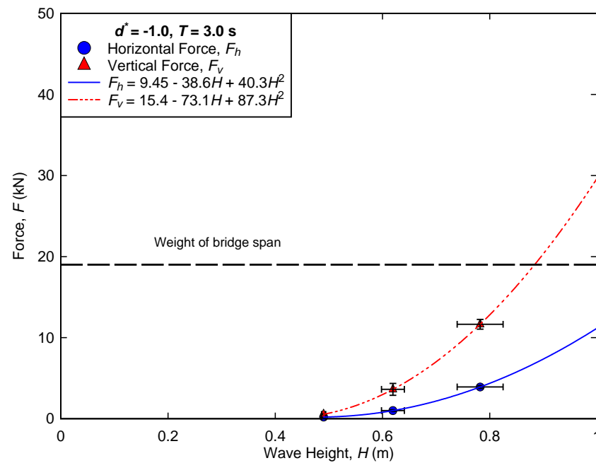
Figure B-3. Measured forces for regular wave trials conducted at d^* = -1.0 , T = 3.0 s.
