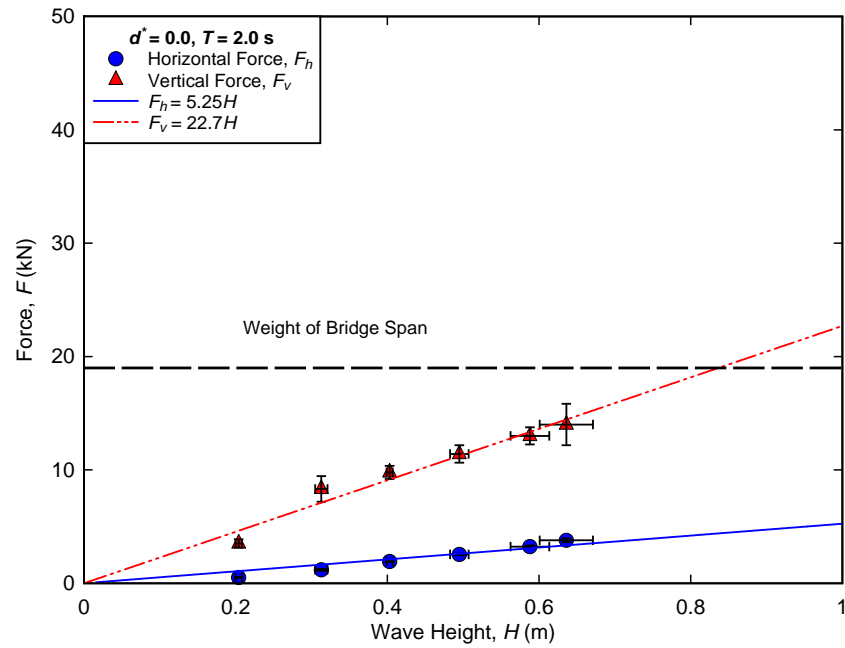
Figure B-13. Measured forces for regular wave trials conducted at d^* = 0.0 , T = 2.0 \text{ s} .
