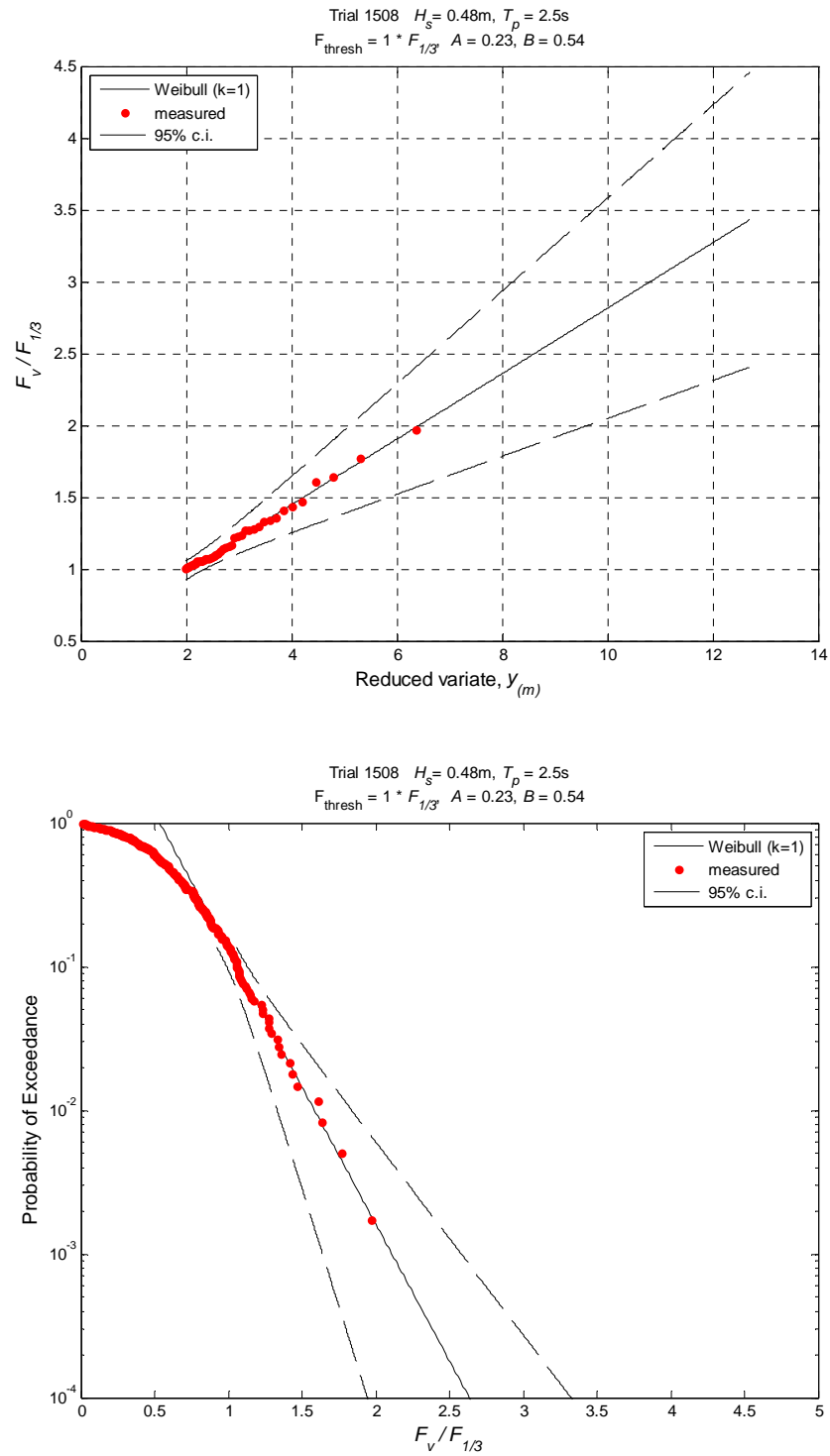
Figure H-8. Exceedance probabilities for normalized vertical forces, d^* = +1.0 , H_s = 0.48\text{ m} , T_p = 2.5\text{s} .
