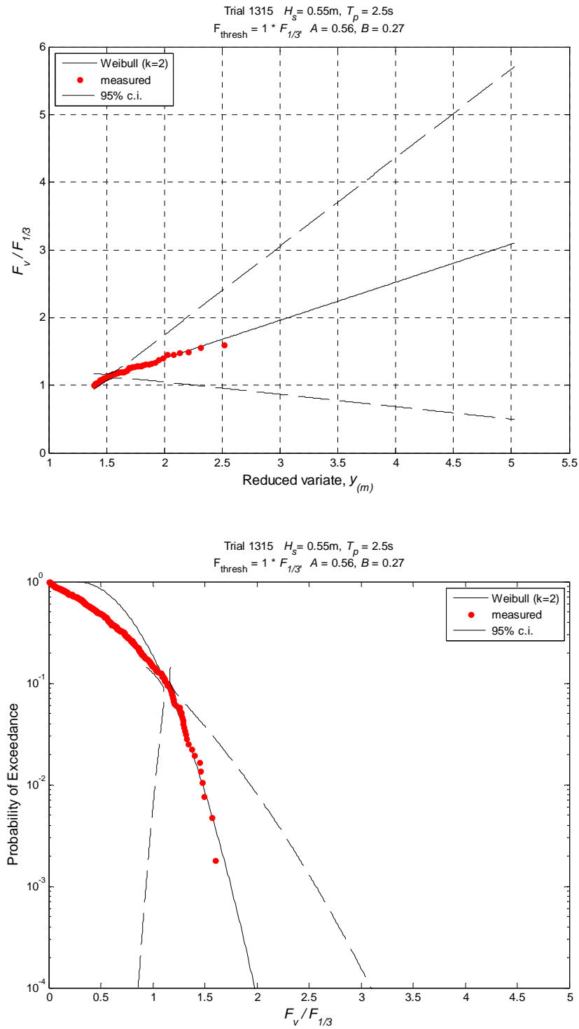
Figure H-4. Exceedance probabilities for normalized vertical forces, d^* = 0.0 , H_s = 0.55\text{ m} , T_p = 2.5\text{s} .
