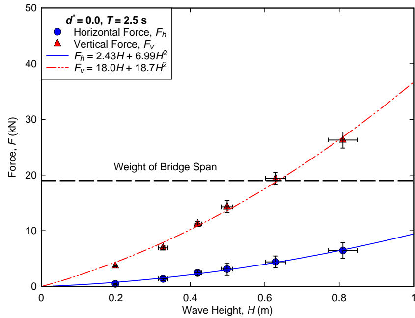
Figure B-14. Measured forces for regular wave trials conducted at d^* = 0.0, T = 2.5 \text{ s} .
