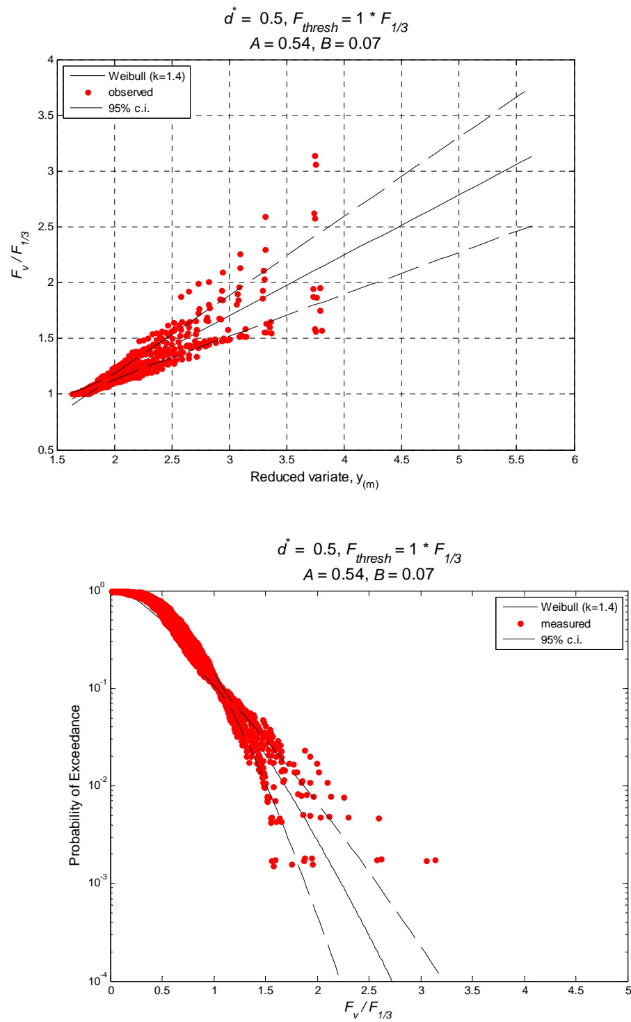
Figure H-16. Exceedance probability for normalized vertical forces, d^* = +0.5
