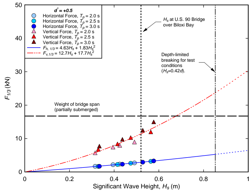
Figure F-4. Force vs. wave height for random wave trials, d^* = +0.5 .
