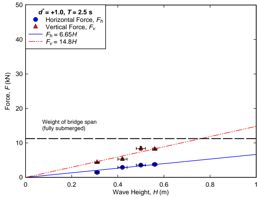
Figure B-26. Measured forces for regular wave trials conducted at d^* = +1.0 , T = 2.5\text{s} .
