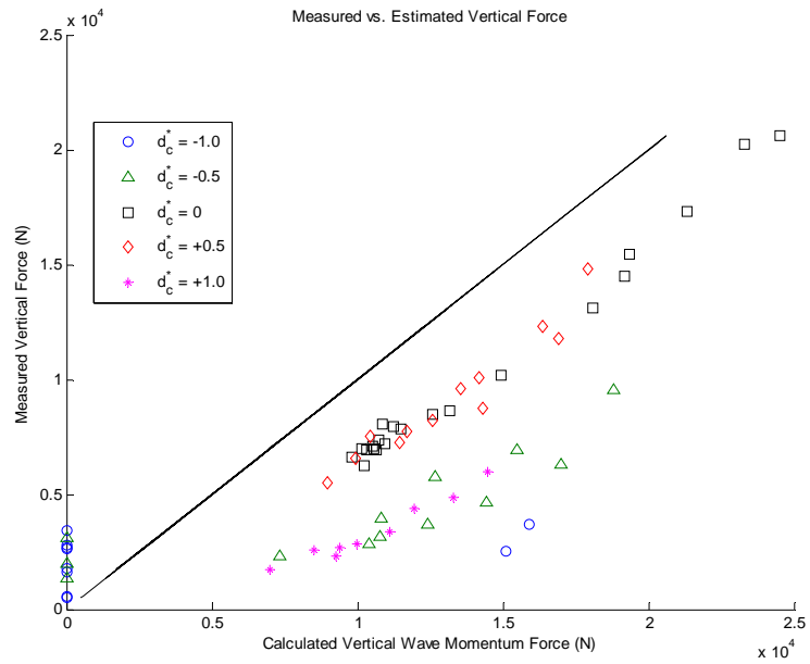
Figure 6-10. Measured vs. calculated vertical force, F_{v,l/3} , for random wave trials.
