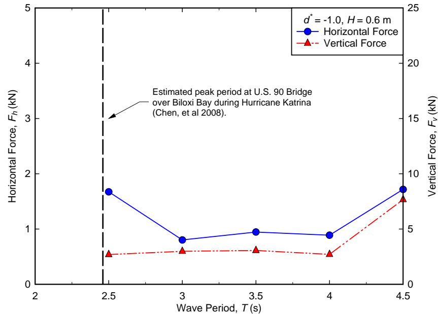
Figure E-1. Effect of wave period on forces for regular waves, d^* = -1.0 .
