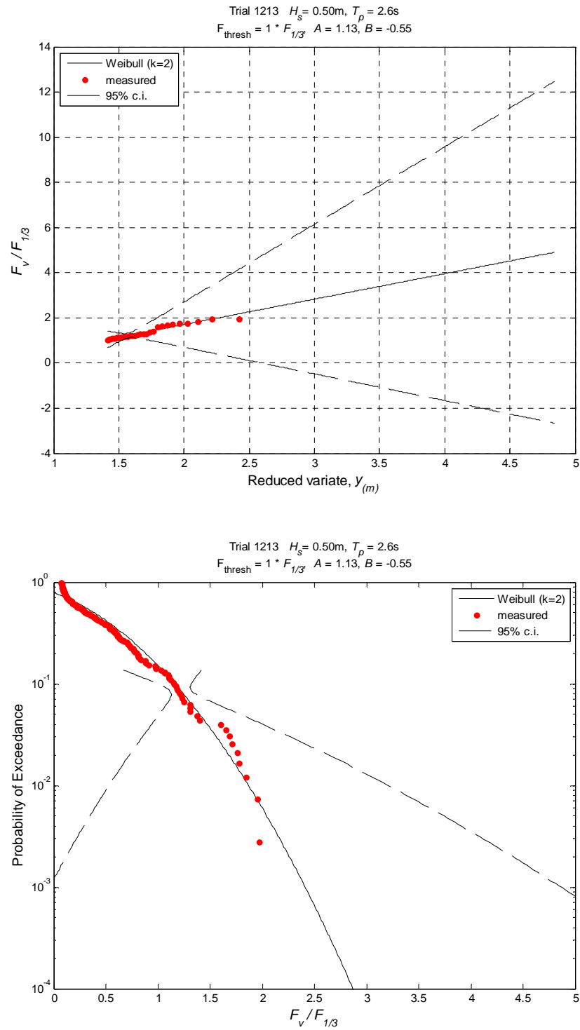
Figure H-2. Exceedance probabilities for normalized vertical forces, d^* = -0.5 , H_s = 0.50\text{ m} , T_p = 2.6\text{s} .
