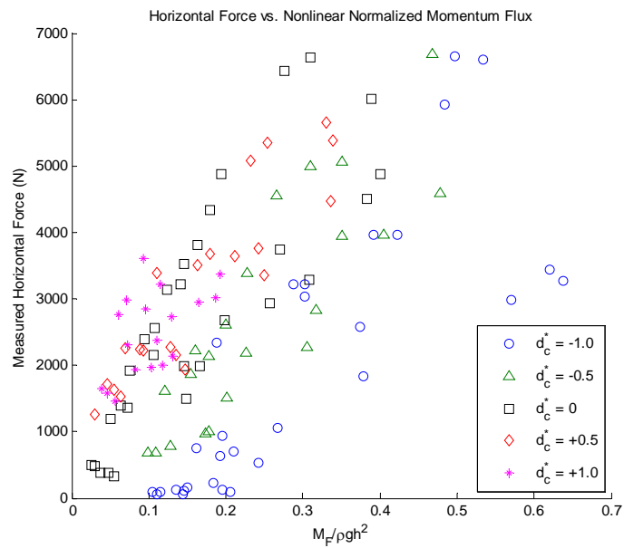
Figure 6-2. Measured horizontal force vs. nonlinear wave momentum flux parameter for regular wave trials.
