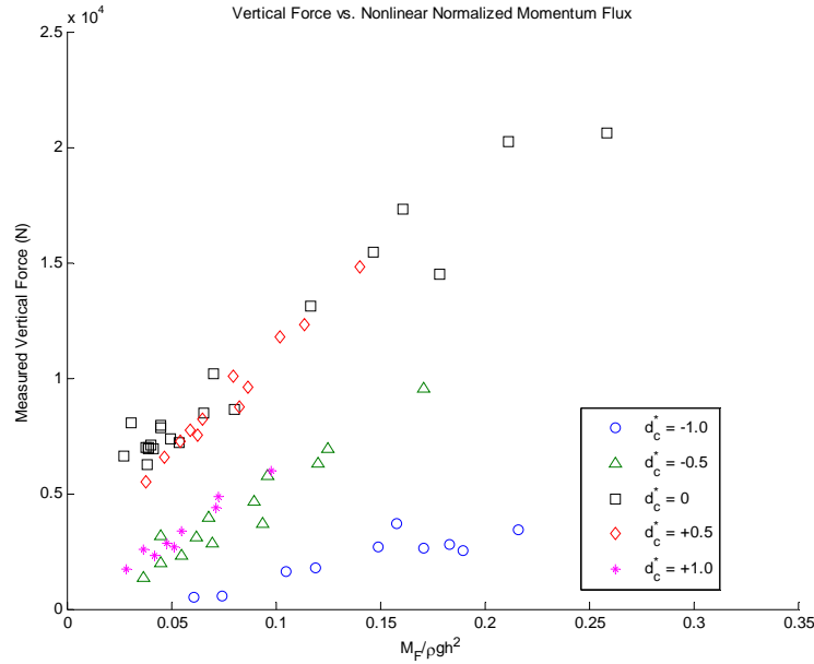
Figure 6-6. Measured F_{v,l/3} vs. nonlinear wave momentum flux parameter for random wave trials.
