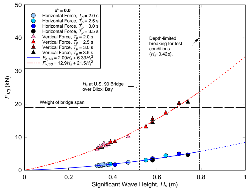
Figure F-3. Force vs. wave height for random wave trials, d^* = 0.0 .
