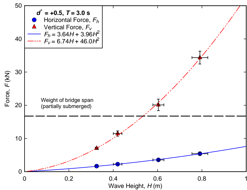
Figure B-21. Measured forces for regular wave trials conducted at d^* = +0.5 , T = 3.0 s.
