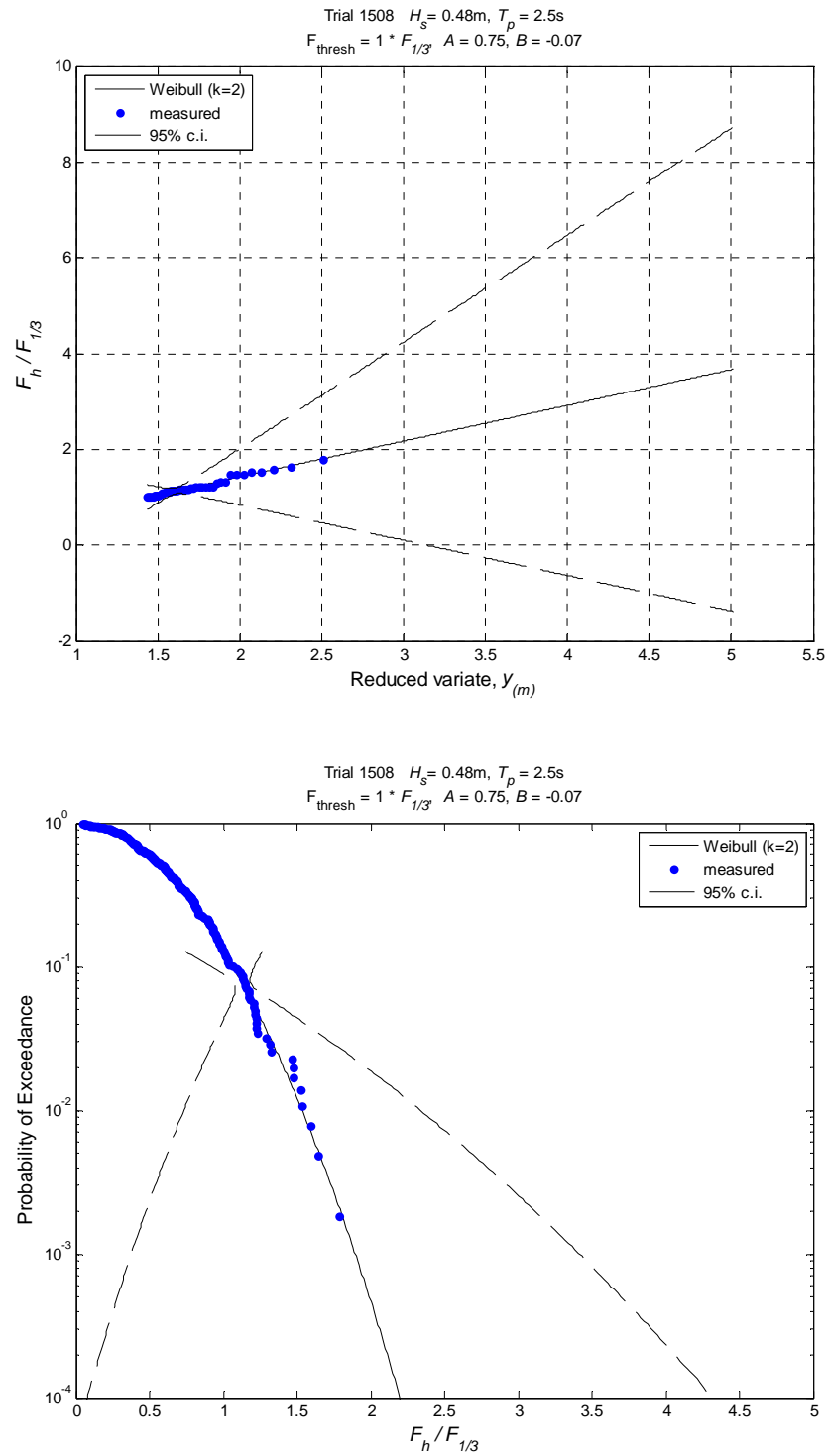
Figure H-7. Exceedance probabilities for normalized horizontal forces, d^* = +1.0 , H_s = 0.48\text{m} , T_p = 2.5\text{s} .
