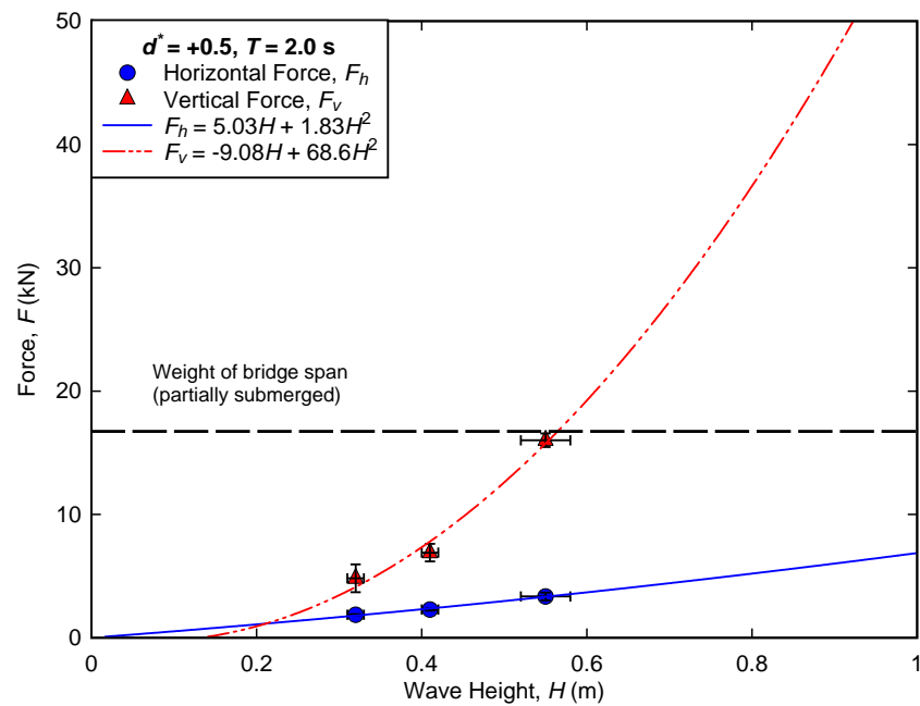
Figure B-19. Measured forces for regular wave trials conducted at d^* = +0.5, T = 2.0 \text{ s} .
