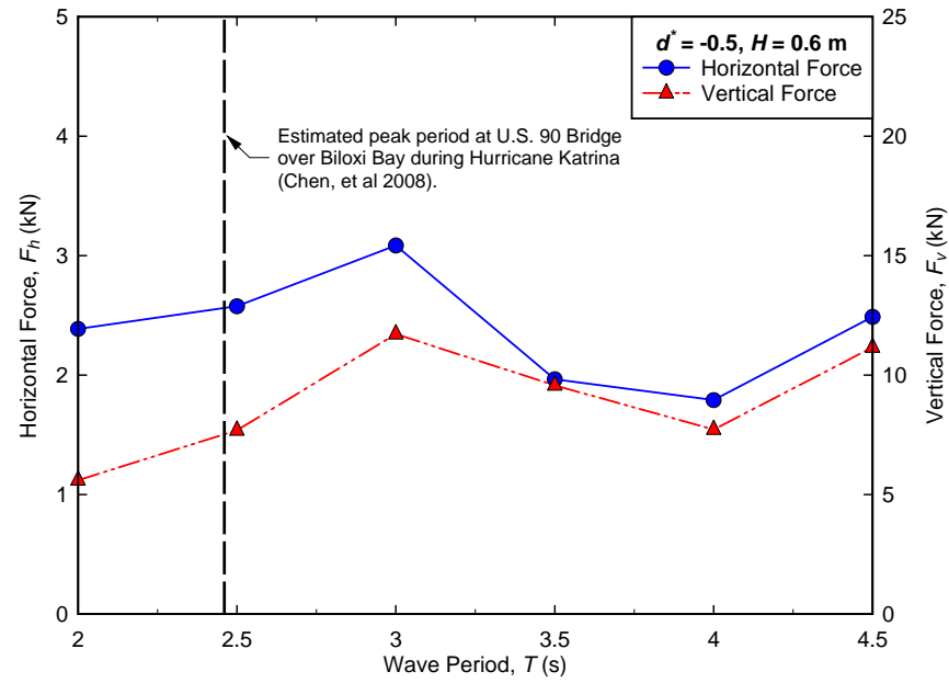
Figure E-2. Effect of wave period on forces for regular waves, d^* = -0.5 .
