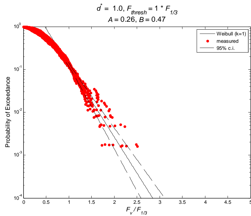
Figure H-18. Exceedance probability for normalized vertical forces, d^* = +1.0
