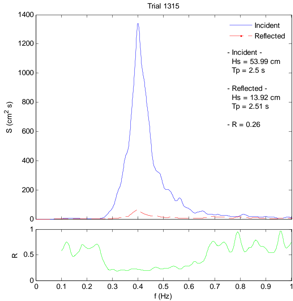
Figure 4-7. Frequency spectrum and corresponding reflection coefficient for random wave trial 1315.
