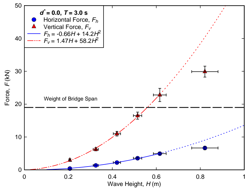
Figure B-15. Measured forces for regular wave trials conducted at d^* = 0.0, T = 3.0 \text{ s} .
