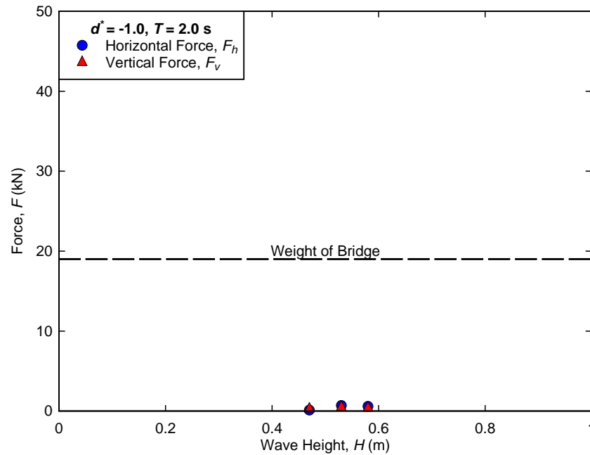
Figure B-1. Measured forces for regular wave trials conducted at d^* = -1.0, T = 2.0 s.
