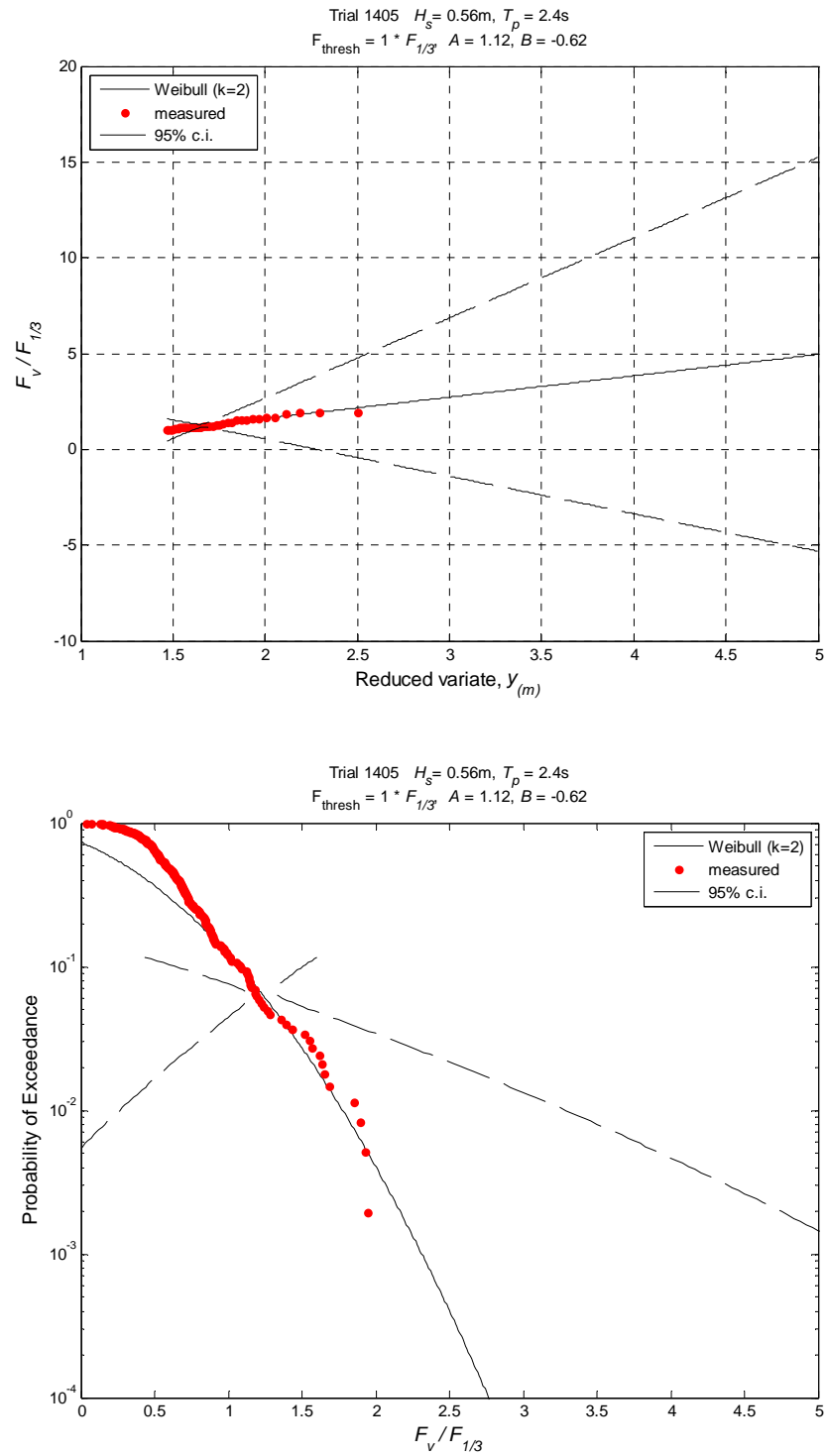
Figure H-6. Exceedance probabilities for normalized vertical forces, d^* = +0.5 , H_s = 0.56\text{ m} , T_p = 2.4\text{ s} .
