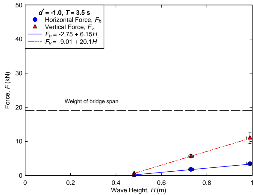
Figure B-4. Measured forces for regular wave trials conducted at d^* = -1.0, T = 3.5 \text{ s} .
