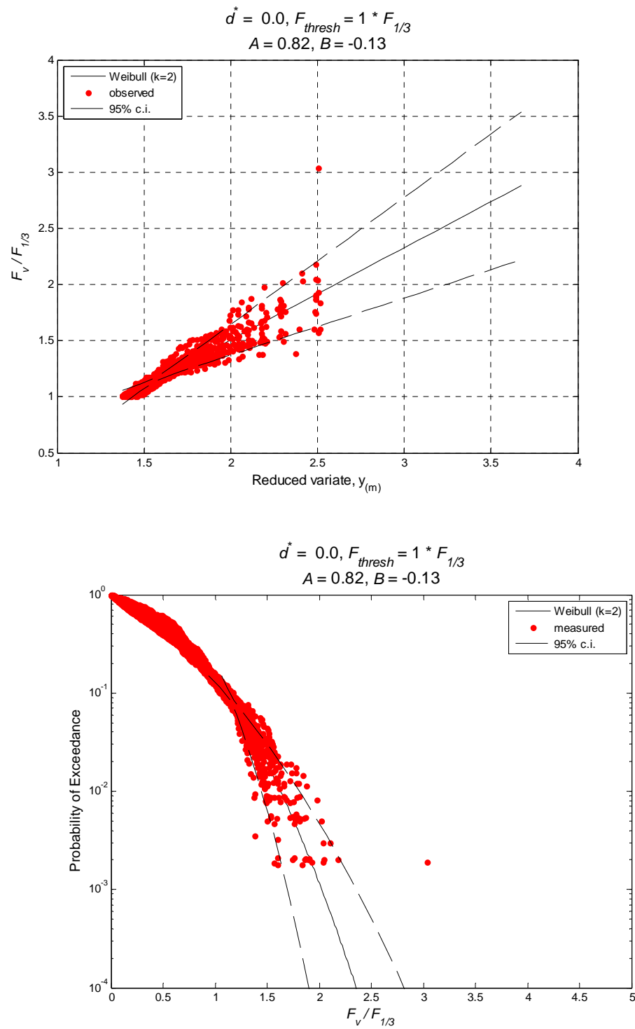
Figure H-14. Exceedance probability for normalized vertical forces, d^* = 0.0
