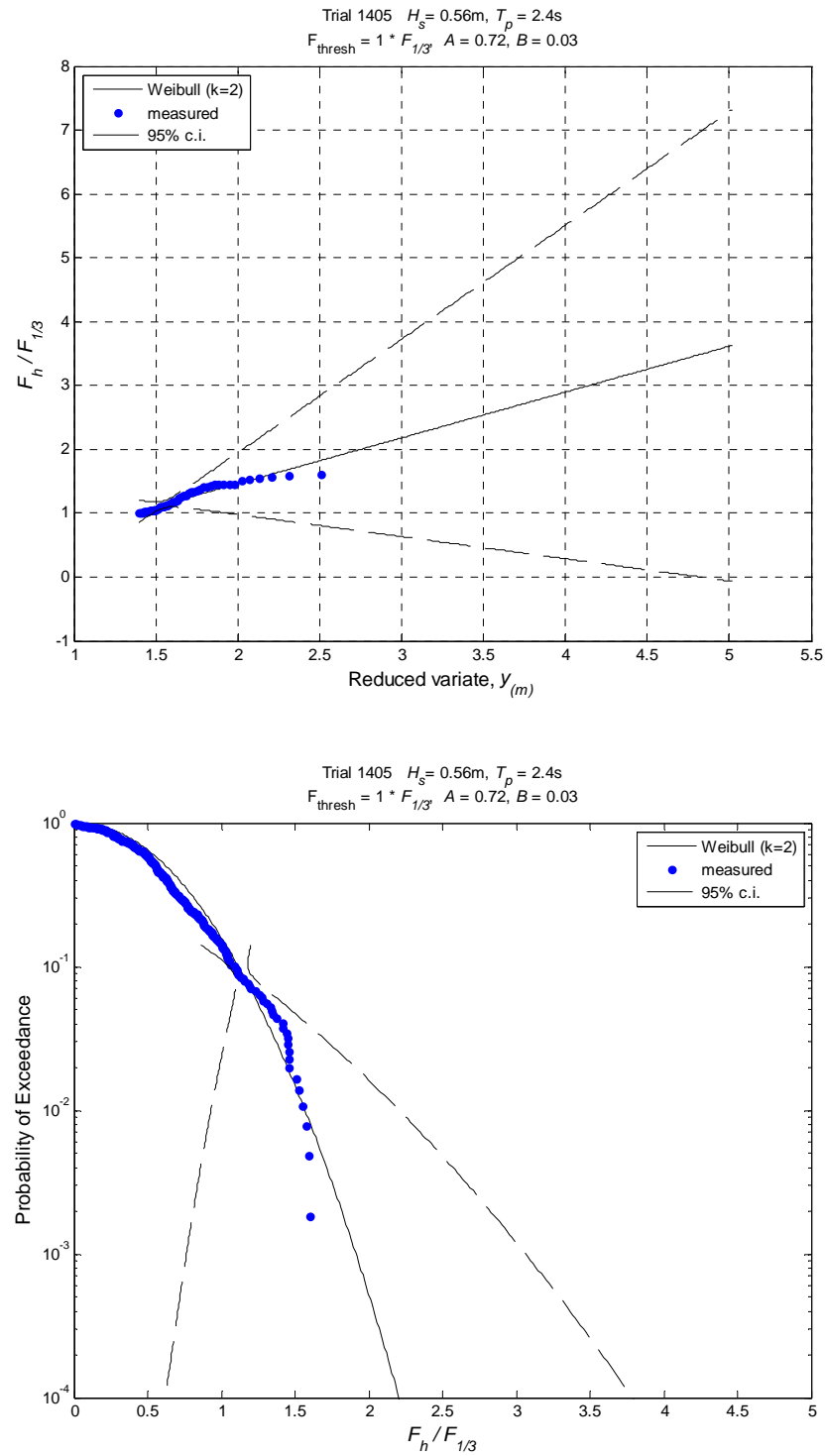
Figure H-5. Exceedance probabilities for normalized horizontal forces, d^* = +0.5 , H_s = 0.56 m, T_p = 2.4 s.
