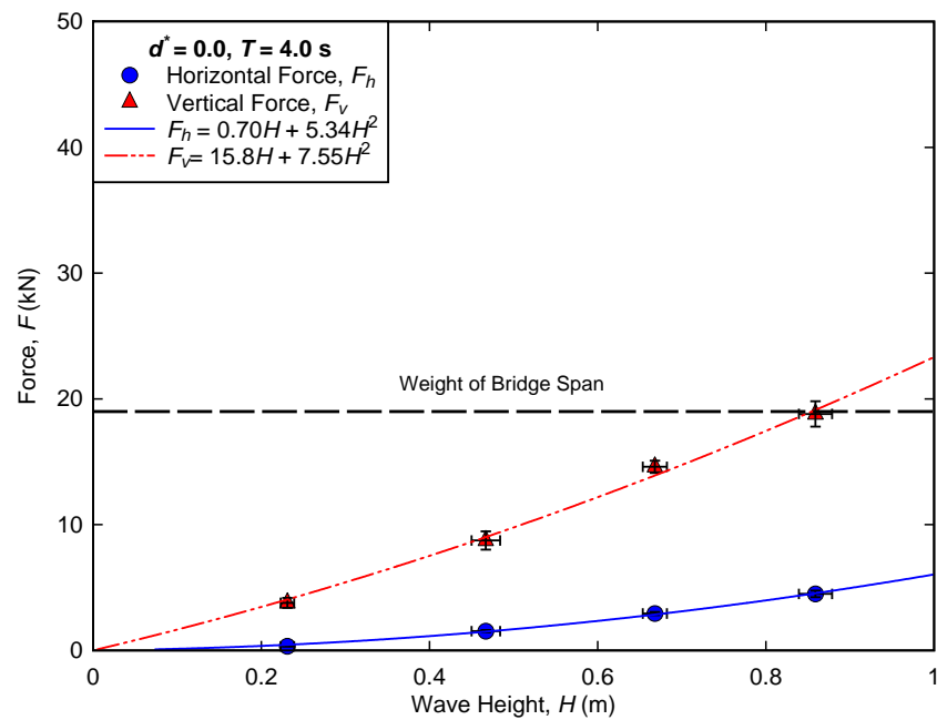
Figure B-17. Measured forces for regular wave trials conducted at d^* = 0.0, T = 4.0 \text{ s} .
