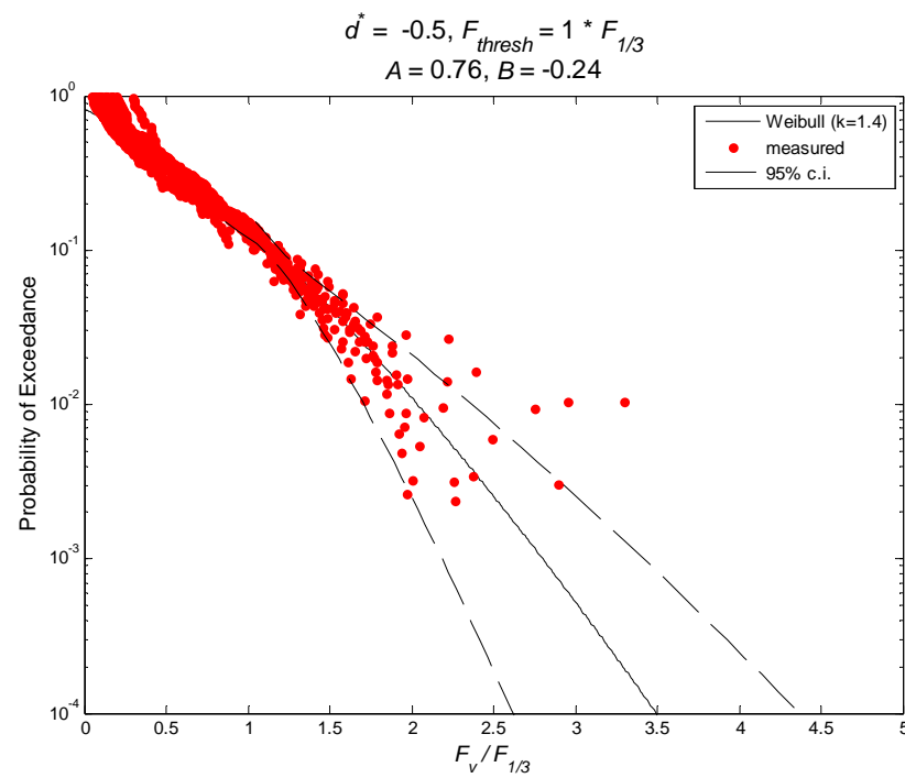
Figure H-12. Exceedance probability for normalized vertical forces, d^* = -0.5 .
