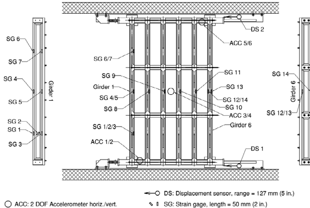
Figure 3-11. Instrumentation plan for strain gages, displacement sensors, and accelerometers; plan view (deck not shown for clarity). Courtesy of Thomas Schumacher, Oregon State University.
