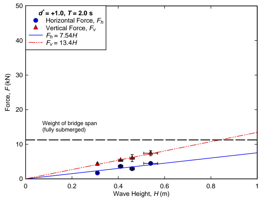
Figure B-25. Measured forces for regular wave trials conducted at d^* = +1.0 , T = 2.0\text{s} .
