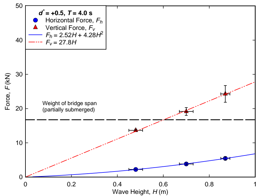
Figure B-23. Measured forces for regular wave trials conducted at d^* = +0.5 , T = 4.0\text{s} .
