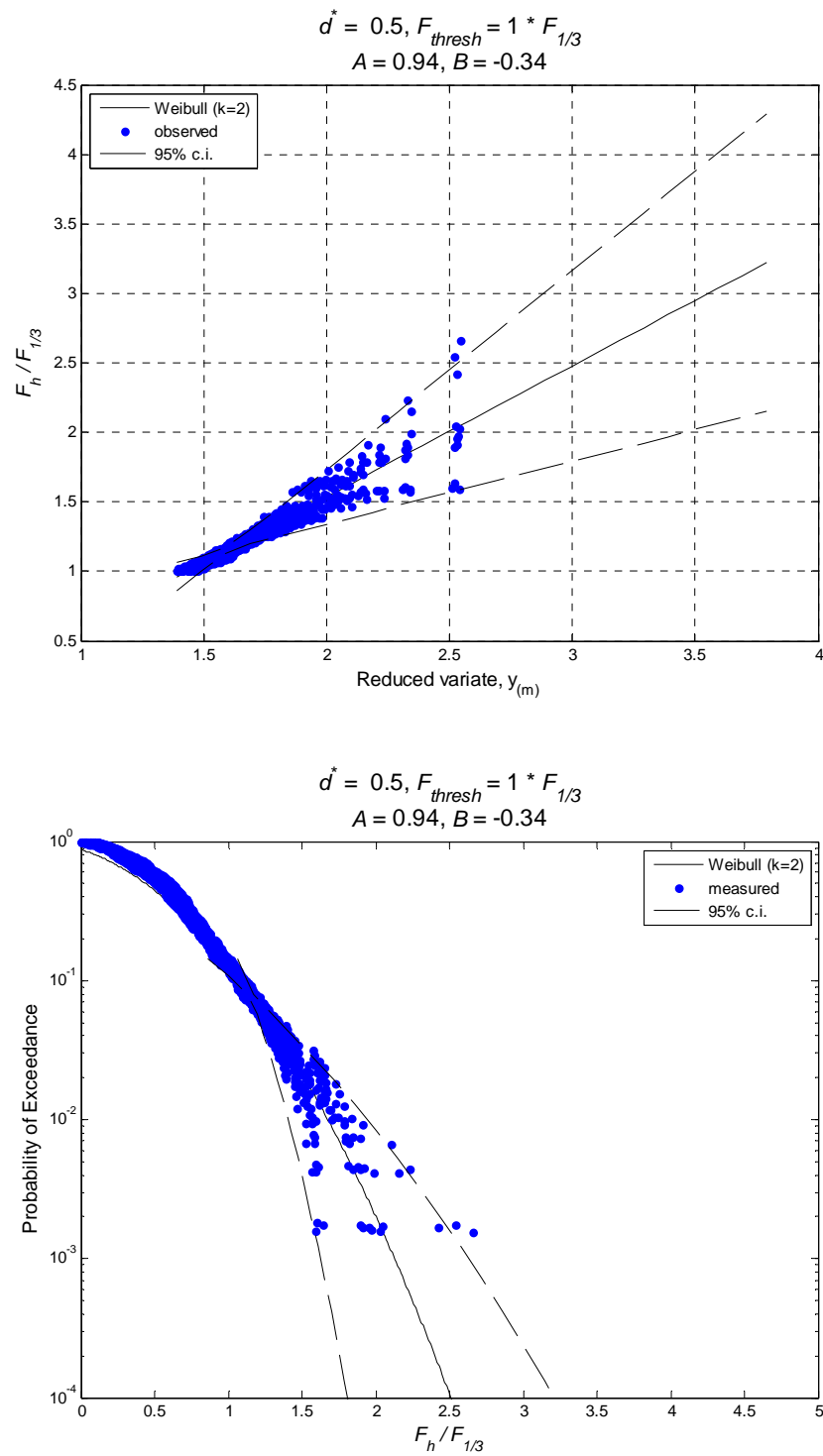
Figure H-15. Exceedance probability for normalized horizontal forces, d^* = +0.5
