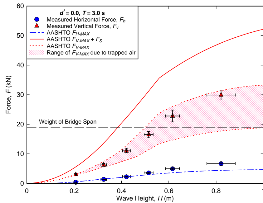
Figure G-7. Comparison of AASHTO guidelines with measured forces, d^* = 0.0 , T = 3.0 s.
