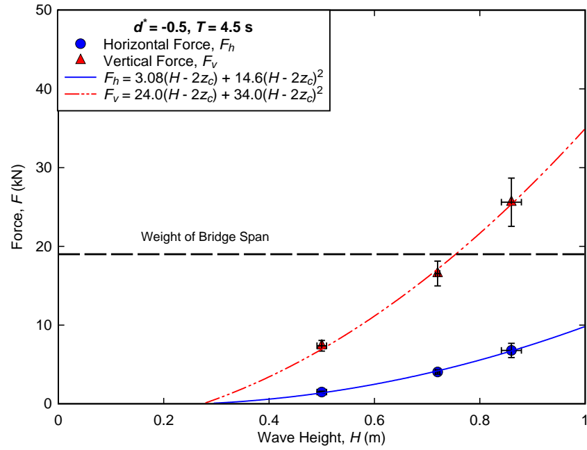
Figure B-12. Measured forces for regular wave trials conducted at d^* = -0.5 , T = 4.5 \text{ s} .
