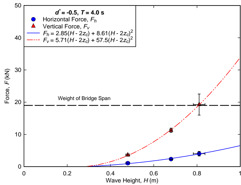
Figure B-11. Measured forces for regular wave trials conducted at d^* = -0.5, T = 4.0\text{s} .
