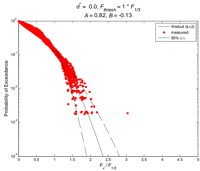
Figure 8-3. Exceedance probability for normalized horizontal forces (top) and vertical forces (bottom), d^* = 0.0
