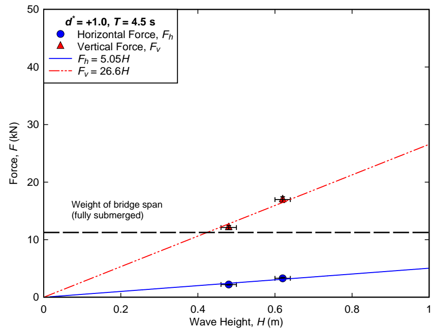
Figure B-30. Measured forces for regular wave trials conducted at d^* = +1.0 , T = 4.5 s.
