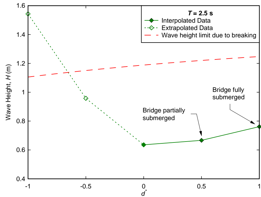
Figure D-2. Minimum wave height to overcome weight of superstructure, T = 2.5 s.
