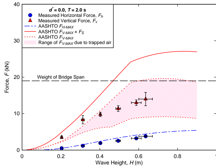
Figure G-6. Comparison of AASHTO guidelines with measured forces, d^* = 0.0 , T = 2.0 s.
