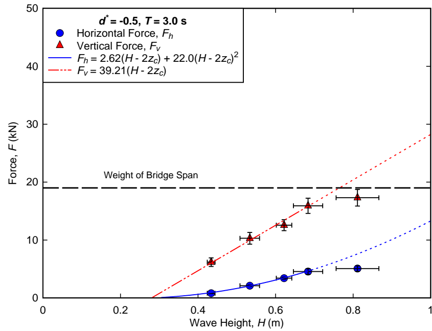
Figure B-9. Measured forces for regular wave trials conducted at d^* = -0.5, T = 3.0 \text{ s} .
