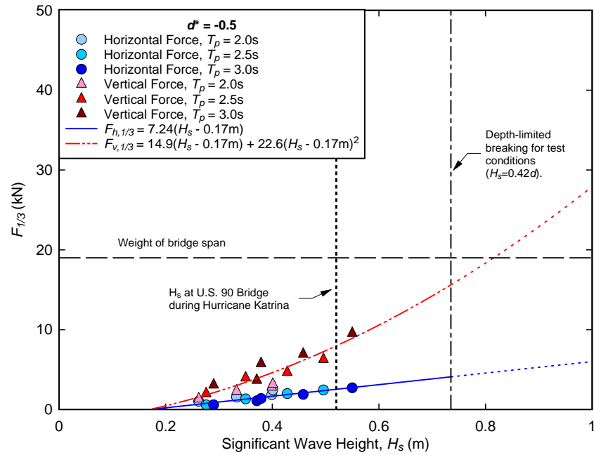
Figure F-2. Force vs. wave height for random wave trials, d^* = -0.5 .
