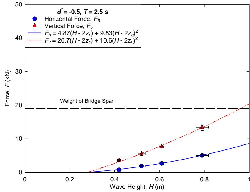
Figure B-8. Measured forces for regular wave trials conducted at d^* = -0.5, T = 2.5 \text{ s} .
