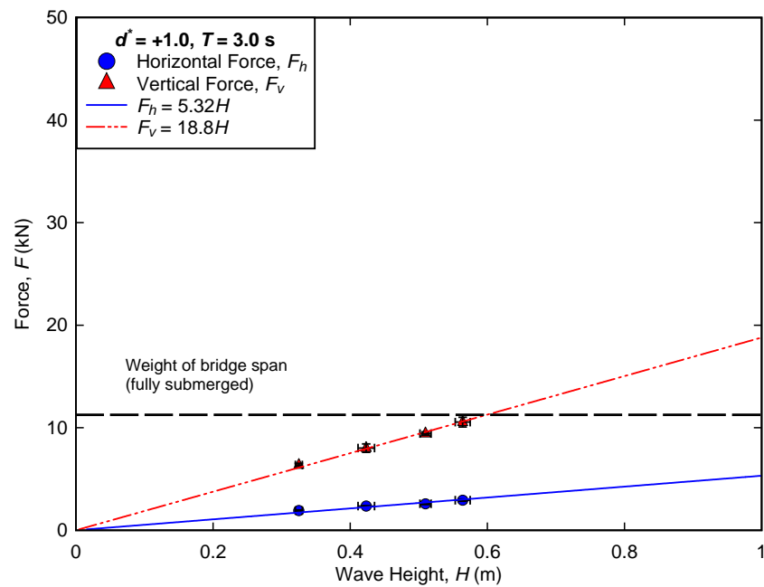
Figure B-27. Measured forces for regular wave trials conducted at d^* = +1.0 , T = 3.0\text{s} .
