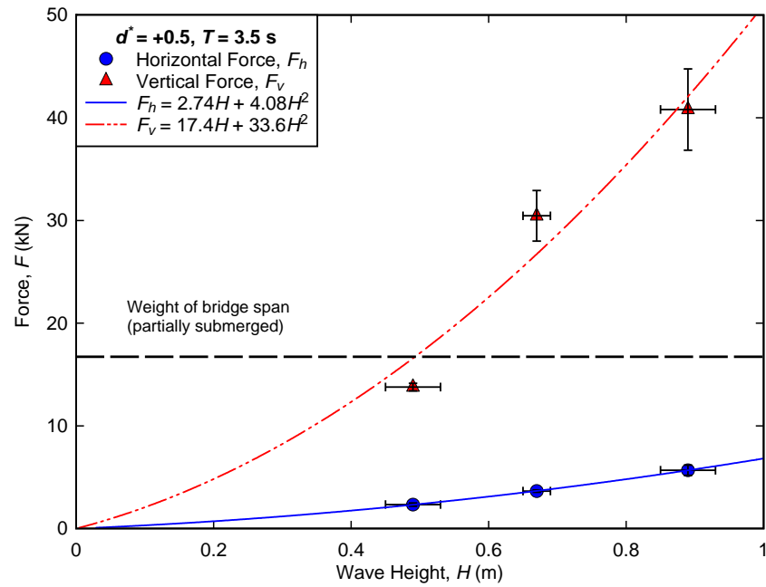
Figure B-22. Measured forces for regular wave trials conducted at d^* = +0.5 , T = 3.5\text{s} .
