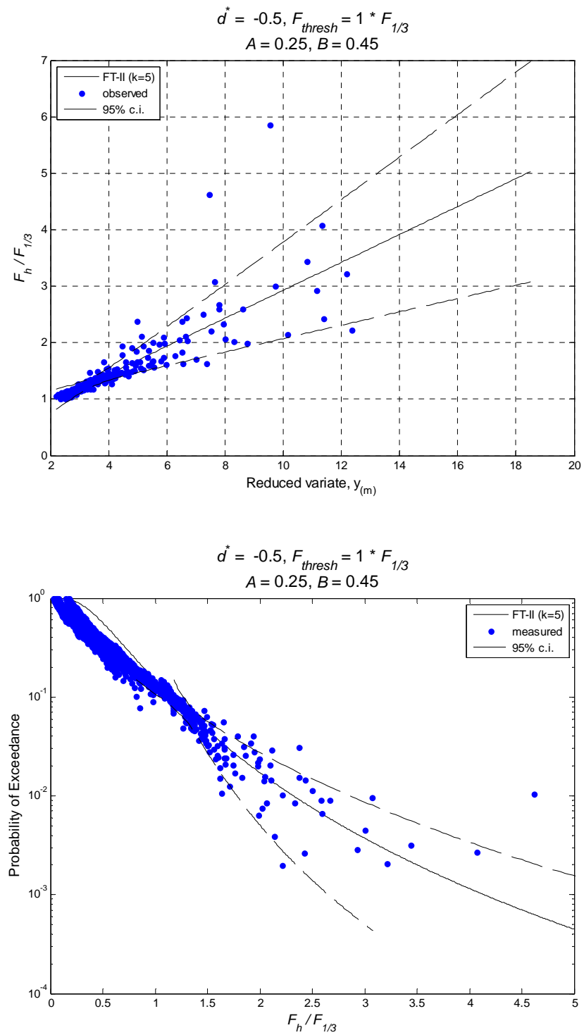
Figure H-11. Exceedance probability for normalized horizontal forces, d^* = -0.5 .
