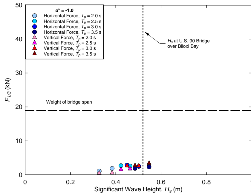
Figure F-1. Force vs. wave height for random wave trials, d^* = -1.0 .
