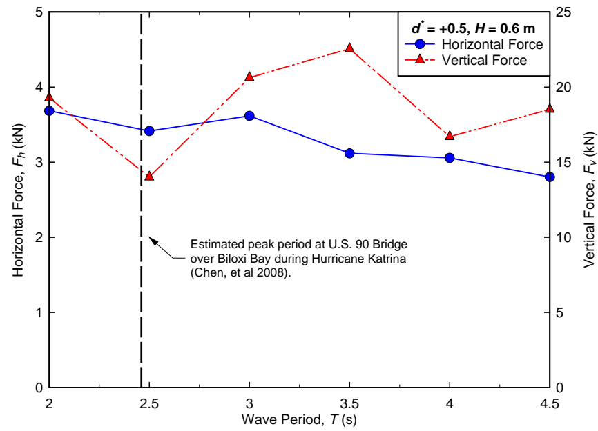
Figure E-4. Effect of wave period on forces for regular waves, d^* = +0.5 .
