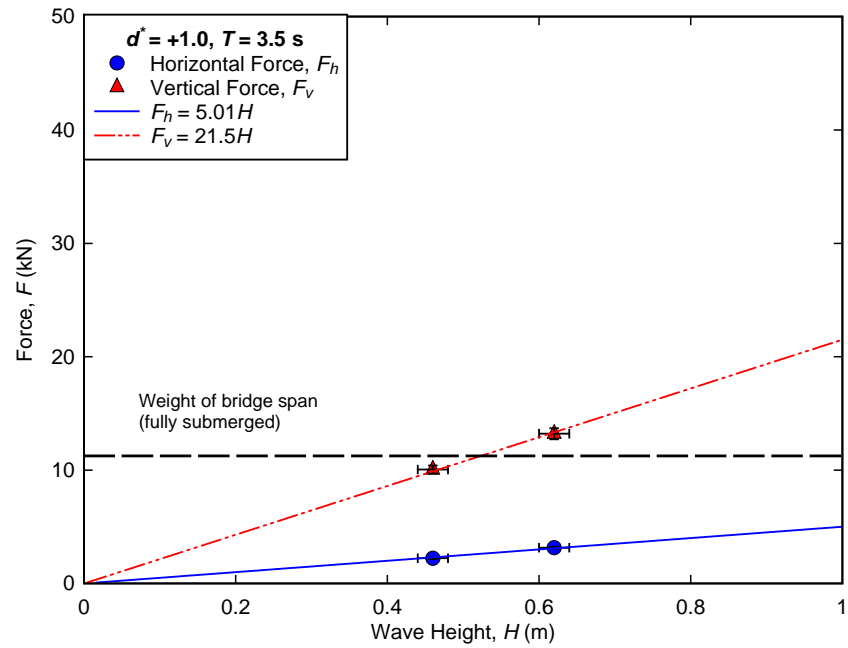
Figure B-28. Measured forces for regular wave trials conducted at d^* = +1.0 , T = 3.5\text{s} .
