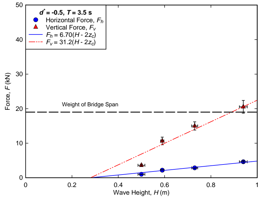
Figure B-10. Measured forces for regular wave trials conducted at d^* = -0.5, T = 3.5\text{s} .
