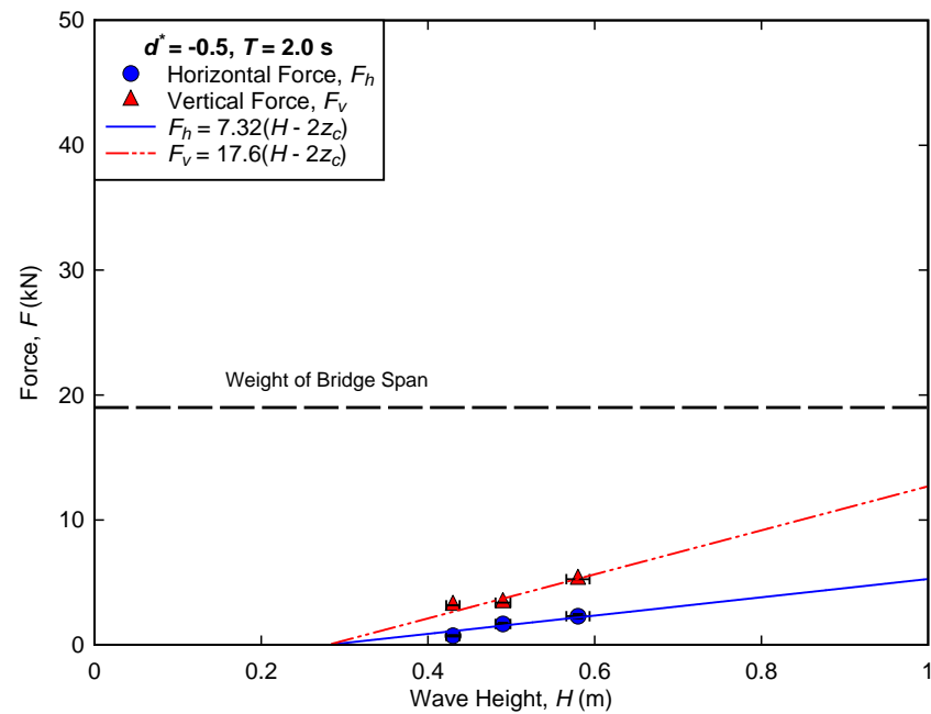
Figure B-7. Measured forces for regular wave trials conducted at d^* = -0.5 , T = 2.0 \text{ s} .
