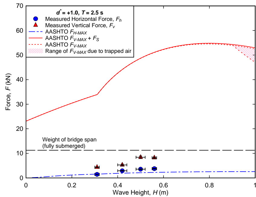
Figure G-5. Comparison of AASHTO guidelines with measured forces, d^* = +1.0 , T = 2.5 s.
