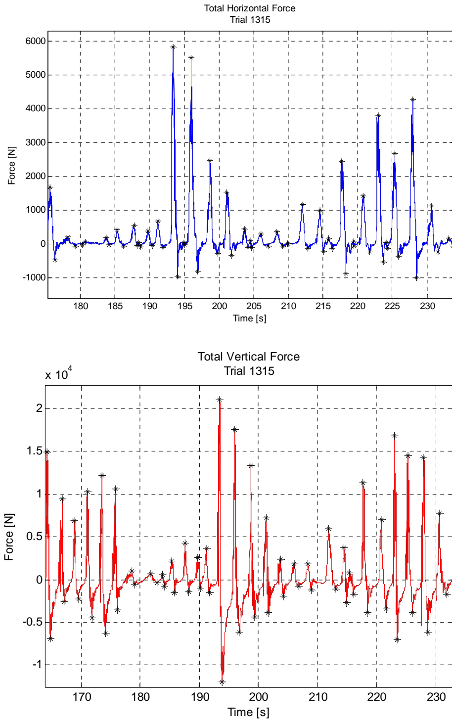
Figure 4-13. Expanded portion of horizontal (top) and vertical (bottom) times series for random wave trial 1315. Markers represent peak forces.
