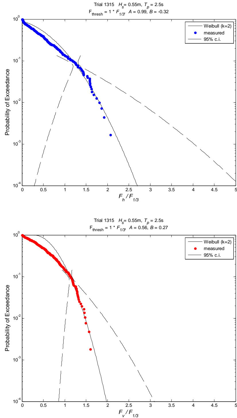
Figure 8-1. Exceedance probabilities for normalized horizontal (top) and vertical (bottom) forces for random wave trial 1315 ( d^* = 0 , H_s = 0.55 m, T_p = 2.5 s).
