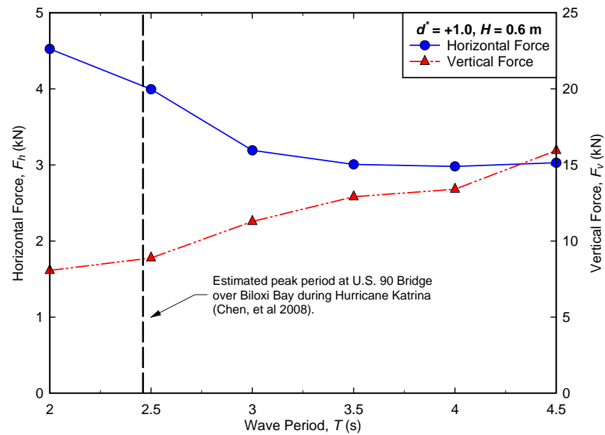
Figure E-5. Effect of wave period on forces for regular waves, d^* = +1.0 .
