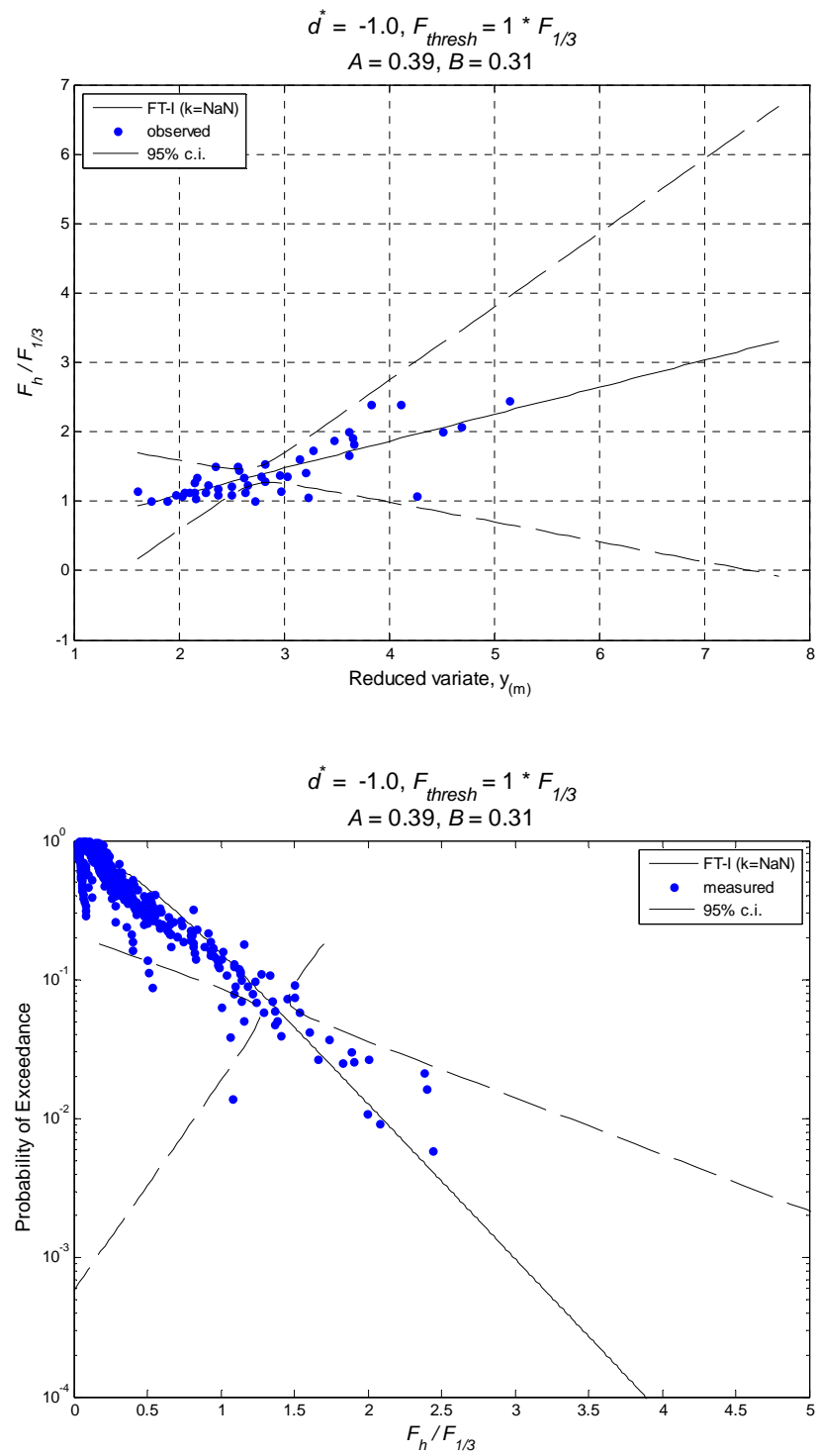
Figure H-9. Exceedance probability for normalized horizontal forces, d^* = -1.0
