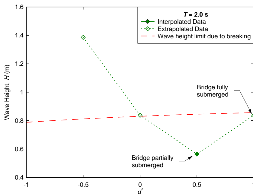
Figure D-1. Minimum wave height to overcome weight of superstructure, T = 2.0 s.
