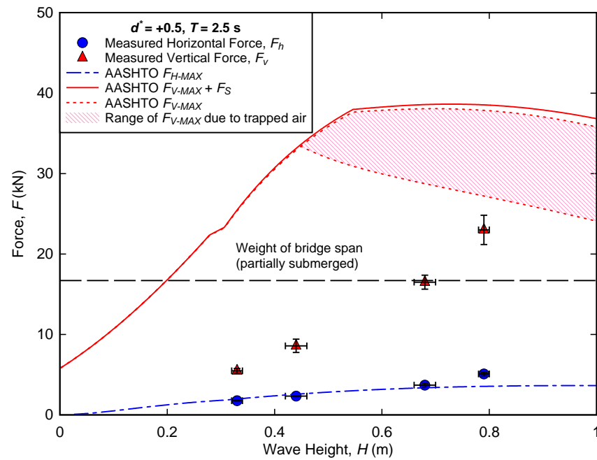
Figure 7-3. Comparison of AASHTO guidelines with measured forces, d^* = +0.5 , T = 2.5 s.
