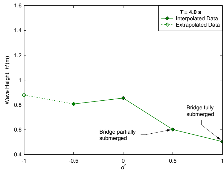
Figure D-5. Minimum wave height to overcome weight of superstructure, T = 4.0 \text{ s} .
