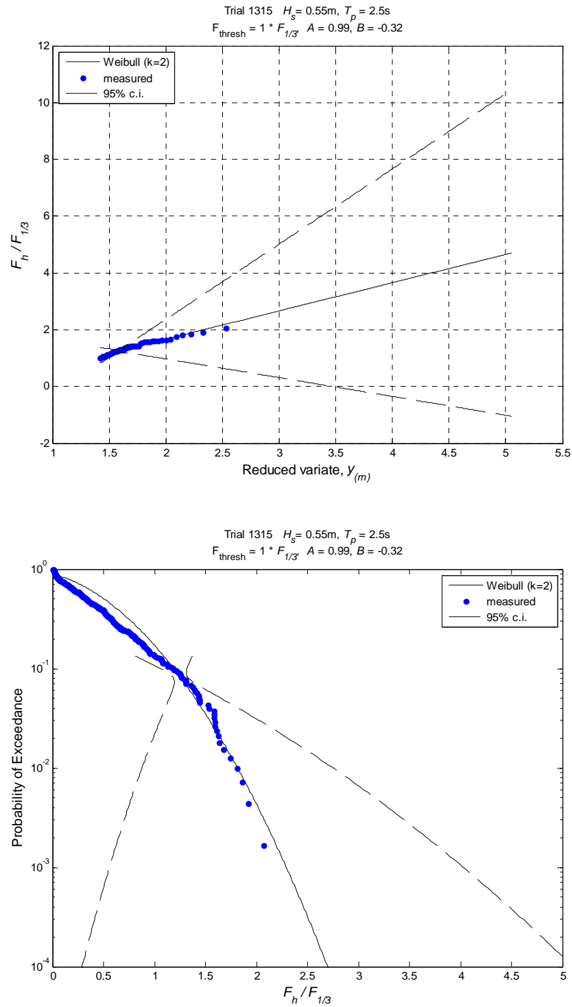
Figure H-3. Exceedance probabilities for normalized horizontal forces, d^* = 0.0 , H_s = 0.55 m, T_p = 2.5 s.
