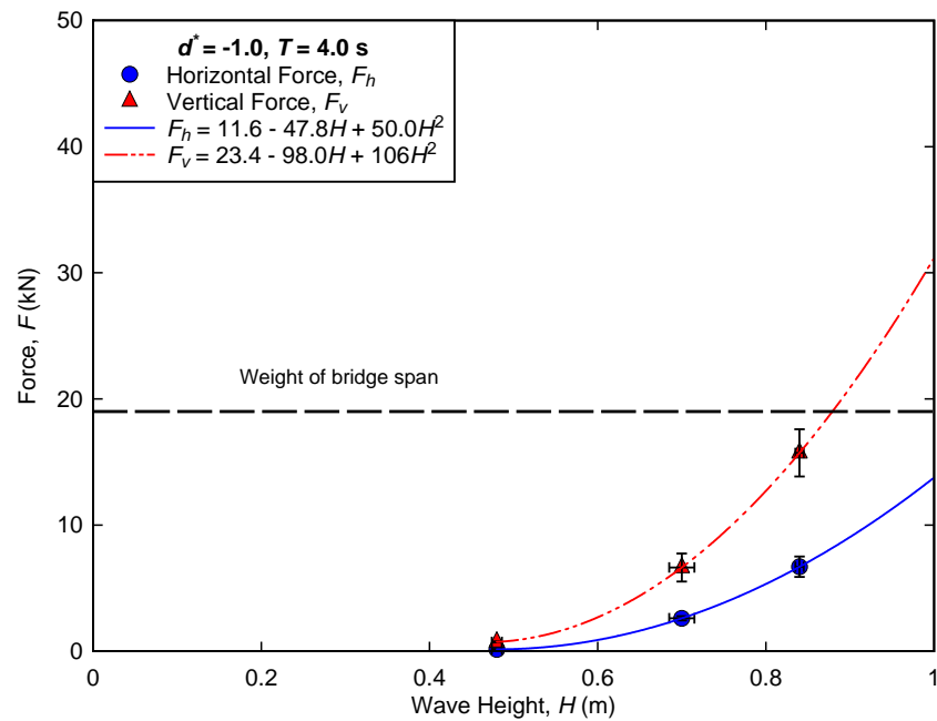
Figure B-5. Measured forces for regular wave trials conducted at d^* = -1.0, T = 4.0 \text{ s} .
