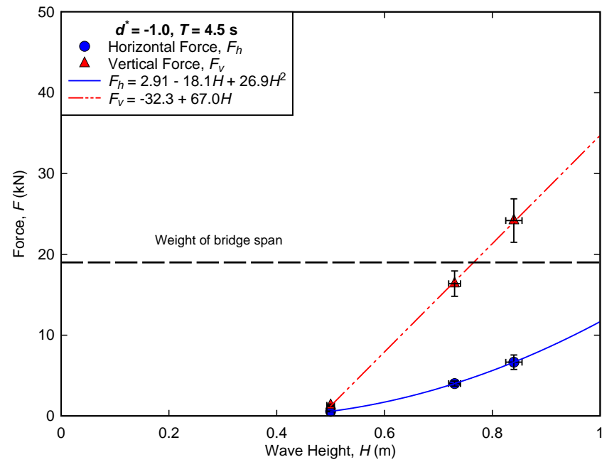
Figure B-6. Measured forces for regular wave trials conducted at d^* = -1.0 , T = 4.5 \text{ s} .
