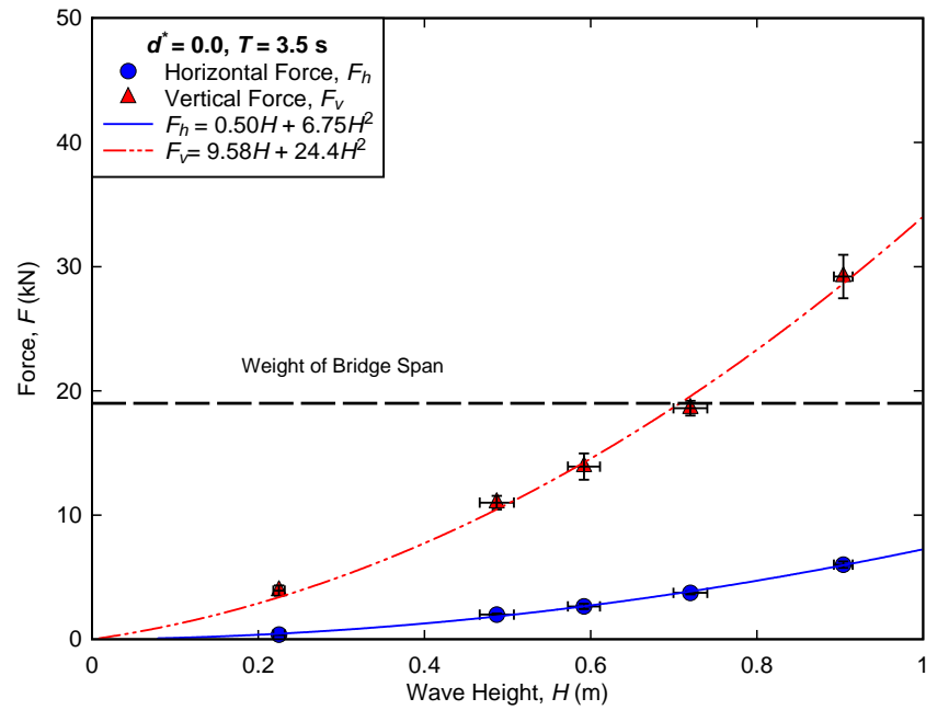
Figure B-16. Measured forces for regular wave trials conducted at d^* = 0.0, T = 3.5 \text{ s} .
