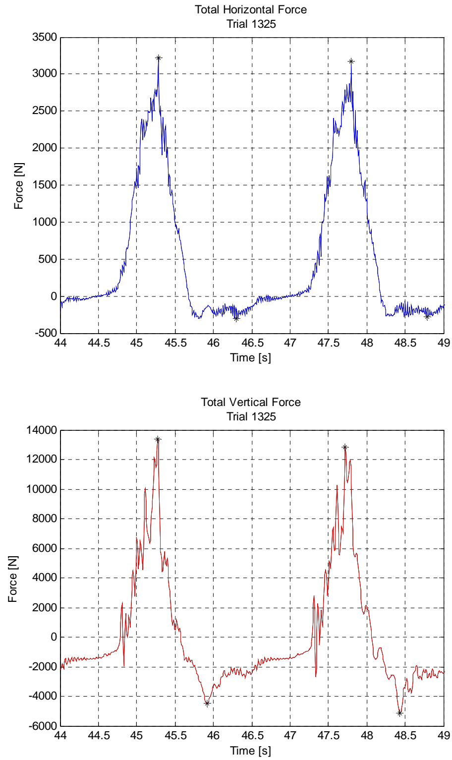
Figure 5-3. Comparison of total horizontal and vertical force events, regular wave trial 1325.
