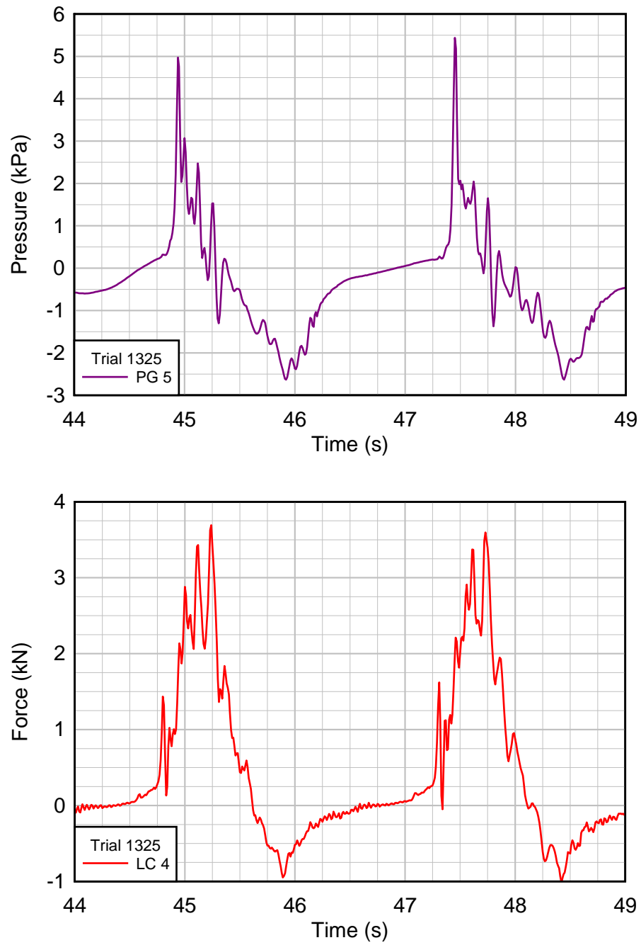
Figure 5-1. Pressure measurement taken beneath the deck and corresponding measurement of the nearest vertical load cell, regular wave trial 1325. See Figure 3-10 for instrument locations.
