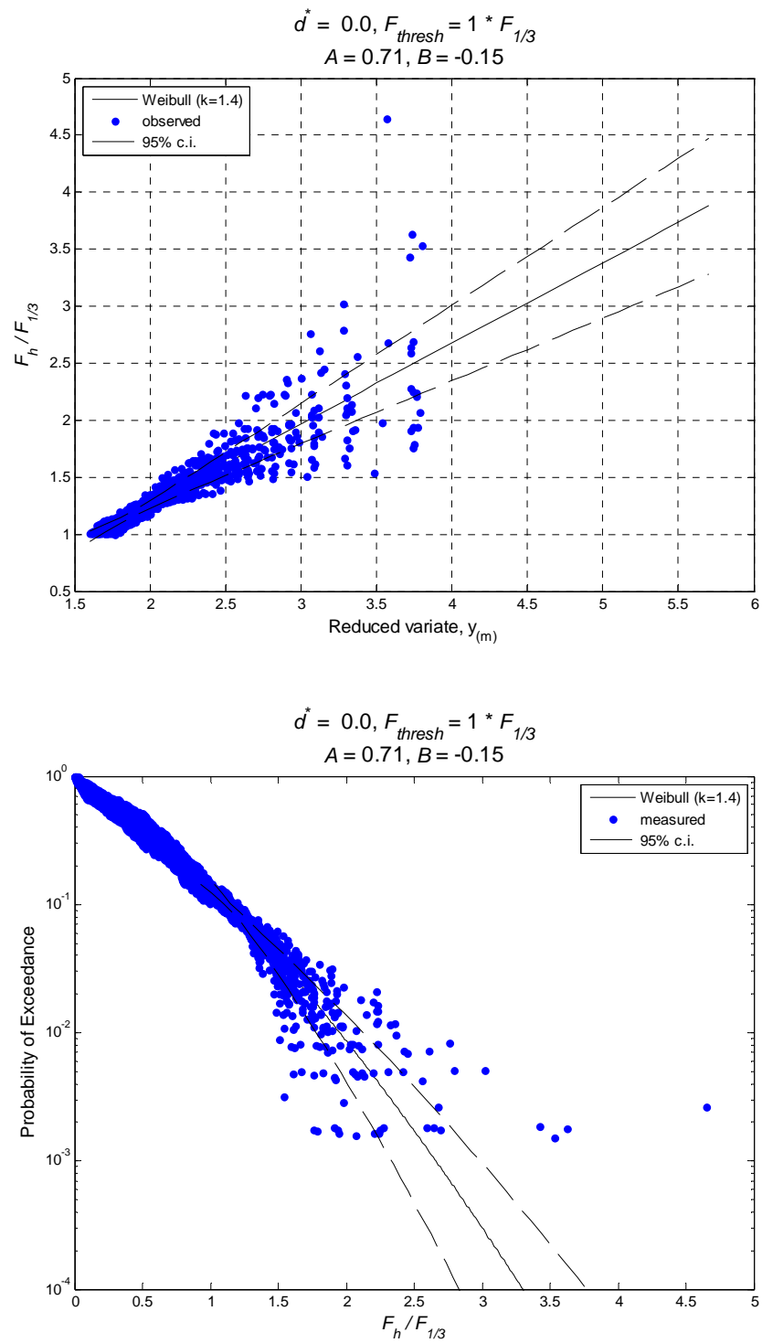
Figure H-13. Exceedance probability for normalized horizontal forces, d^* = 0.0
