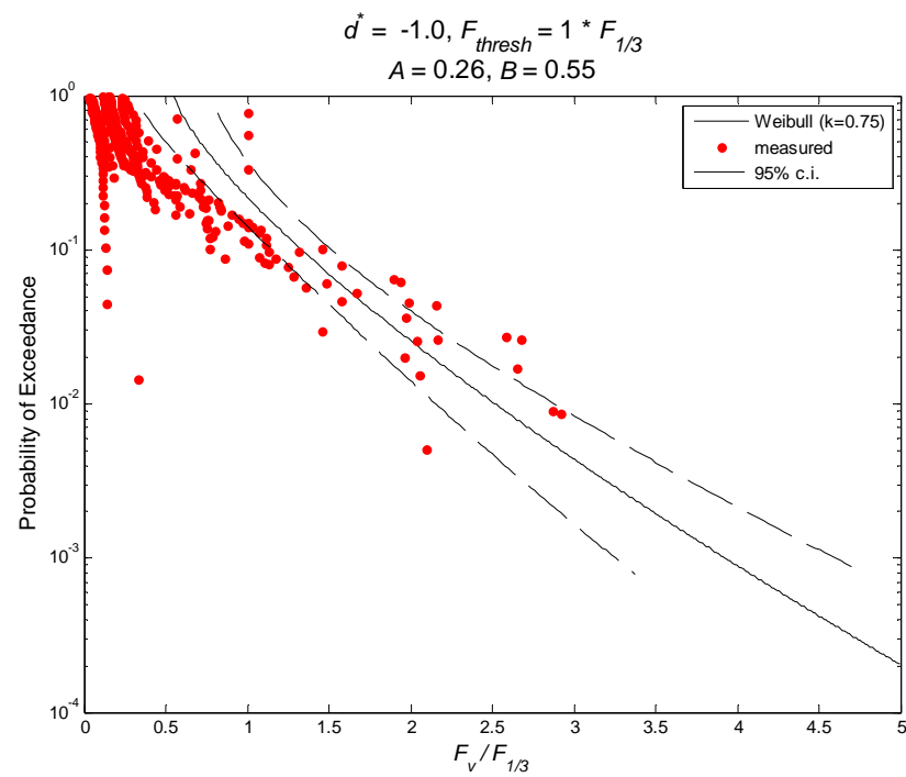
Figure H-10. Exceedance probability for normalized vertical forces, d^* = -1.0
