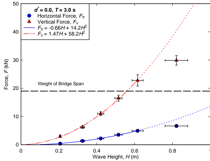
Figure 5-6. Measured forces for regular wave trials conducted at d^* = 0.0 , T = 3.0 s.
