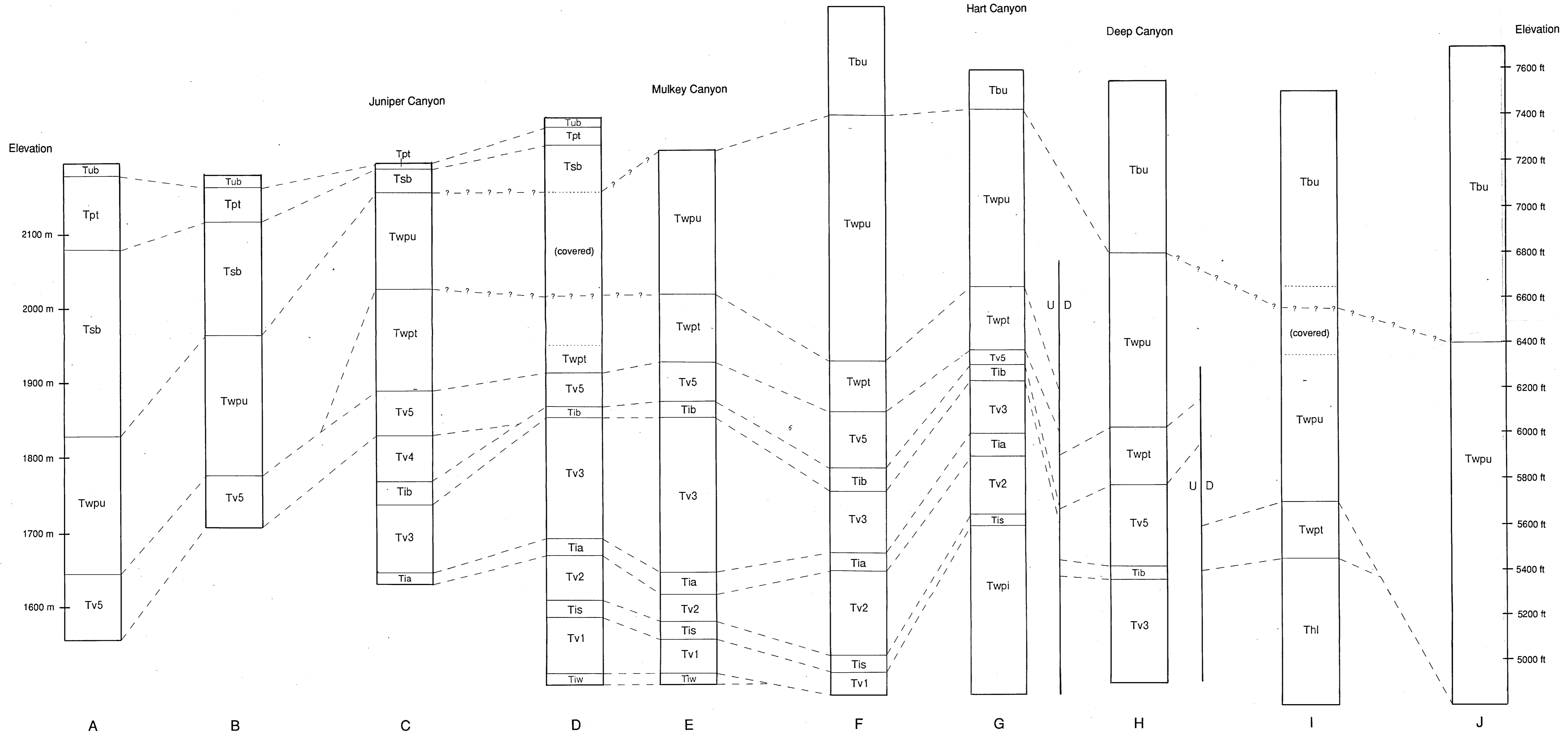
Stratigraphy of the West Side of Hart Mountain, Southern Oregon
