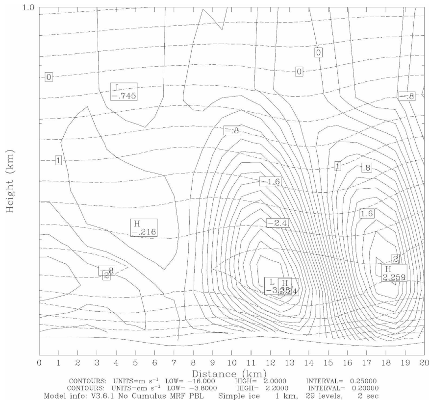
FIG. 1. North-south cross section of modeled (MM5; 1 km \times 1 km horizontal resolution) boundary layer flow over a small surface corrugation with an amplitude of about 7.5 m and a wavelength of about 8 km for a calm night in the CASES-99 experimental campaign [1200 UTC (0600 LT) 23–24 Oct 1999]. Solid lines: vertical wind speed ( \text{cm s}^{-1} ); dashed line: wind component perpendicular to the orography ( \text{m s}^{-1} ).
