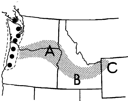
Fig. 7. Following eruption and emplacement of the Coast Range Basalts (dashed line is inferred extent, solid circles are eruptive centers), North America moved westward over the Yellowstone hot spot along the stippled path. Dike swarms which fed the Miocene Columbia River Basalts (A), basaltic volcanism in the Snake River Plain (B), and the current geothermal anomaly at Yellowstone (C) may all be manifestations of this hot spot.
