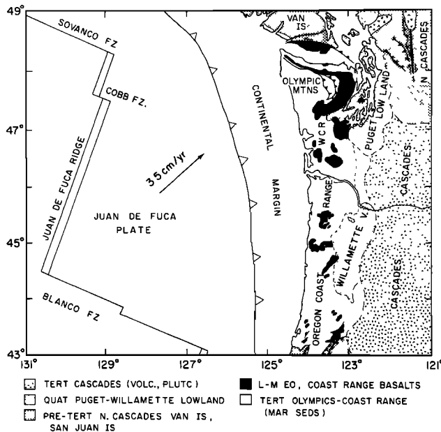
Fig. 1. Generalized geology and present plate boundaries in the Pacific Northwest. The basement rocks in the Coast Range (solid black) crop out in a north-south linear pattern from the southern tip of Vancouver Island to southern Oregon. These are tholeiitic submarine pillow lavas and subaerial alkalic basalts, which are thought to have been erupted as a line of islands at a segment of the early Tertiary Farallon-Kula plate spreading ridge.
