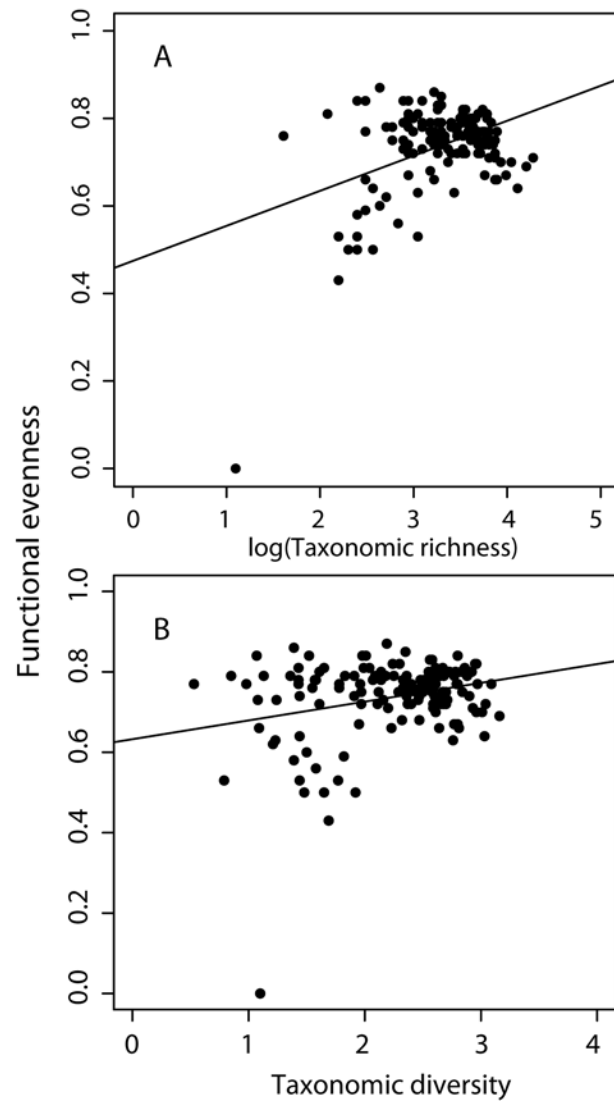
Appendix S2. Functional evenness (FEve) vs taxonomic richness ( y = 0.08\log[x] + 0.474 ) (A) and taxonomic diversity ( y = 0.05x + 0.6325 ) (B).
