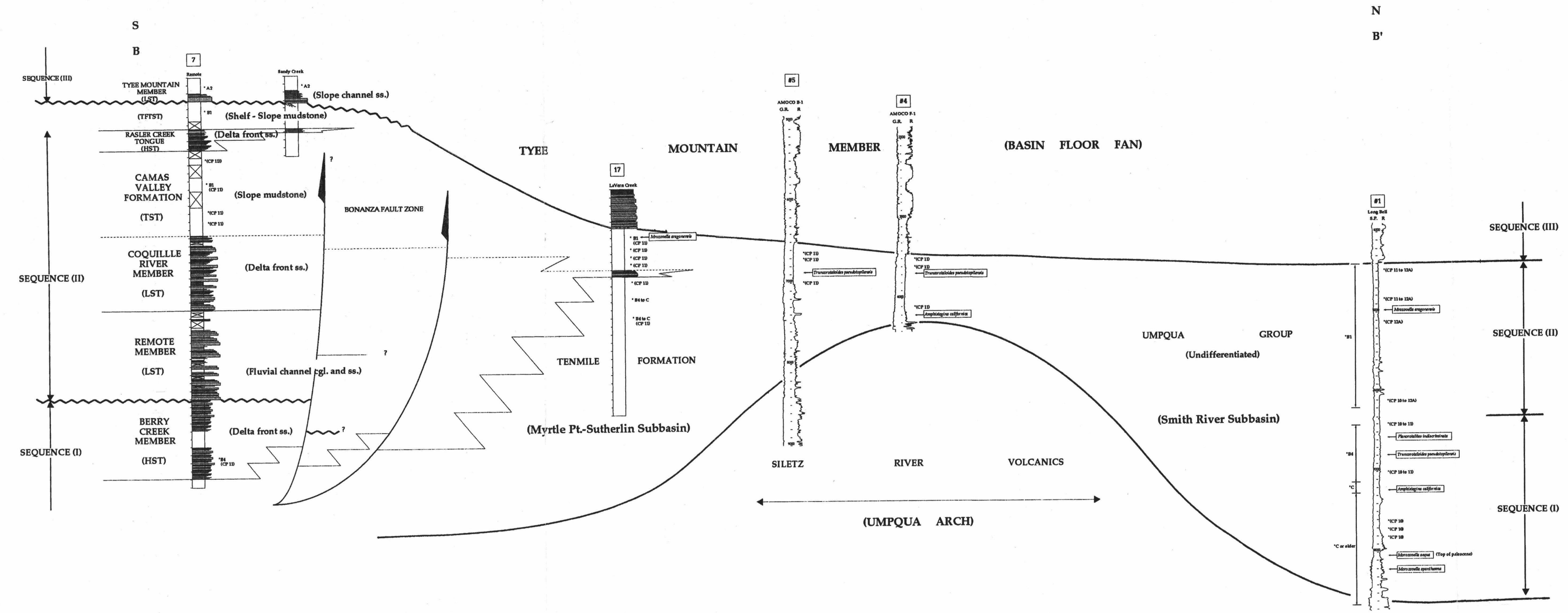
Plate 3B: Stratigraphic Cross Section: Sequence II (depositional dip-oriented)
