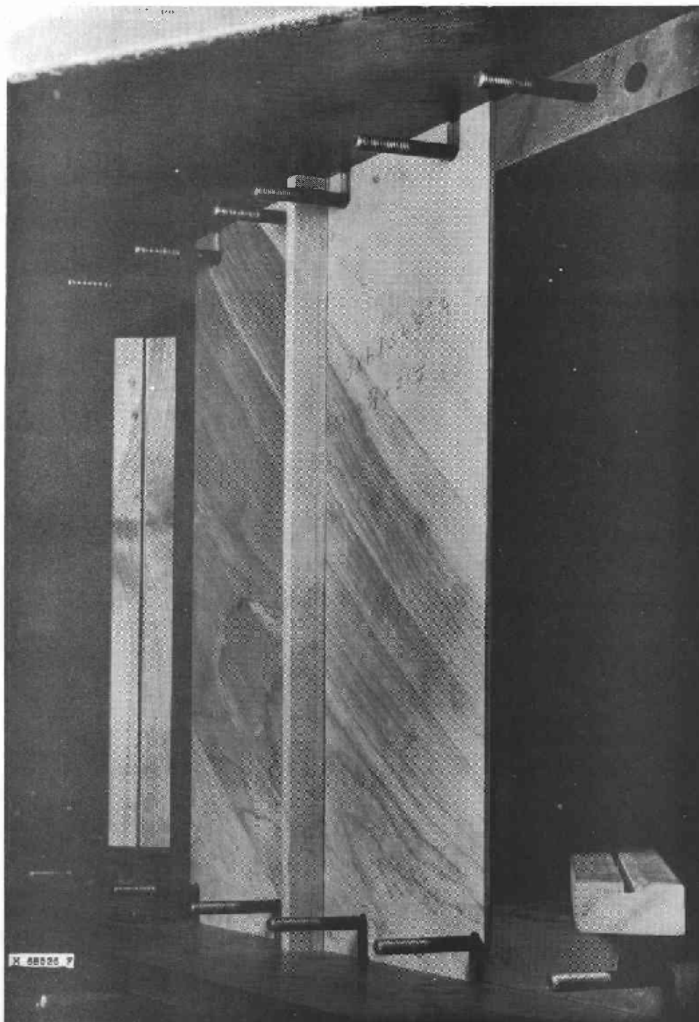
Figure 28.--Stiffened plywood plate shown fitted in test apparatus before clamping. 2 M 78962 F
