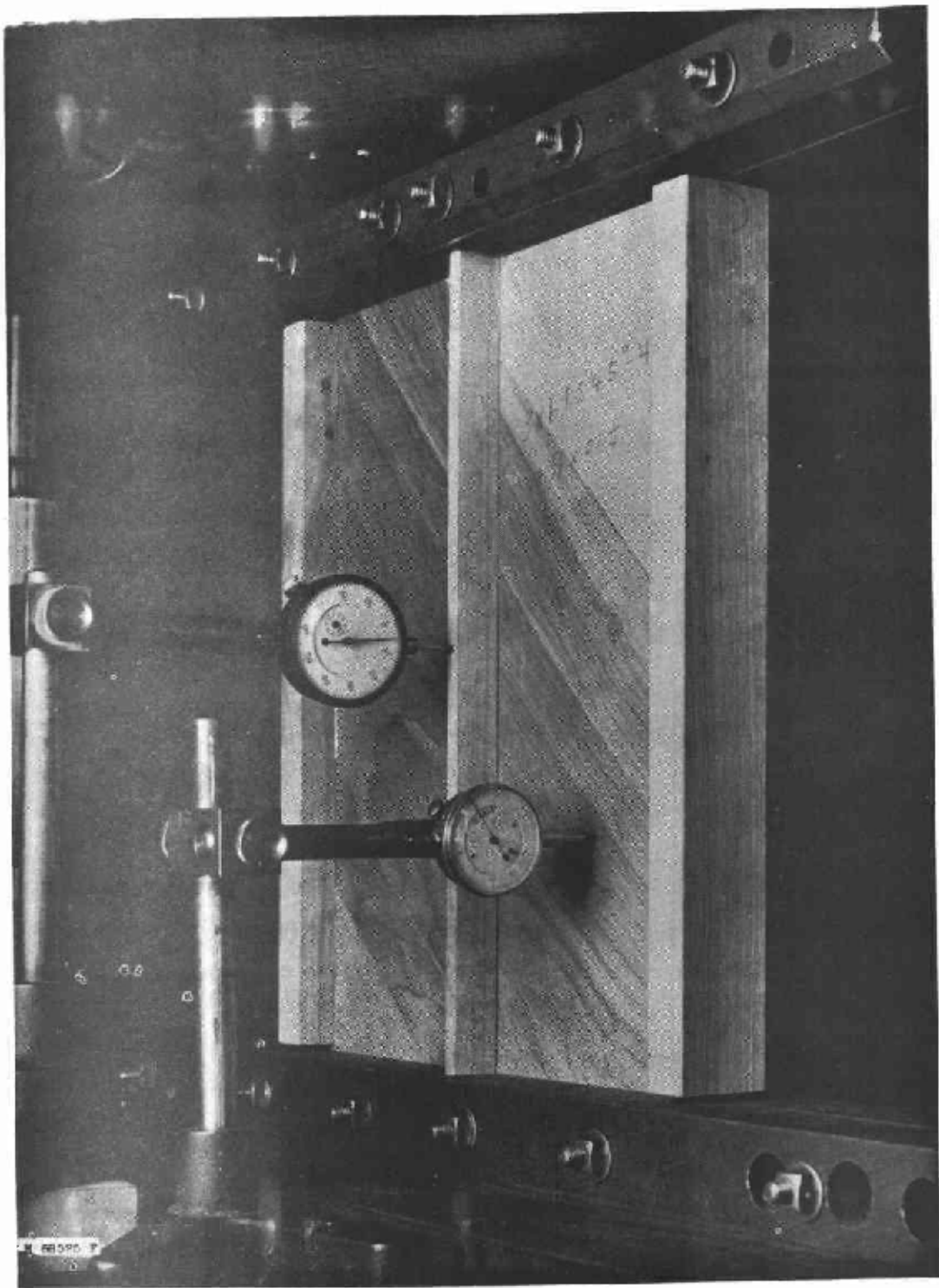
Figure 29.--Specimen ready for test. Loaded ends clamped, edges simply supported, and lateral-deflection indicating dials in position.
