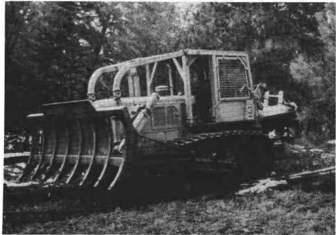
FIGURE 1. BRUSH BLADE.
