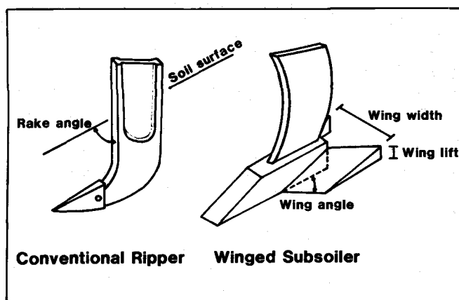
FIGURE 5. GEOMETRY OF CONVENTIONAL AND WINGED RIPPING TINES.
