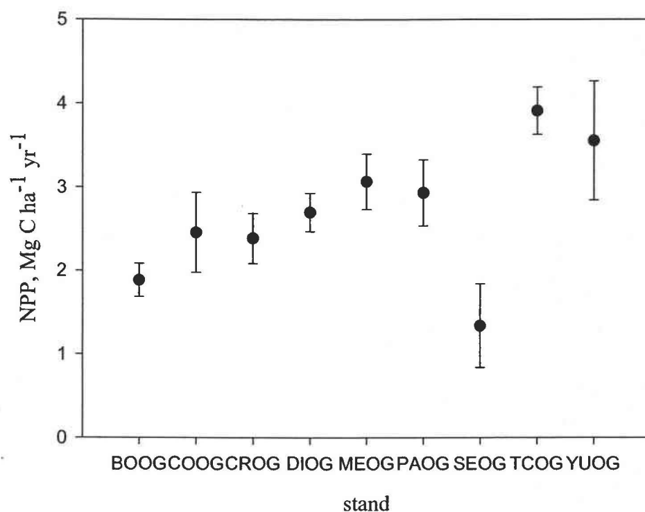
Figure 3-2: NPP b of individual 500-year old conifer forest stands on the Wind River Ranger District, Washington. Data represent differences between 1999 biomass determined by DBH and the mean of 20 Monte Carlo simulations, scaled to annual values and C content, \pm 2 SD.
