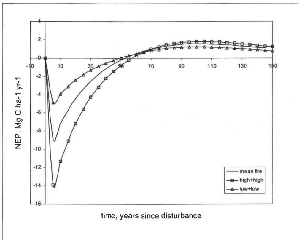
Figure 4-8: Predicted NEP_w dynamics over time (on site) during secondary succession for Scenario (4), in which all live trees in an old-growth stand are assumed killed by fire and allowed to decompose in situ . When these stores remained on site the transition from negative to positive NEP_w took approximate 50 years. As in other scenarios curves were generated by combining simple exponential decomposition models, Chapman Richards functions, and empirically derived parameters. Predicted NEP_w values are based on data from a 500 -year chronosequence of Pseudotsuga-Tsuga dominated stands at Wind River, Washington.
