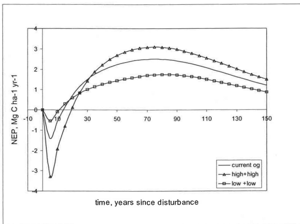
Figure 4-7: Predicted NEP_w dynamics over time (on site) during secondary succession for scenario when decomposition of old-growth CWD C stores are paired with live bole regeneration (Scenario 3). As with Scenario 2 (figure 6), the transition from negative to positive NEP_w occurred approximately 14 years after clearcutting. However, the curves, pairings of means and extremes of the ranges of live and CWD old-growth C stores, show a wider range than scenario 2, indicating CWD stores are homogenized by clearcutting. C stores removed from the site by clearcutting are not included. Predicted NEP_w values are based on data from a chronosequence of Pseudotsuga-Tsuga dominated stands at Wind River, Washington.
