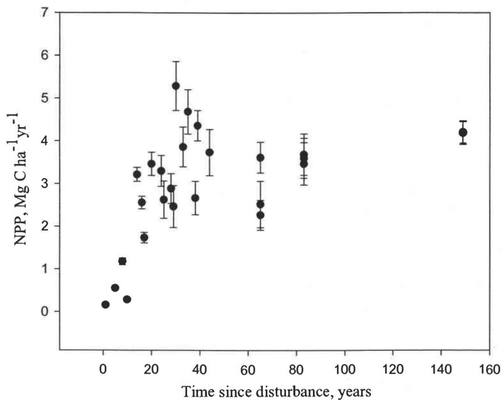
Figure 3-1: NPP_b of individual second-growth conifer forest stands on the Wind River Ranger District, Washington. Data represent differences between 1999 biomass determined by DBH and the mean of 20 Monte Carlo runs, scaled to annual values and C content, \pm 2SDs .
