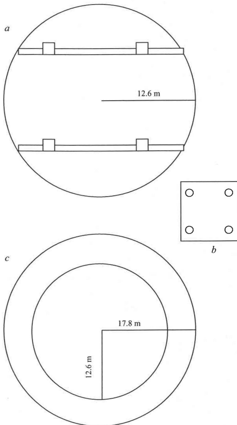
Figure 2-1: Spatial arrangement of sampling system: a) inner circle magnified to show belt transect used to inventory shrub stems and 1 m 2 quadrants used to inventory herbaceous species and fine wood debris, b) magnified 1 m 2 quadrant showing location of litter cores, c) full view of individual plot showing concentric live tree (radius=12.6 m, 0.05 ha) and CWD (radius=17.8 m, 0.1 ha) sample zones.
