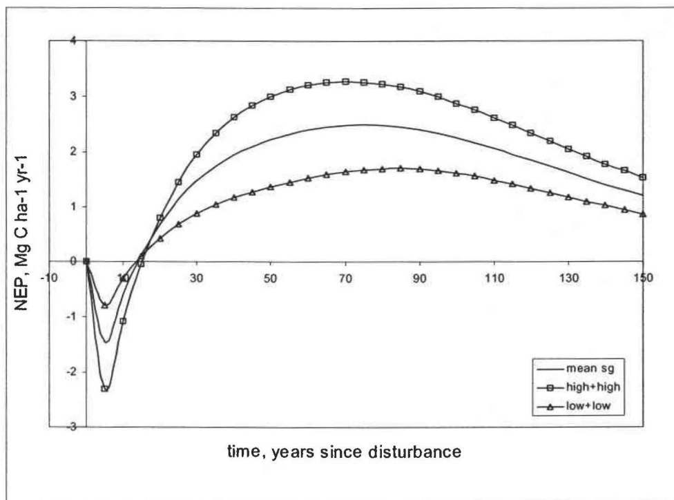
Figure 4-6: Predicted NEP_w dynamics over time (on site) during secondary succession when legacy CWD C stores were paired with live bole regeneration (Scenario 2). The solid curve describes NEP_w over succession based on mean legacy CWD C mass and mean asymptotic live bole mass. Dashed curves describe pairings of extremes of the ranges of live and CWD C stores. Totals include de novae CWD, but not stores removed from the site by clearcutting. Predicted NEP_w values are based on data from a chronosequence of Pseudotsuga-Tsuga dominated stands at Wind River, Washington.
