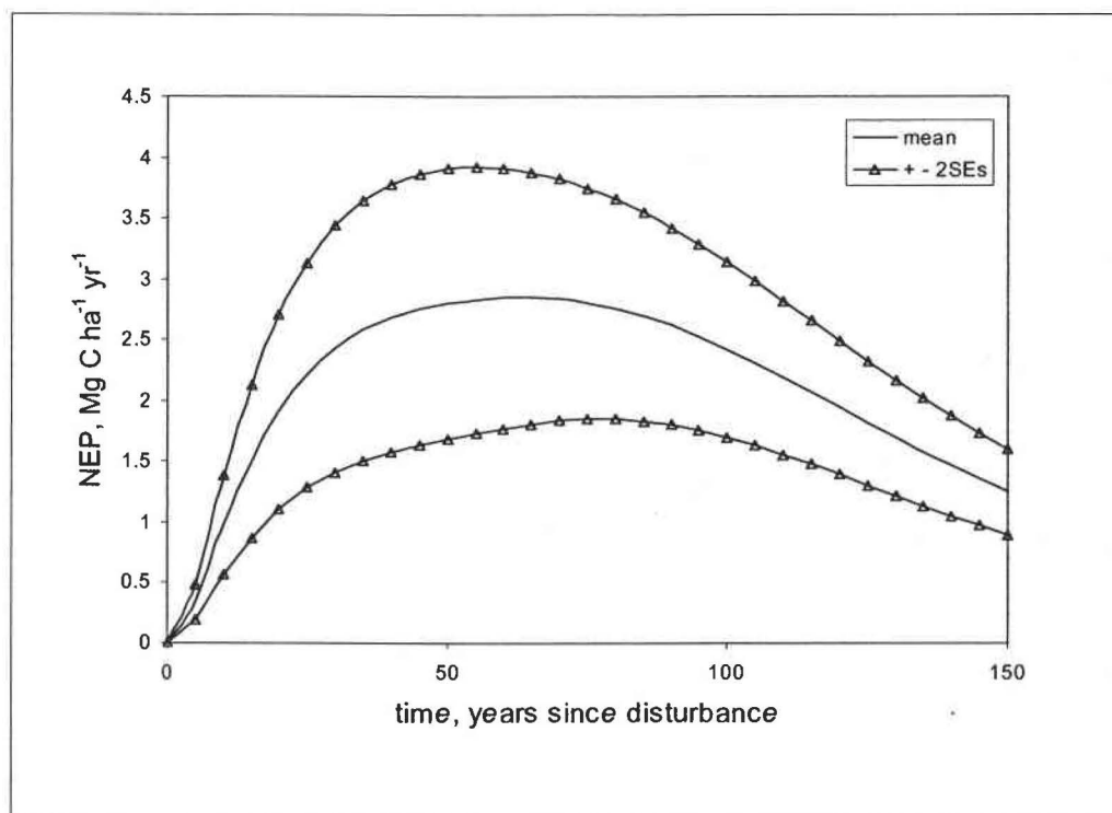
Figure. 4-5: Predicted NEP w dynamics over time (on site) during secondary succession. This scenario (1) shows live tree biomass accumulation (stand regeneration) assuming all CWD C stores are removed by logging and/or burning. Curves represent changes in NEP w based on mean growth rate derived from a Chapman-Richards function and mean asymptotic live tree mass \pm 2 SEs. Predicted NEP w values are based on data from a chronosequence of Pseudotsuga-Tsuga dominated stands at Wind River, Washington.
