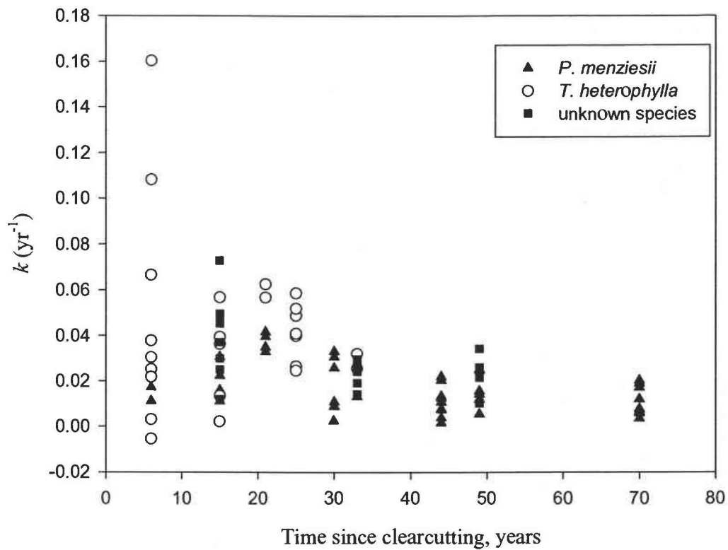
Fig 2-2: Decomposition constant ( k ) estimated for each stump and log sampled at Wind River, Washington. Estimated k calculated from Eq. 2, green wood densities for each species (USDA Wood Handbook), and empirical density estimates. Density of P. menziesii ( 0.45 \text{ Mg m}^{-3} ) was used for the unknown species.
