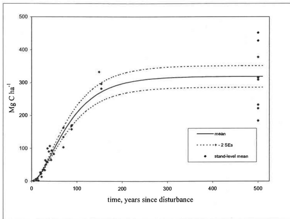
Figure 4-1: Live tree bole C stores along a 500-year chronosequence of 36 Pseudotsuga-Tsuga dominated forest stands at Wind River, Washington. The x-axis is years since disturbance, or age of the stand. The y-axis is live bole C stores in each stand. Data were fit using a Chapman Richards function where all parameters were allowed to vary.
