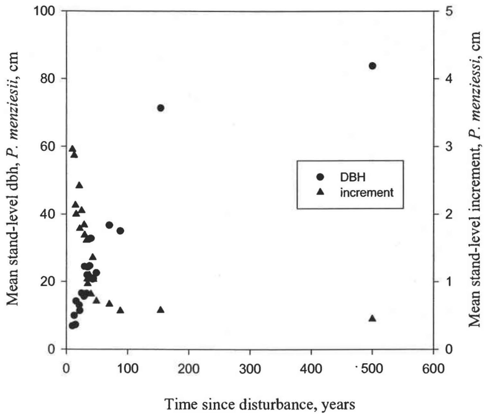
Figure 3-4: Relationship between mean DBH and mean increment (first five years before present) of P. menziesii . Data from a chronosequence of conifer dominated stands at Wind River, Washington.
