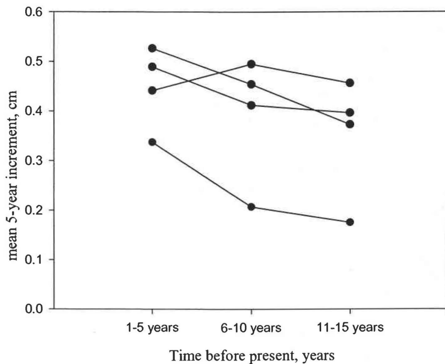
Figure 3-6: Radial increment of four old-growth stands. Points are mean 5-year radial increment widths, all species, for the 15-year period before the present. Data from a chronosequence of conifer-dominated stands at Wind River, Washington.
