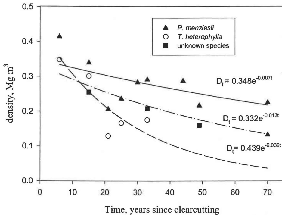
Figure 2-1: Decomposition trajectories based on non-linear regression parameter estimates shown against species mean and wood density in each stand. Data from above-ground stumps and logs along a chronosequence of conifer stands regenerating after clearcutting and fire at Wind River, Washington.
