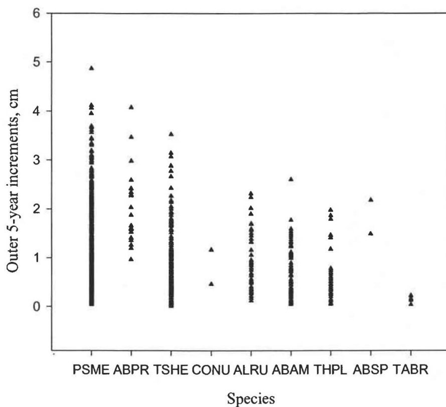
Figure 3-3: Distribution of DBH increment in the last 5 years of growth for major tree species of all stands sampled. Data from Wind River, Washington.
