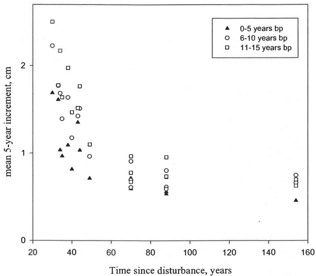
Figure 3-5: Radial increment width of second-growth stands > 30 years of age showing decline in mean increment width of individual stands over time. Each stand's current age on the X-axis is used for all of its increments for clarity. Data from a chronosequence of conifer-dominated stands at Wind River, Washington.
