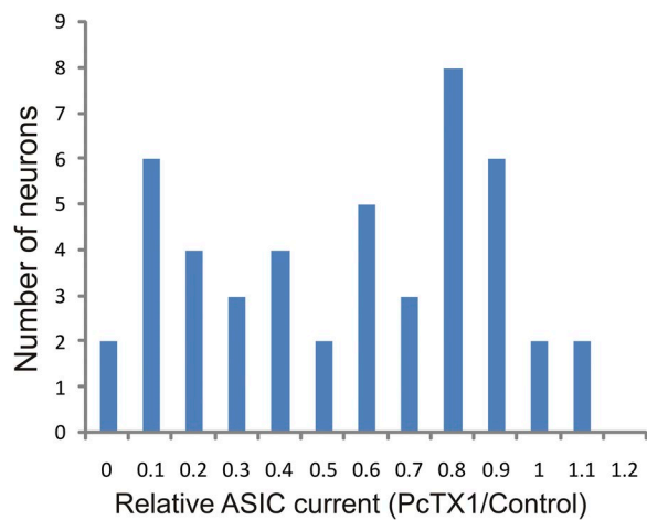
Figure S1. Histogram plot of PcTX1 inhibition of the ASIC current in cultured olfactory bulb neurons. The relative amplitude of ASIC currents in the presence of PcTX1 versus control was plotted against the number of neurons. The plot shows a trend of two major categories of responses that centered near 0.1 and 0.8.
