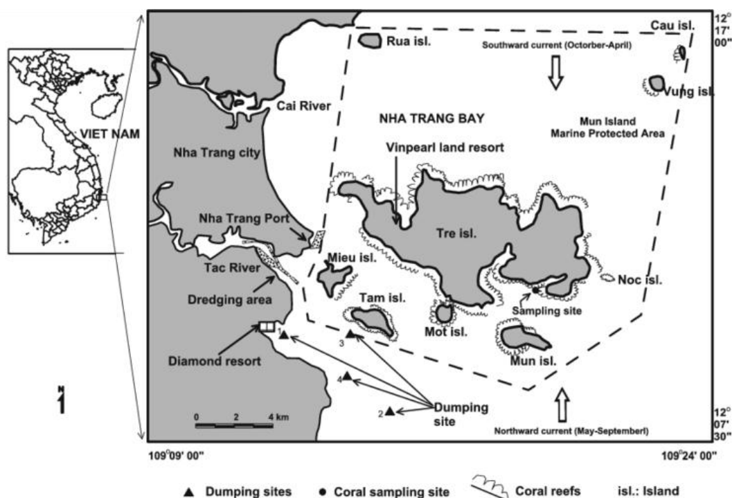
Figure 1: The map of Nha Trang Bay (adapted from Nguyen, et al., 2013)
