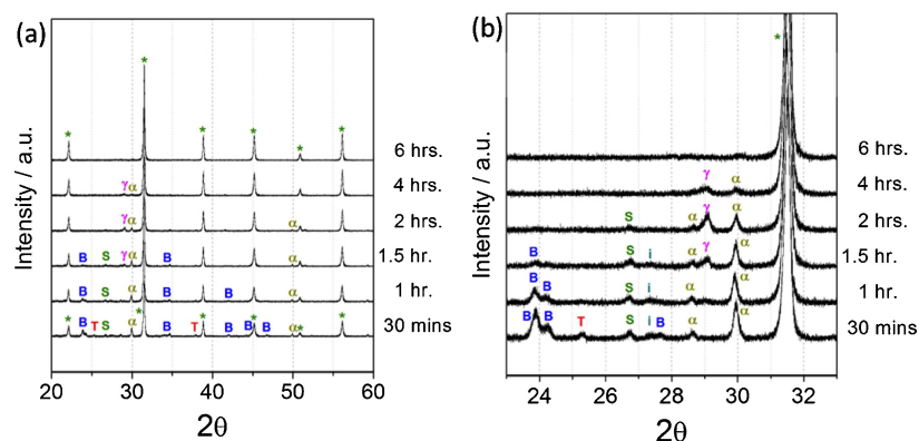
Fig. 3. X-ray diffraction patterns of 0.85BT–0.15BZT powders after calcination at 850°C for various times. B = BaCO 3 , T = TiO 2 or Ba 0.2 Bi 0.8 Ti 0.2 S, i = Bi 2 O 3 , S = potential BaCO 3 , * = perovskite phases, α = Bi 1.74 Ti 2 O 6.624 or Bi 2 O 3 (stabilized), and γ = BaBiO 3 (ss).
