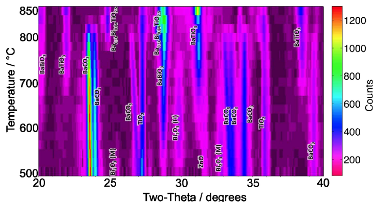
Fig. 4. Diffraction patterns from in situ measurements. Two \text{Bi}_2\text{O}_3 phases were identified: (M) room temperature monoclinic and (H) a high temperature form. Continuity of peaks also enabled the identification of the S peak from Fig. 3 as \text{BaCO}_3 .
