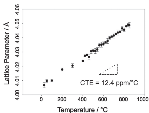
Fig. 8. Lattice parameter values of the single-phase perovskite 0.80BT-0.20BZT powder after calcination collected during re-heating and showing a constant CTE = 12.4 ppm/°C.
