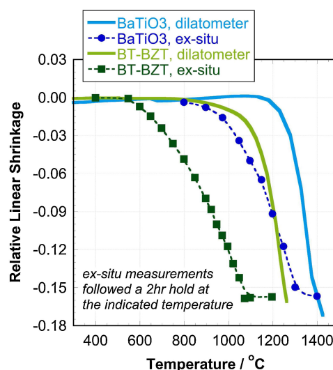
Fig. 5. Linear shrinkage of pure BT and BZT–BT measured via ex situ measurement of shrinkage after 2 h soak times at different temperatures (dotted line) and via in situ measurement of shrinkage by dilatometry (solid line).
