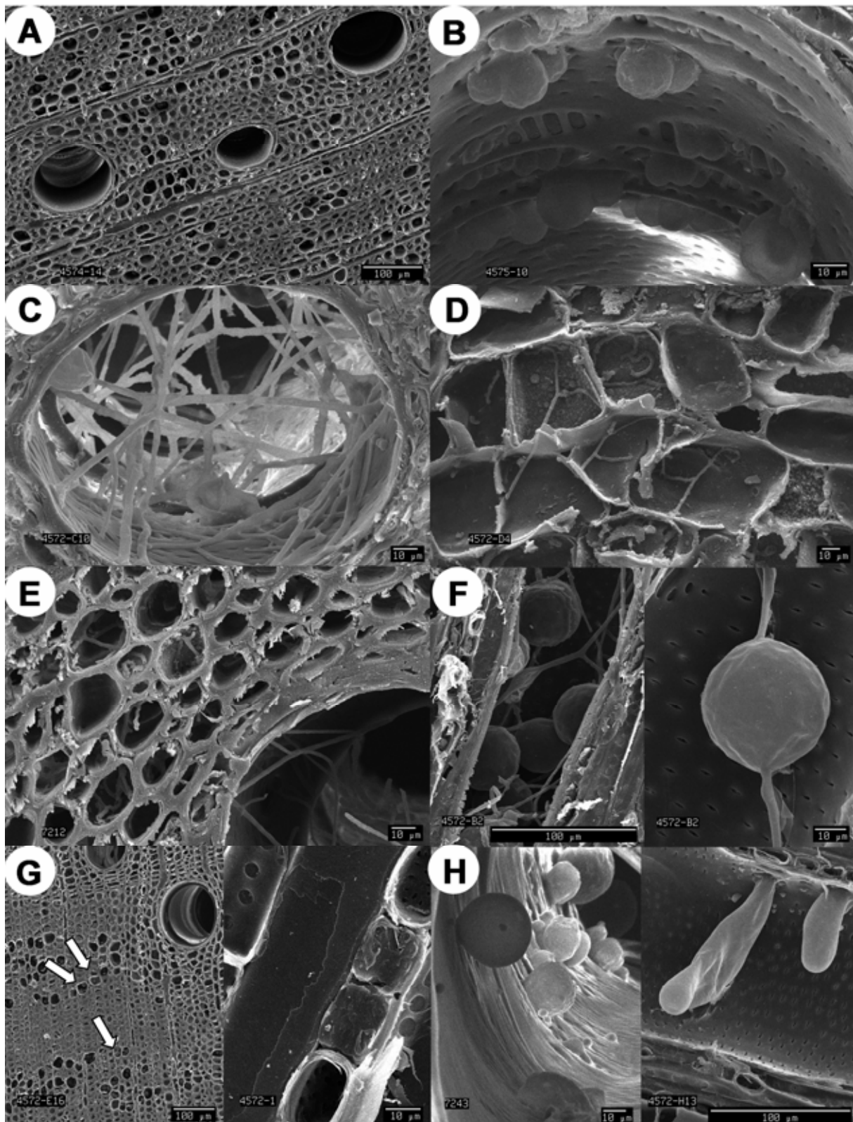
Fig. 2. Scanning electron micrographs of sapwood (A and B) not infected or (C through H) infected with Phytophthora ramorum . A, No hyphae in sapwood; B, tyloses in vessels; C, hyphae in vessels; D, hyphae in inner bark; E, hyphae in ray tracheid; F, chlamydospores in vessels; G, infected fiber cells (arrows); and H, tyloses in vessels.
