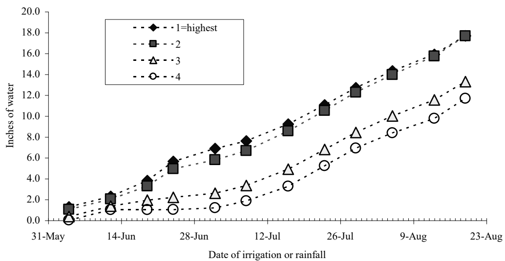
Figure 2.2. Cumulative irrigation in LSI experiment.
