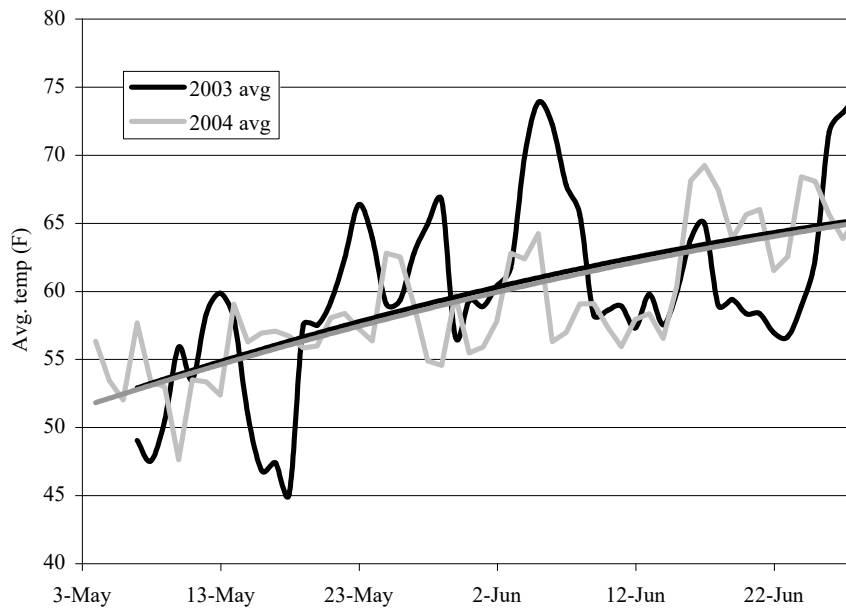
Figure 6. Average temp ((max+min)/2) and trend lines for the first 6 weeks after planting in 2003 and 2004.
