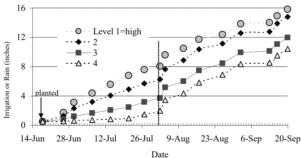
Figure 2.3. Cumulative irrigation for LSII experiment.
