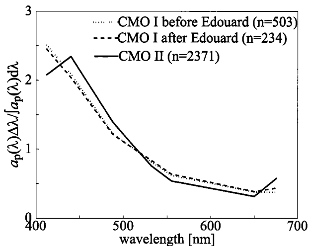
Figure 4. Medians of the area-normalized shape of particulate absorption a_p(\lambda) (the average of normalized shape is 1). The deviations from the 16th to the 86th percentile were smaller than 0.05 \text{ m}^{-1} and are not displayed. Numbers in parentheses denote the number of spectra used for the analysis.
