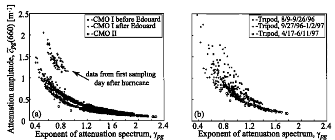
Figure 5. Parameters of the least squares fit model to the beam attenuation spectra c_{pg}(\lambda) = \bar{c}_{pg}(660)(\lambda/660)^{-\gamma_{pg}} for all the data from the BBL at the time series station (a) for both CMO cruises and (b) from the tripod data at 2 m above bottom.
