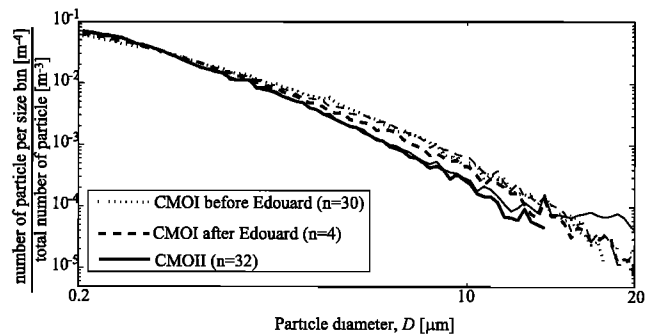
Figure 6. Mean (thin line) and median (thick line) of the area-normalized particle size distribution shape of all data of each sampling period. When no values are present, zero particles median or mean were recorded.
