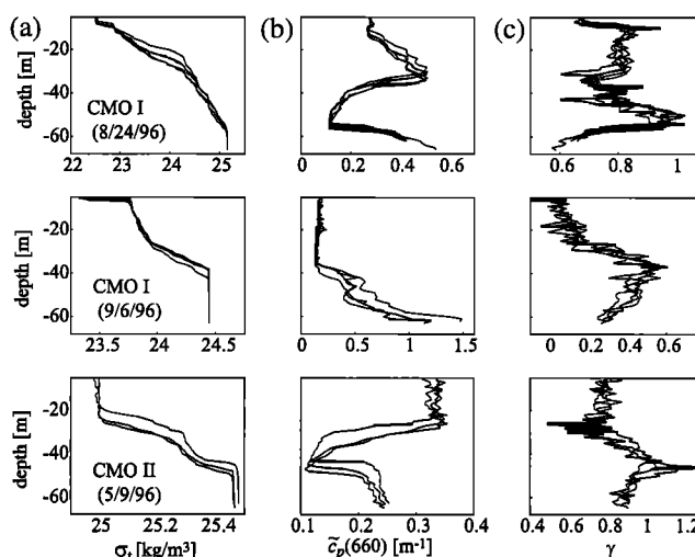
Figure 2. (a) Representative depth profiles of density \sigma_t , (b) the magnitude ( \tilde{c}_p(660) ), and (c) the exponent of a hyperbolic fit ( \gamma ) to the particulate attenuation. Data from consecutive profiles (typically within 40 min) in the fall during CMO I prior to Hurricane Edouard (August 24, 1996), during CMO I following the hurricane (September 6, 1996), and in the spring during CMO II (May 9, 1997). BBL is typically only the bottom 10–20 m of each profile. Note the different scales.
