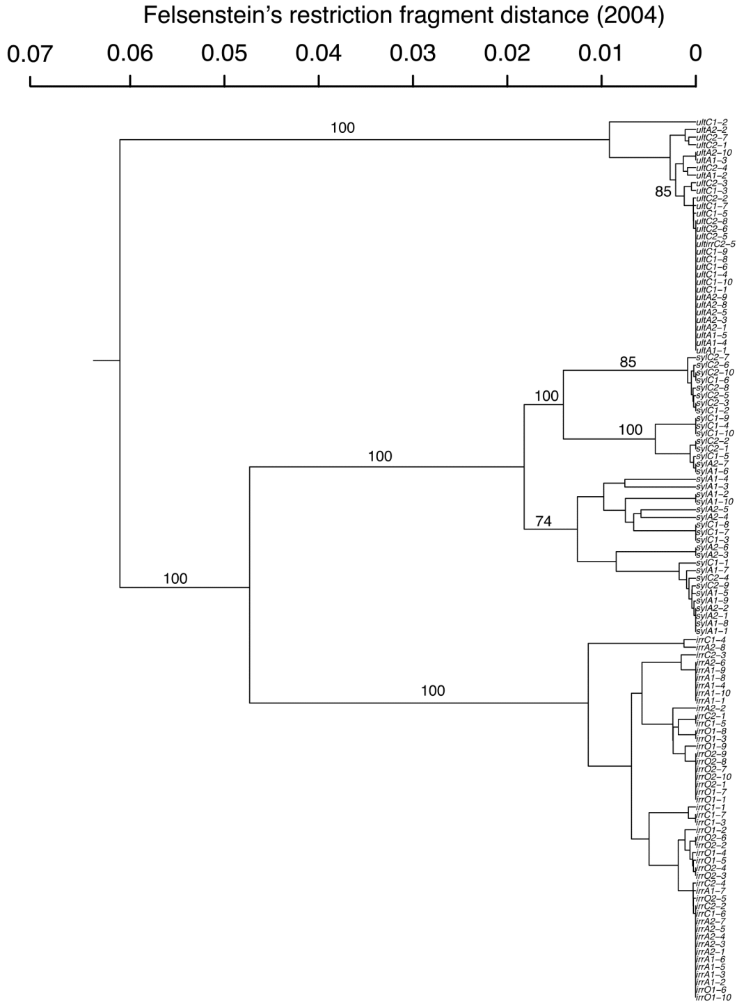
eXtra Fig. 1. UPGMA tree of P. irregulare , P. sylvaticum , and P. ultimum based on Felsenstein's restriction fragment distance of the primer AC-A. Branches with >70% bootstrap support are labeled.
