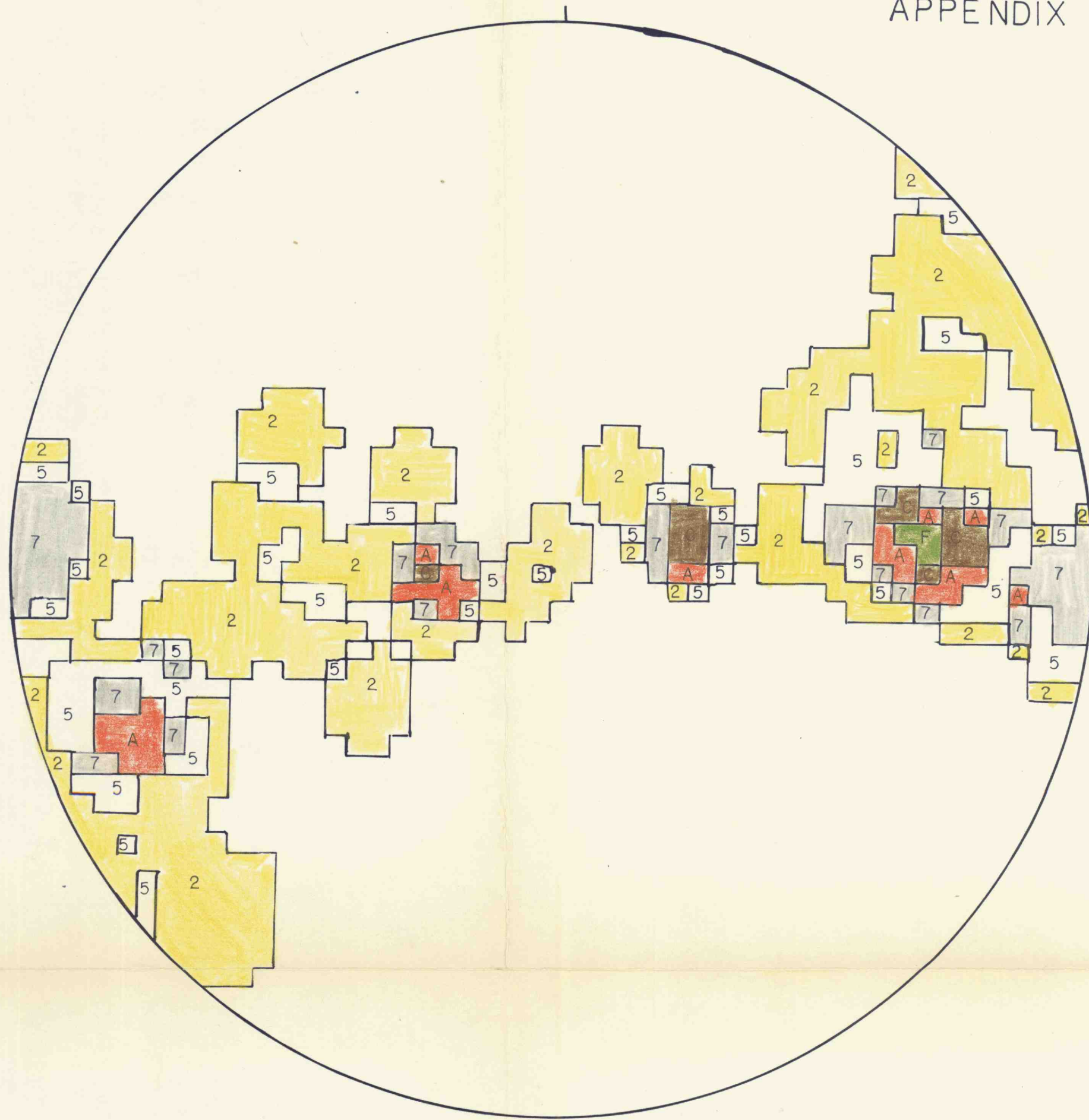
A) STERONEPLOT OF POLES TO S_1 IN SECTIONS 34, 35, 36 IN THE NORTHWEST AND NORTHCENTRAL PARTS OF THESIS AREA
