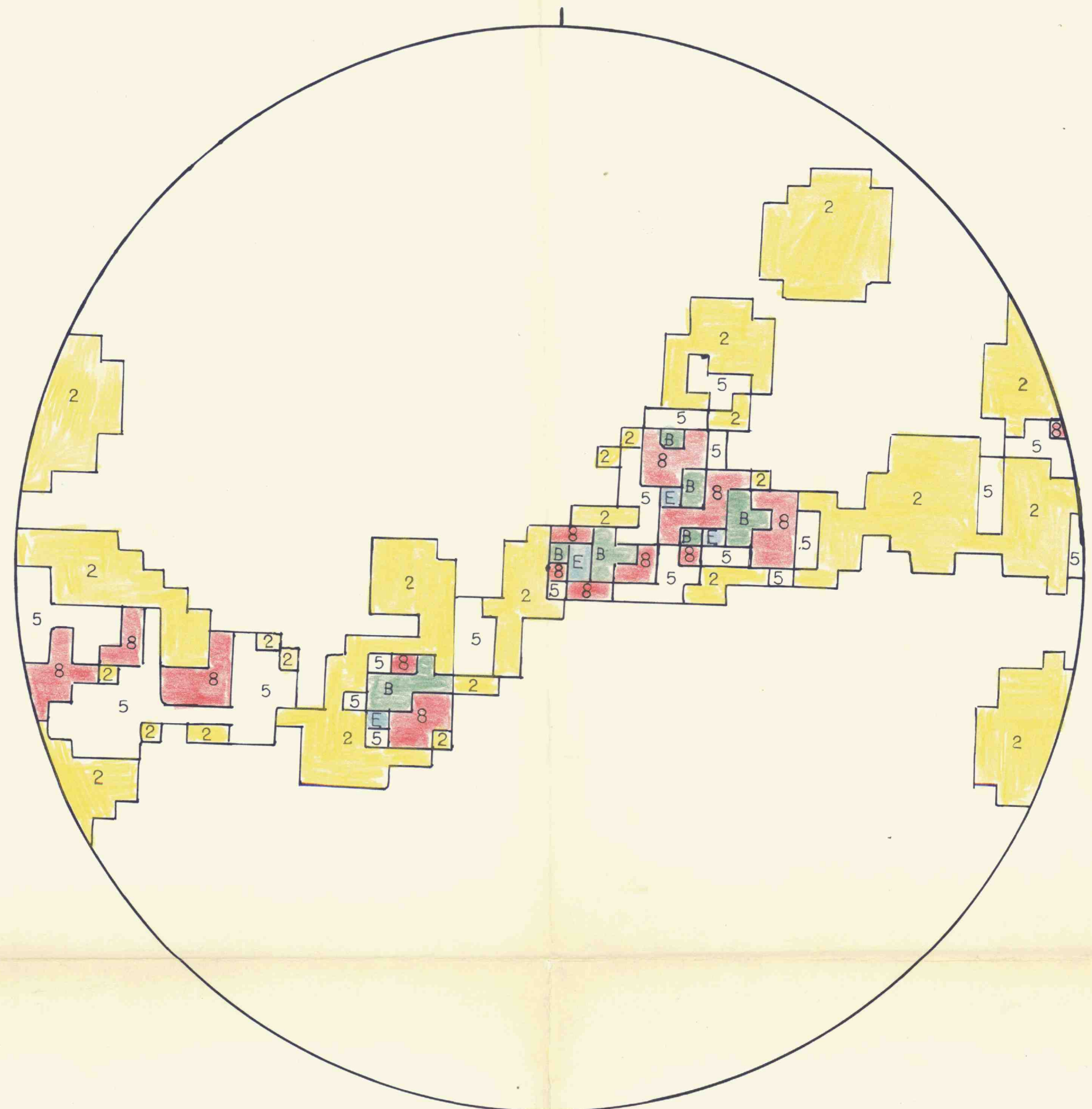
B) STERONEPLOT OF POLES TO S_1 IN THE SOUTHCENTRAL AND SOUTHWEST PARTS OF THESIS AREA
