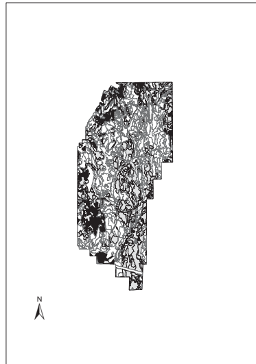
Figure 4. Current (1989) volume per ha as low (white, up to 400 m 3 /ha), medium (grey, up to 800 m 3 /ha), or high (black, greater than 800 m 3 /ha) classes for i) aerial data and model only; ii) aerial data and model, localized using the ground data; and iii) aerial data and model, based on aggregated stands.
