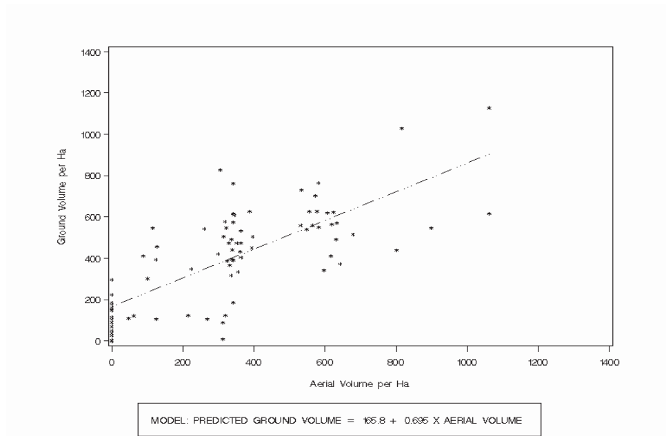
Figure 3. Scatterplot of current ground measured volume versus model-estimated aerial volume using the 83 grid points.
