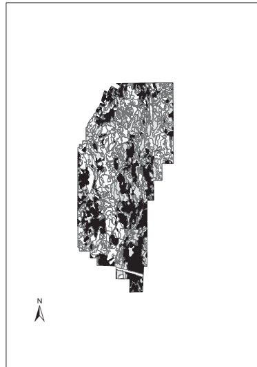
Figure 5. Projected (2019) volume per ha as low (white, up to 400 m 3 /ha), medium (grey, up to 800 m 3 /ha), or high (black, greater than 800 m 3 /ha) classes for i) aerial data and model only; ii) aerial data and model, localized using the ground data; and iii) aerial data and model, based on aggregated stands.
