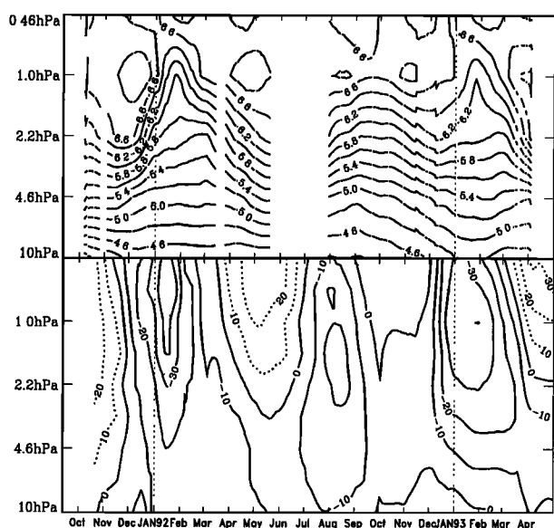
Figure 3. Time- \log_{10}[P/hPa] cross-section of equatorial MLS H_2O (upper panel, 0.2 ppmv contours) and United Kingdom Meteorological Office (UKMO) zonal-mean equatorial winds (lower panel, 5 ms^{-1} contours). Dotted vertical lines show January 1 for 1992 and 1993.
