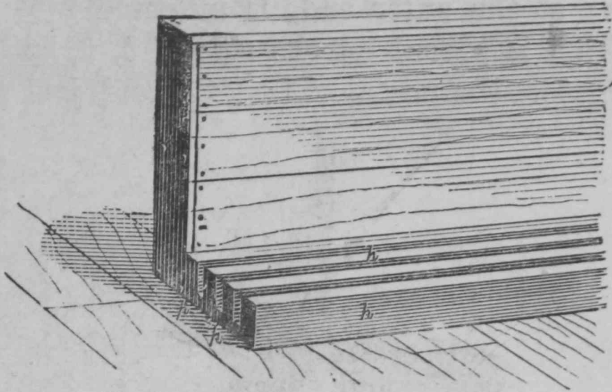
Fig. 172.—A SLATTED STABLE FLOOR.
