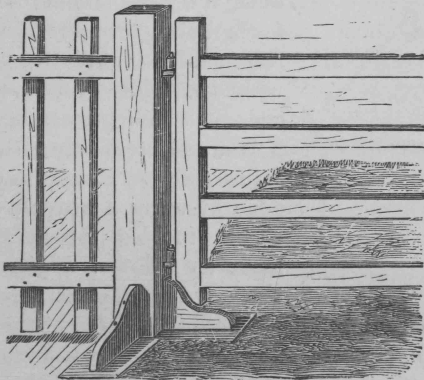
Fig. 88.—BRACING A GATE POST.
