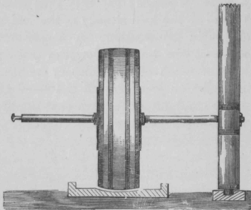
Fig. 132.—HOME-MADE BONE-MILL.
