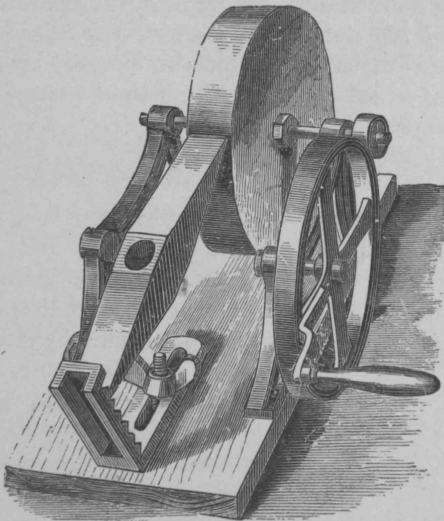
Fig. 16.—DEVICE FOR GRINDING MILL-PICKS.
