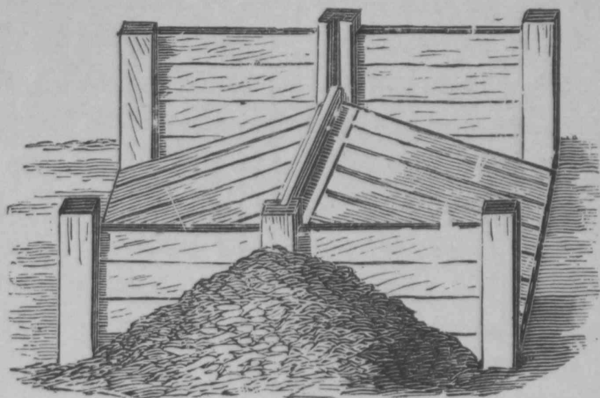
Fig. 123.—WASTE-GATE FOR POND.
