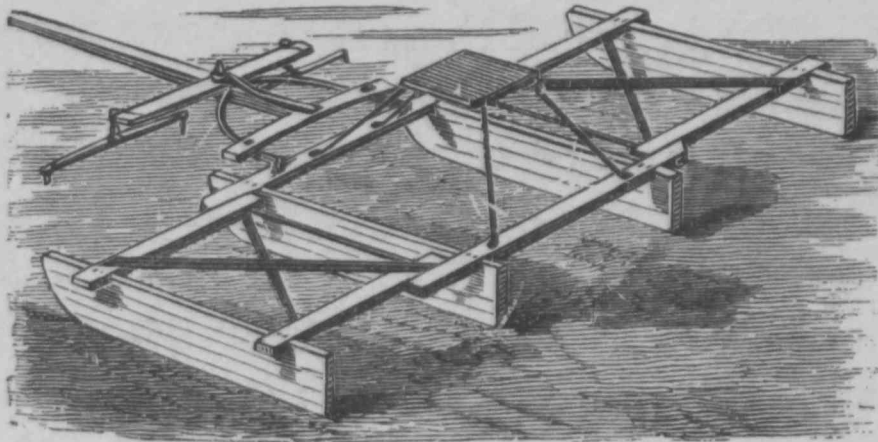
Fig. 38.—FLEXIBLE CORN-MARKER.
