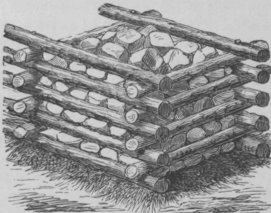
Fig. 193.—A CRIB FOR A DAM.
