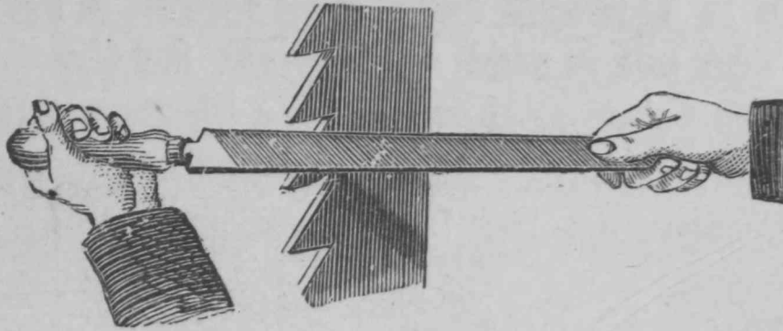
Fig. 102.—TO REST THE HAND IN FILING.
