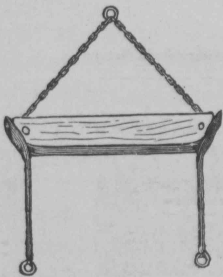
Fig. 89.—WHIPPLE-TREE.
