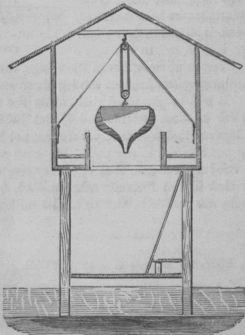
Fig. 119.—SECTION OF BOAT-HOUSE.
