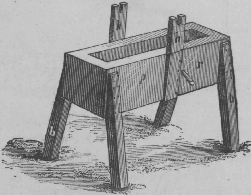
Fig. 175.—A BOX FOR A GRINDSTONE.
