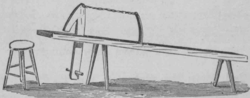
Fig. 28.—SHAVING-HORSE FOR SHINGLES.
