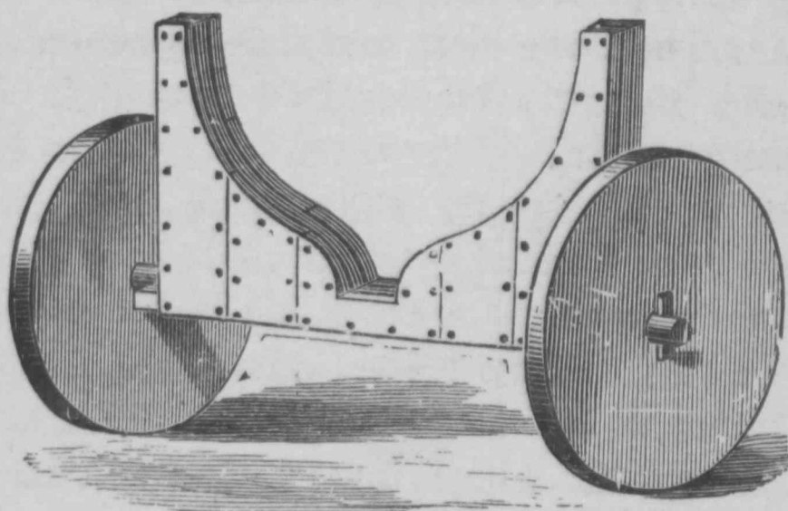
Fig. 47.—CRADLE FOR A BOAT.
