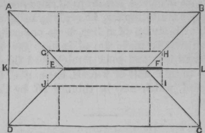
Fig. 73.—PLAN FOR RECTANGULAR FIELD.
