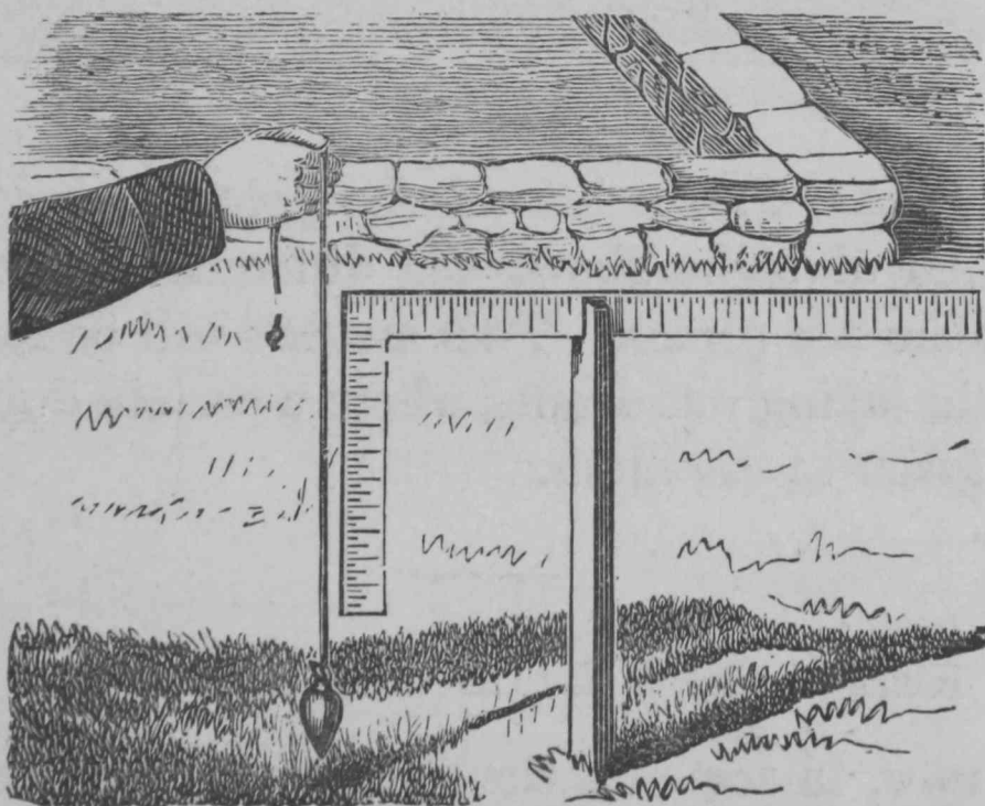
Fig. 24.—MANNER OF LEVELLING A WALL.
