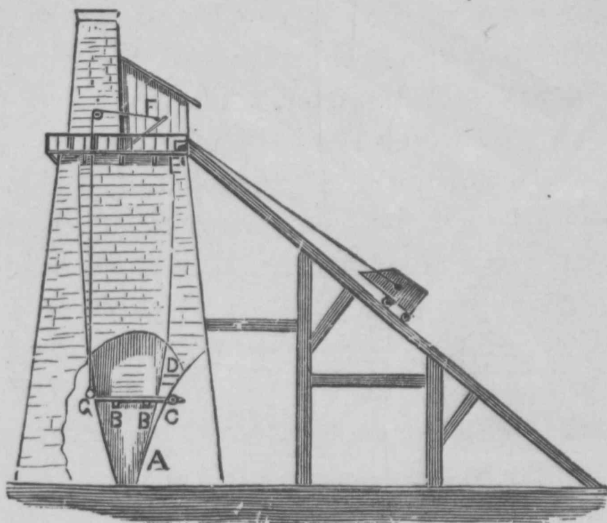
Fig. 65.—IMPROVED LIME KILN WITH ELEVATED TRACK.
