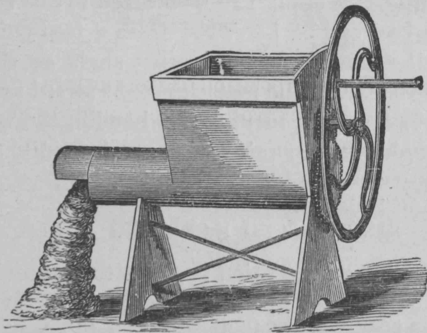
Fig. 57.—MACHINE FOR MIXING CEMENT.
