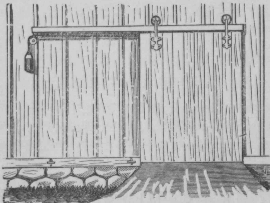
Fig. 34.—SELF-CLOSING SLIDING DOOR.
