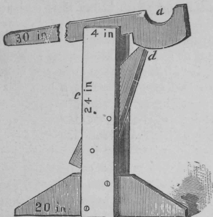
Fig. 124.—MICHIGAN WAGON JACK.
