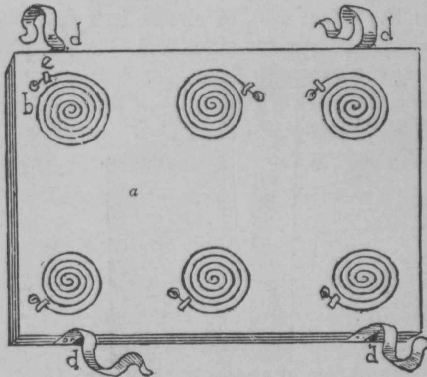
Fig. 164.—BOTTOM-BOARD OF SPRING-BOX.
