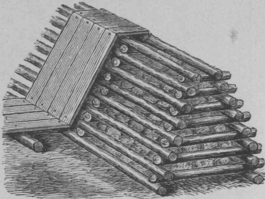
Fig. 194.—LOG FRAME FOR A DAM.
