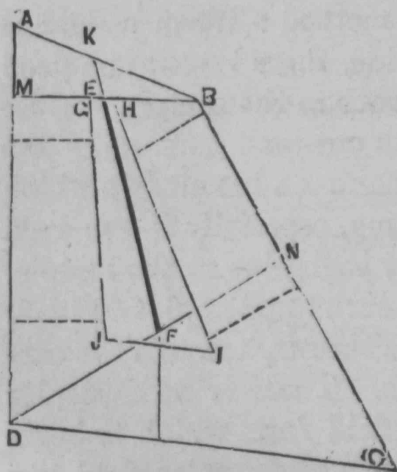
Fig. 74.—PLAN FOR IRREGULAR FIELD.
