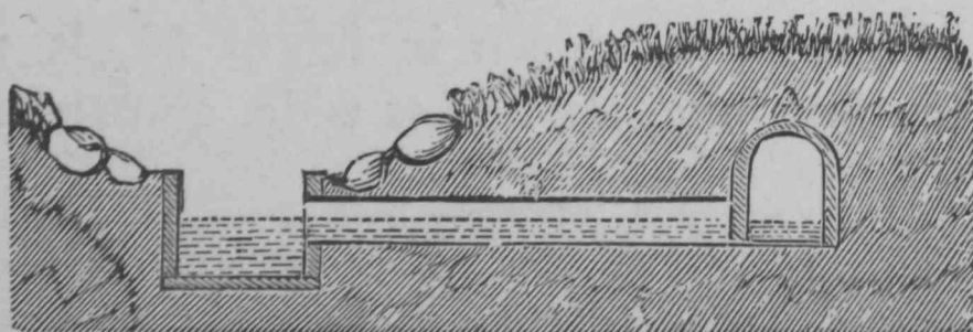
Fig. 26.—TAKING WATER FROM UNDERDRAIN.
