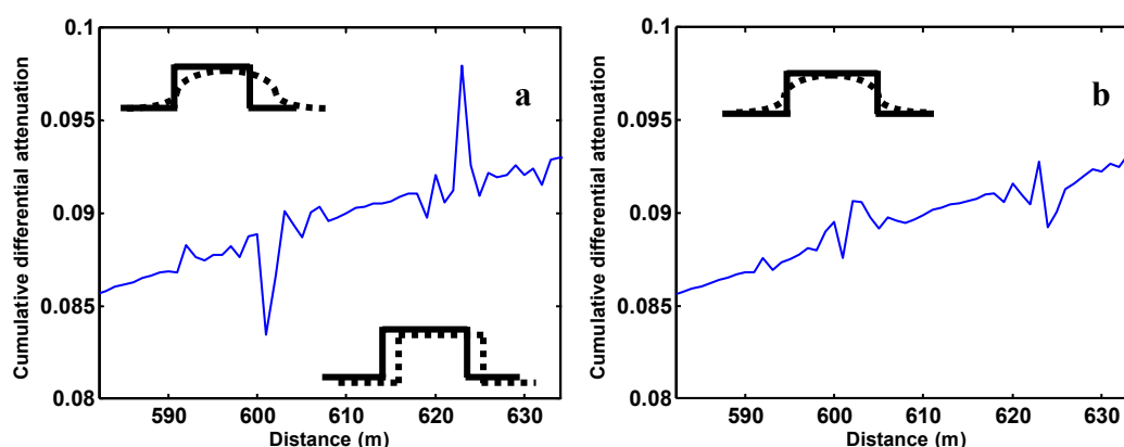
Figure 5. The schematic drawings show the nearby forward anti-Stokes (continuous line) and the shifted and more dispersed far reverse anti-Stokes (dotted line) responses. (a) Overshoot due to misalignment; (b) Overshoot due to dispersion.
