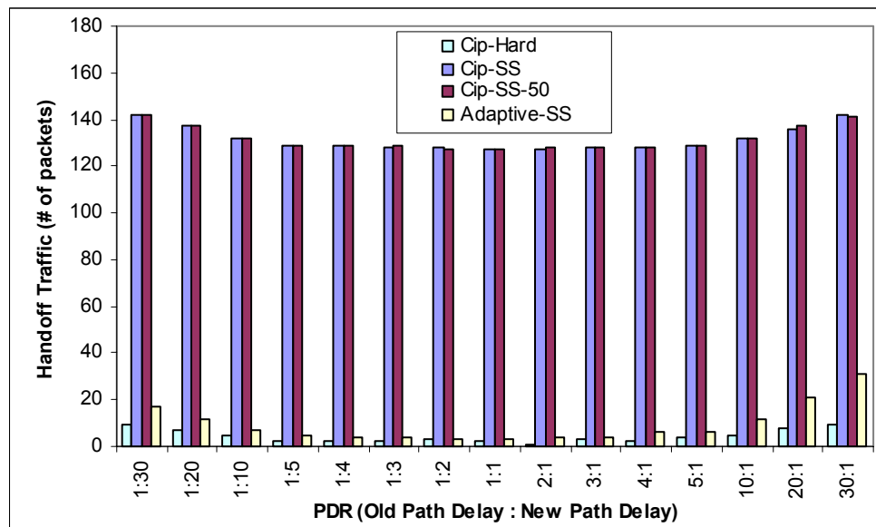
FIGURE 7: Handoff Traffic for Various PDRs
