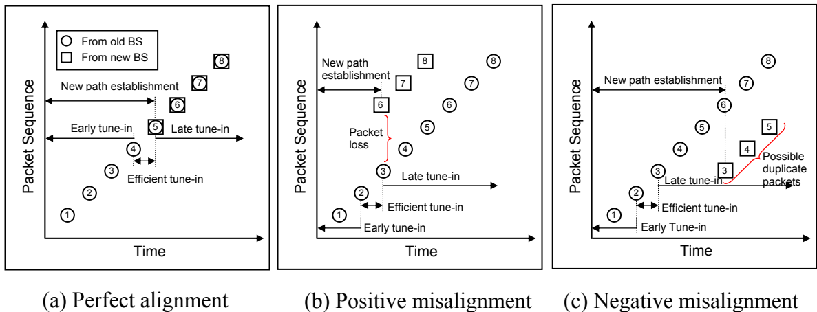
FIGURE 2: Stream Alignment and Tune-in Issues
