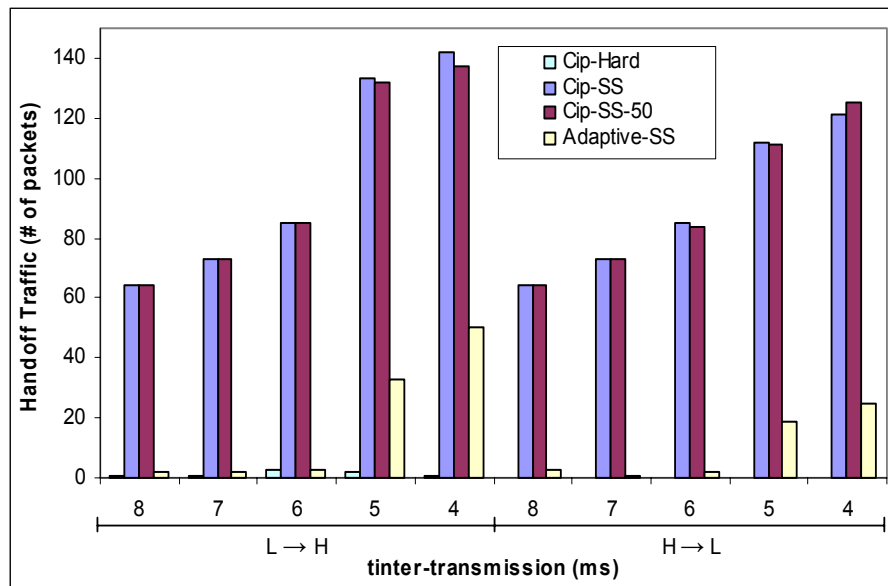
FIGURE 10: Handoff Traffic for Various Cell Densities.
