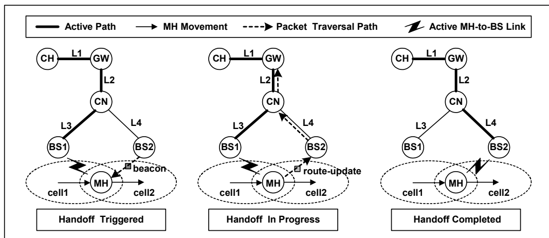
FIGURE 1: A Simple Handoff Scenario
