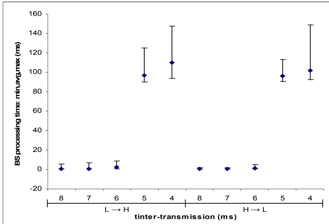
FIGURE 9: BS Processing Times of the High-density Cell for Adaptive-SS.
