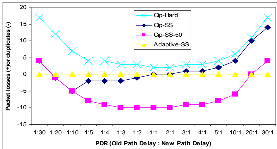
FIGURE 6: Handoff Performance for Various PDRs.
