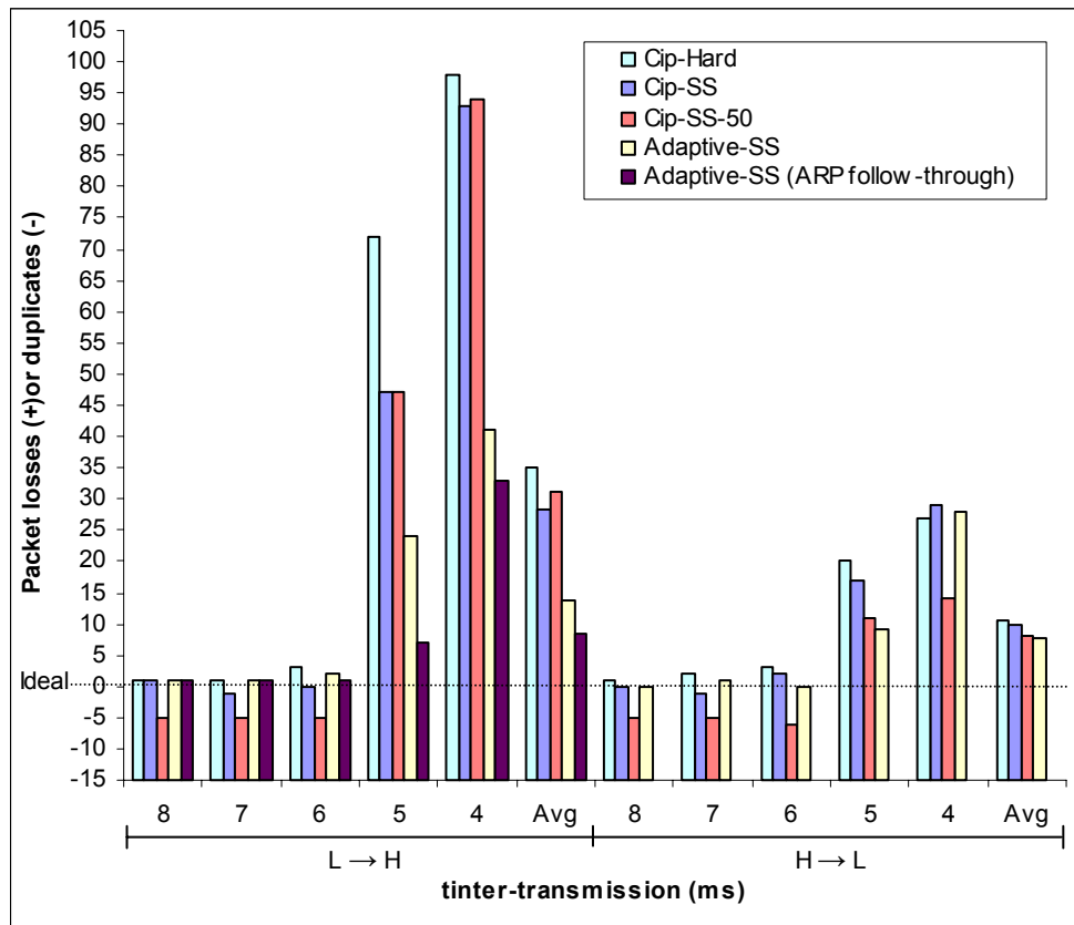
FIGURE 8: Handoff Performance for Various Cell Densities
