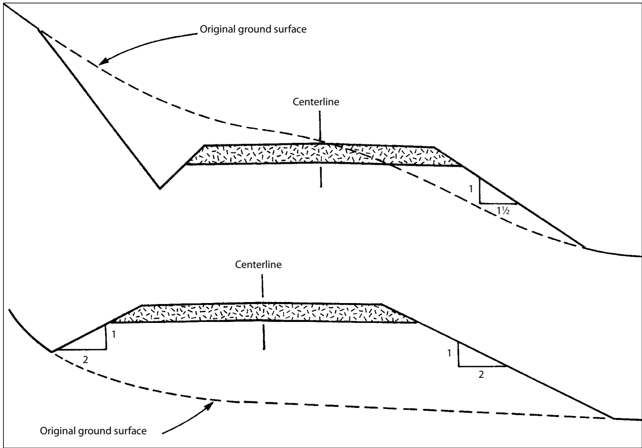
Figure 15. Partial fills at 1 1/2:1 (top) and 2:1 (bottom) fill slopes
