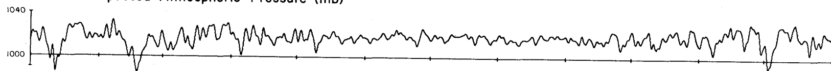
Low-passed Atmospheric Pressure (mb)
