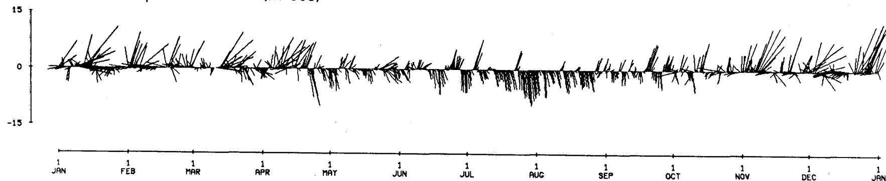
Low-passed Wind (m/sec)
