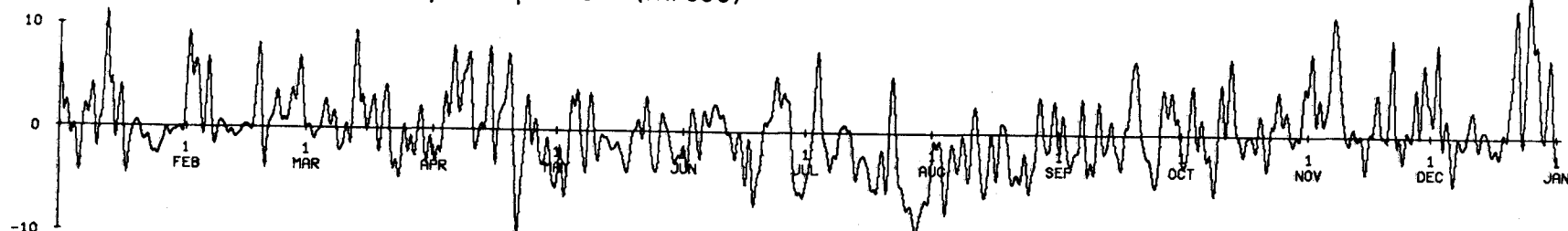
Northward wind, low-passed (m/sec)
