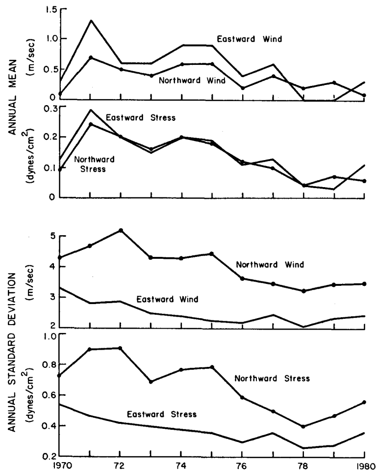
Figure 7. Annual means and standard deviations of low-passed sea level, atmospheric pressure, adjusted sea level, wind and wind stress.
