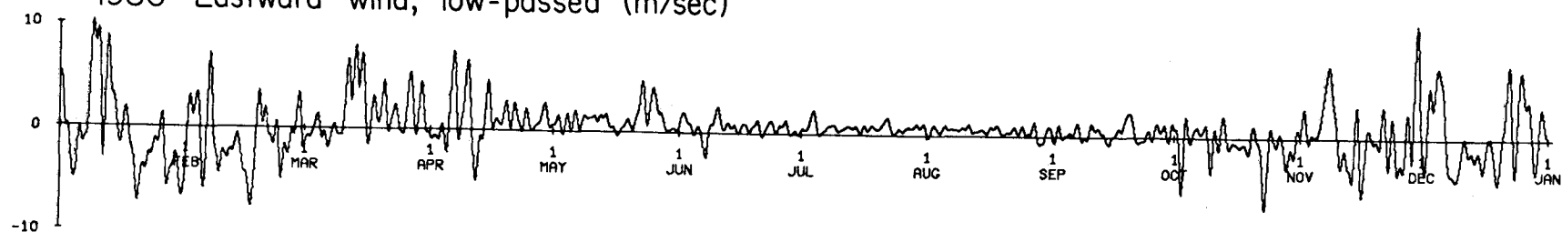
1980 Eastward wind, low-passed (m/sec)
