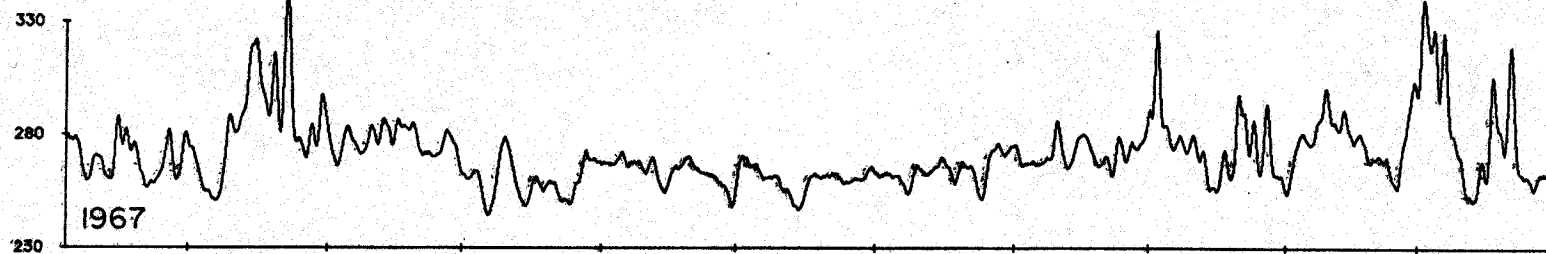
Low-passed Sea Level (cm)
