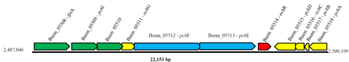
Figure S5. The organization of the predicted pyochelin gene cluster in B. seminalis TC3.4.2R3. Genes are oriented according to the direction of transcription. The clusters include genes encoding membrane proteins (green arrows), NPRSs (blue arrows), and other biosynthetic enzymes (yellow arrows). pchR (red arrow) encodes an AraC family transcriptional regulator.
