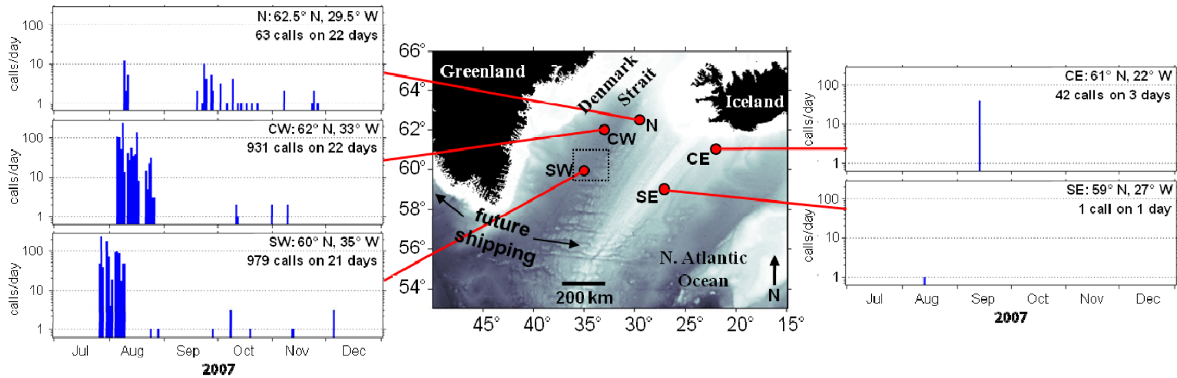
Fig. 1. Locations of passive acoustic moorings near Iceland and southern Greenland (red dots), and the number of right whale upcalls detected per day in late 2007 at the five sites. The rectangular dotted box is the approximate location of the Cape Farewell Ground, as defined by historical catches, and arrows indicate a shipping route that will open when the Northwest Passage becomes reliably ice-free. In ocean areas, depth of color indicates bathymetry.
