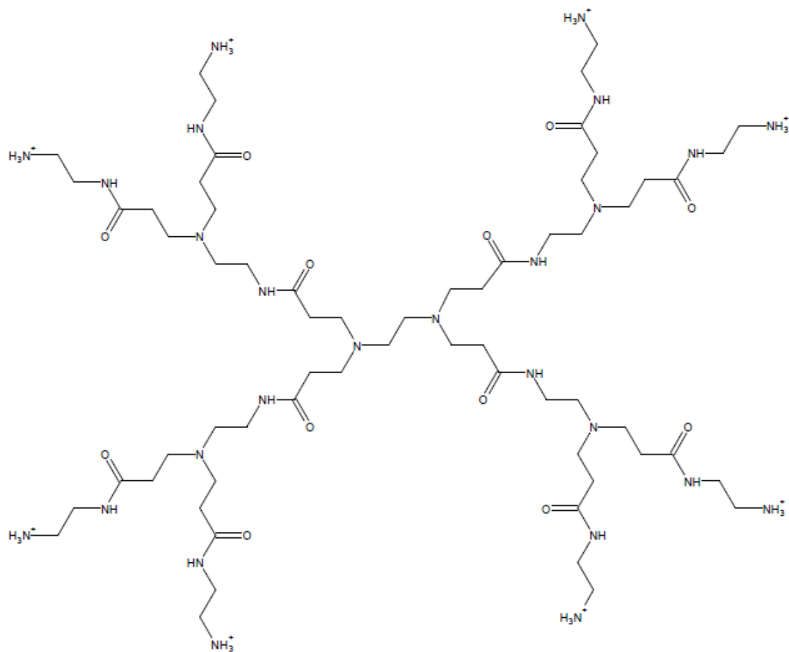
Figure 2: Chemical structure of generation 1 PAMAM dendrimer
