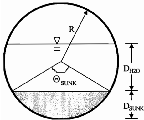
Figure 17: Circular culvert cross-section. From FishXing Help.
