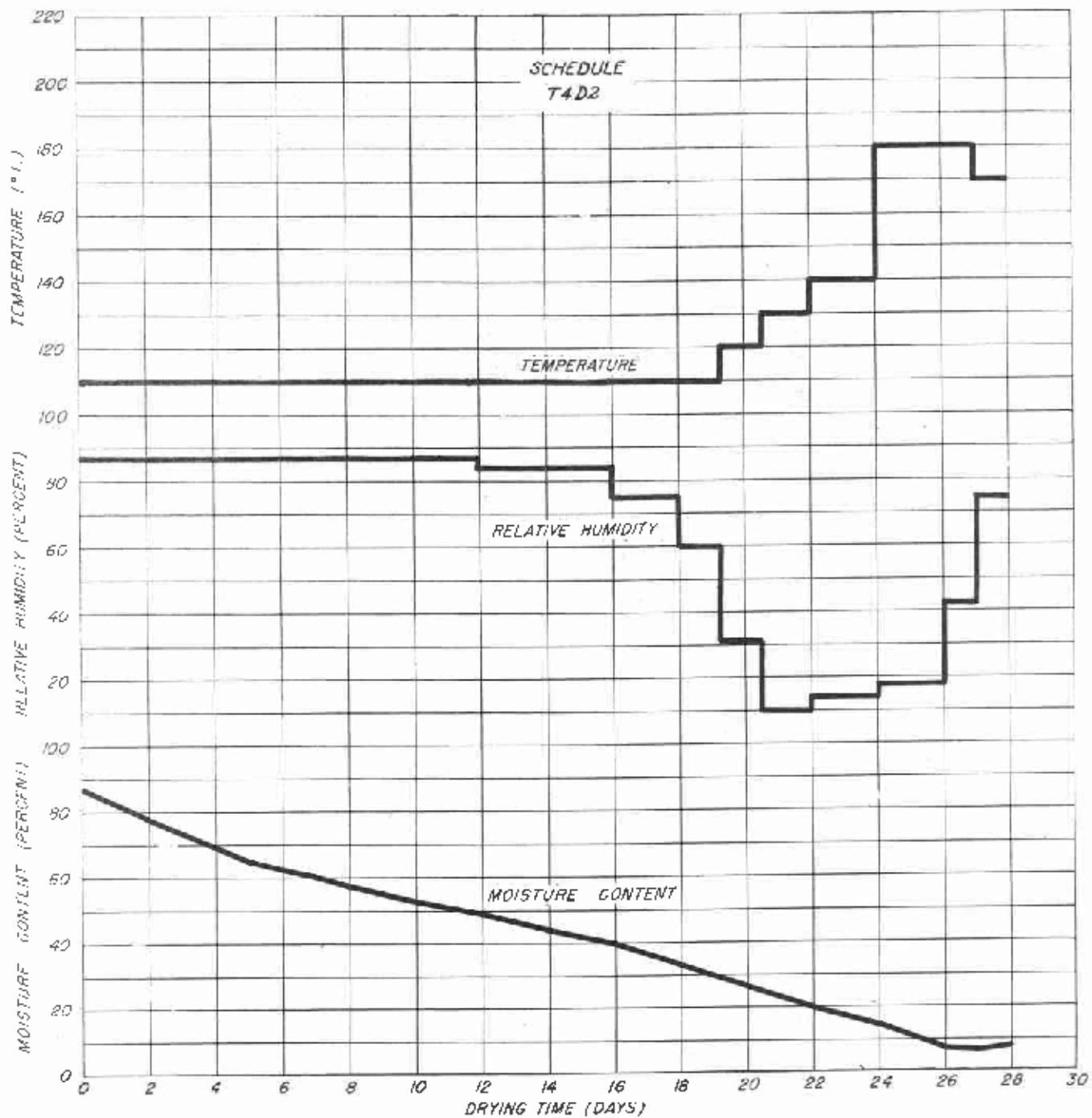
Figure 4. --Kiln conditions and drying curve 4/4 northern red oak, using new schedule T4-D2.
