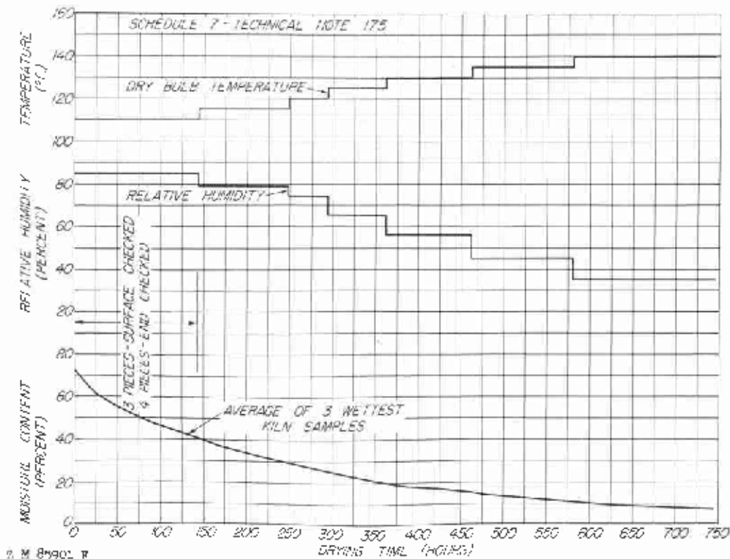
Figure 1. --Kiln conditions and drying curve, 4/4 northern red oak, using old Technical Note 175 schedule 7.
