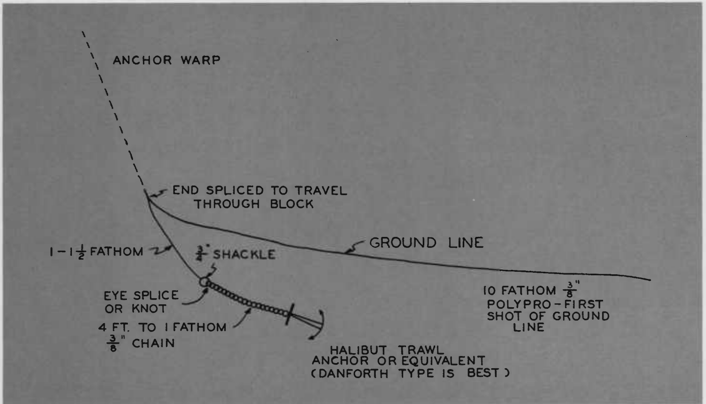
Figure 3. Anchor and ground line securing details.
