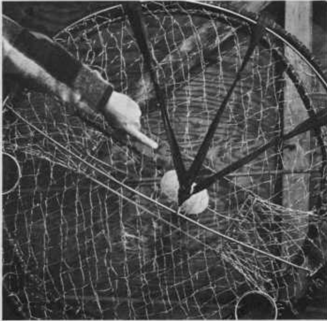
Figure 5B. Single-lid cover harness. New longline pots should have lid cover bar made halfway across the top to ease handling with single-lid cover retaining harness.
