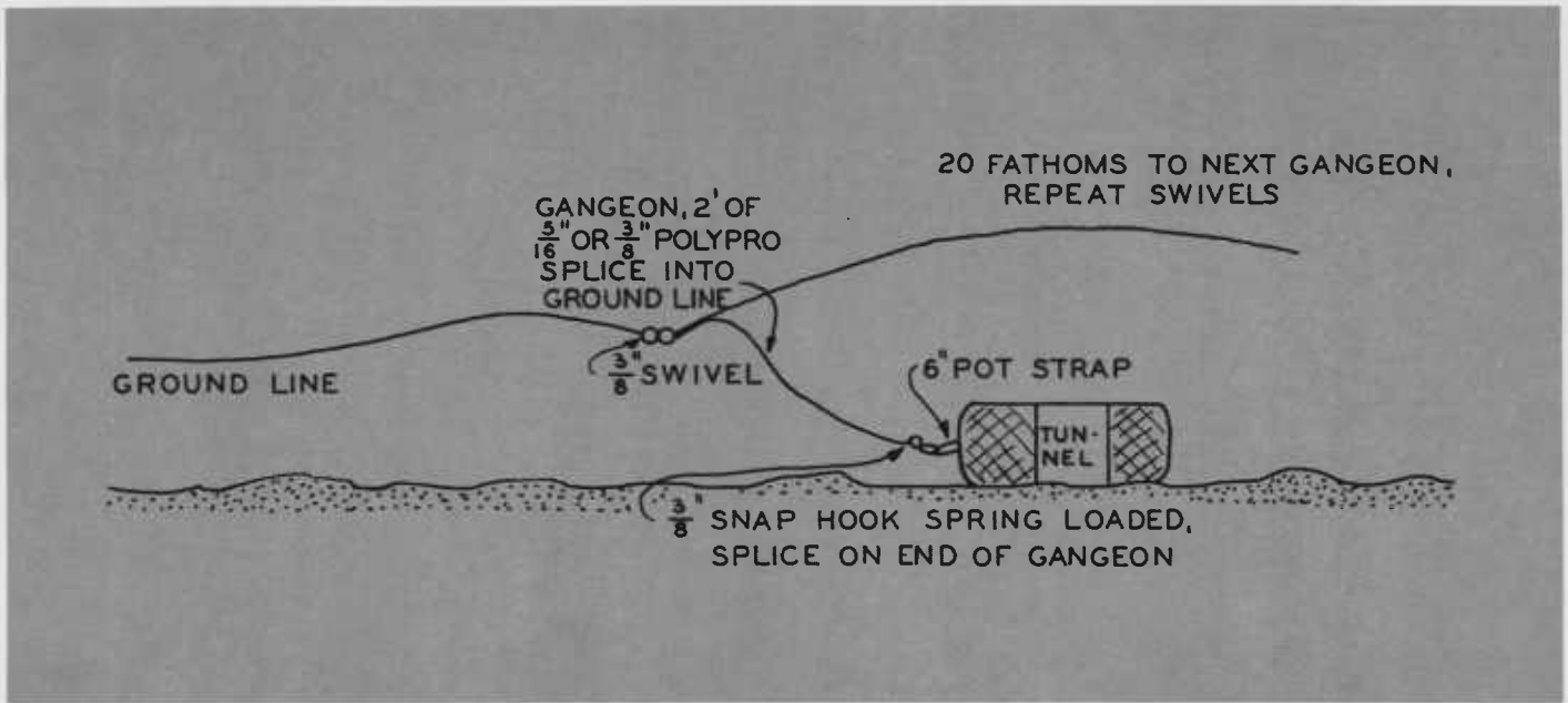
Figure 4. Gangeon and gangeon fastening details.
