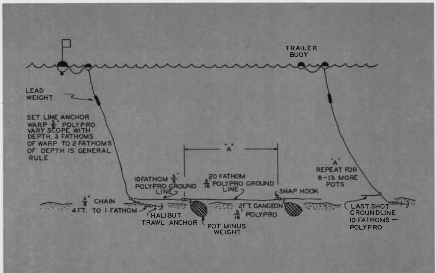
Figure 1. Overall sketch of Long-Line Crab Pot System.
