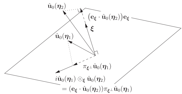
FIG. 1. Geometric interpretation of \hat{\mathbf{u}}_0(\boldsymbol{\eta}_1) \odot_{\boldsymbol{\xi}} \hat{\mathbf{u}}_0(\boldsymbol{\eta}_2) .
