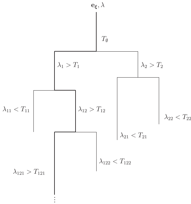
FIG. 2. Self-similar cascade with explosion cartoon.
