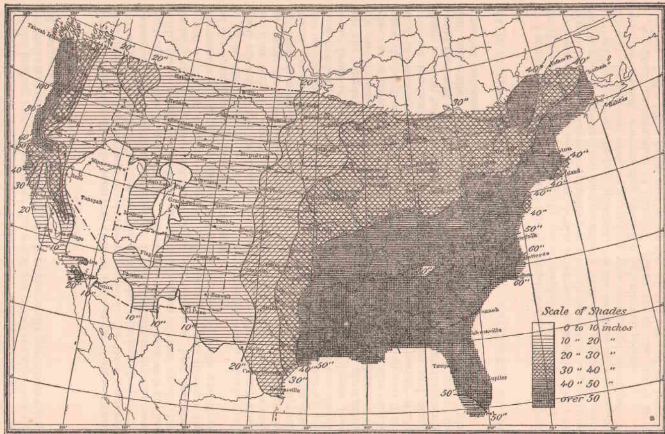
CHART B.—Annual precipitation.
