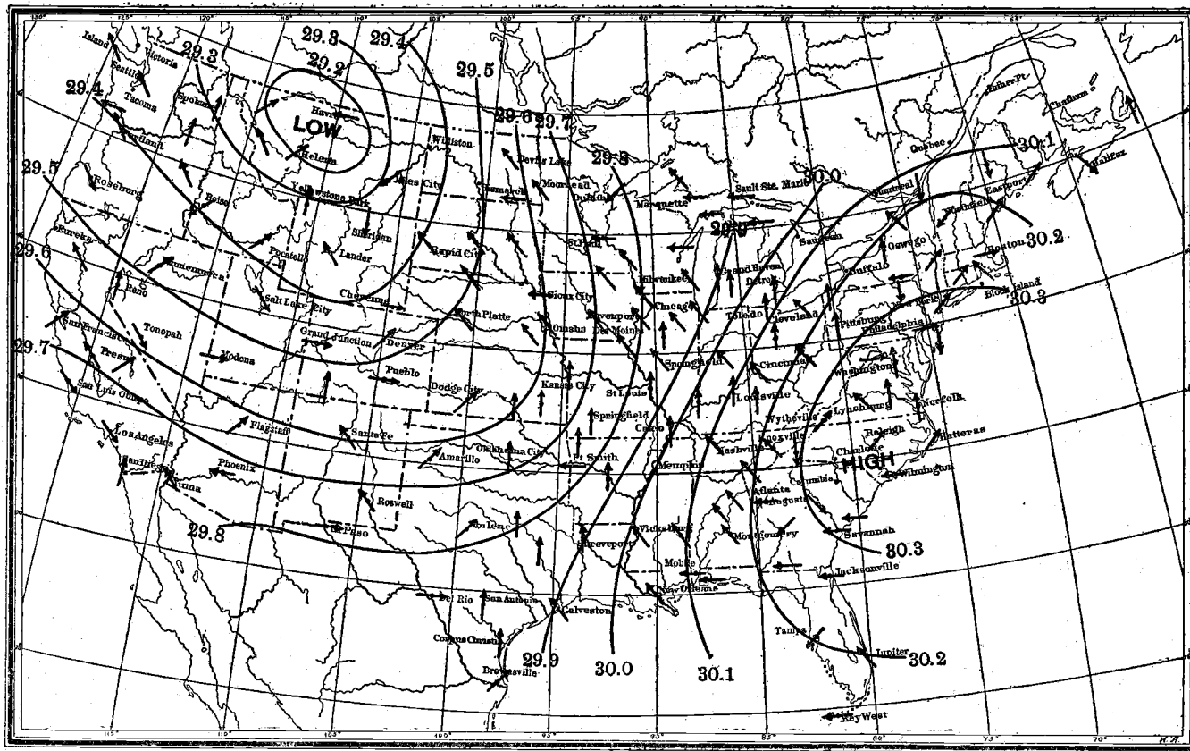
CHART A.—Arrows fly with the wind and show how the vaporous atmosphere of the Gulf of Mexico and the South Atlantic Ocean is drawn inland.
