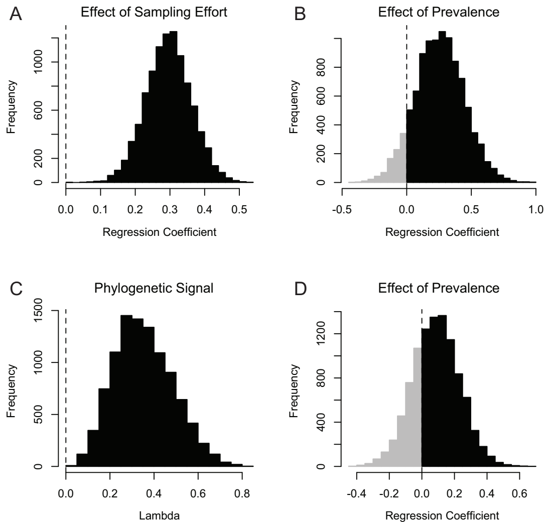
Figure 1: Parameter estimates (posterior probability distributions). Regression coefficients from the Markov chain Monte Carlo analysis of intracellular parasite richness regressed on sampling effort (A) and weighted helminth prevalence (B). In both cases, the analysis revealed support (“strong” in the case of sampling effort), with evidence for phylogenetic signal (C). Effects of weighted helminth prevalence were weaker in analyses of extracellular richness as the response variable (D). Black bars indicate positive values, gray bars negative values, and the dashed lines equal a value of zero.
