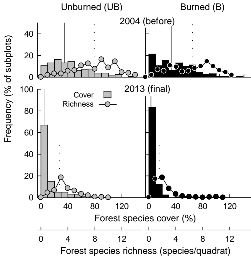
Fig. S4. Frequency distributions of forest understory species cover and richness before treatment (2004) and at final sampling (2013) among unburned (UB) and burned (B) subplots. Vertical lines are median cover (solid) and richness (dashed).
