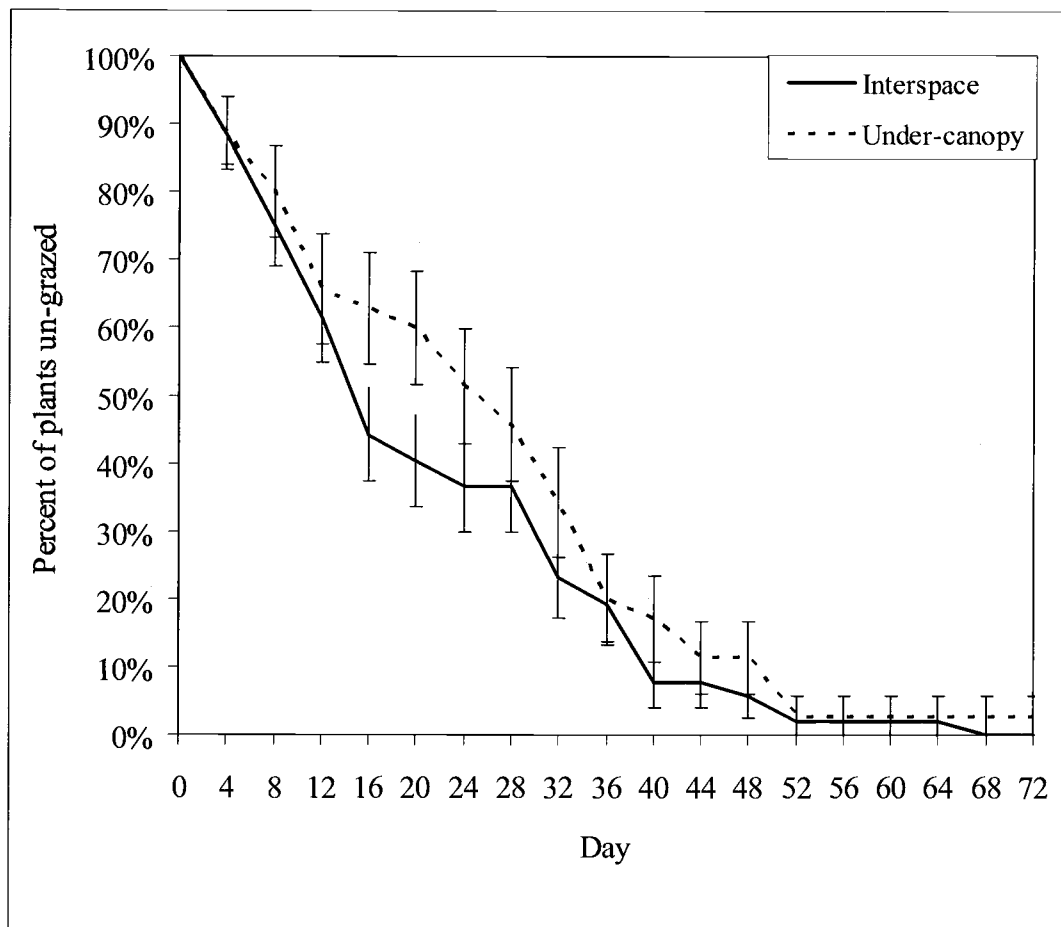
Figure 12: Life-test analysis evaluating cattle preference for interspace or under-canopy grass tussocks in an 800ha pasture at the Northern Great Basin Experimental Range, near Burns, Oregon in 2004.
