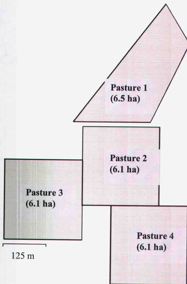
Figure 1: Four fenced pastures established for trial 1 at Foster Flat, Oregon, in which livestock grazed for 18 days for assessments of under-canopy and interspace utilization of grass tussocks in a Wyoming big sagebrush environment in 2003 and 2004.
