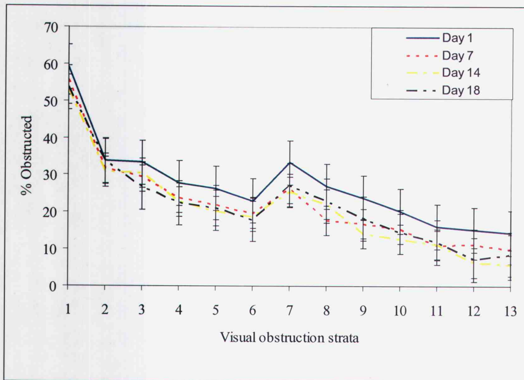
Figure 9: Percent visual obstruction for the random view for the 4 sampling times across the 13 strata (1 being the bottom and 13 being the top) of the Robel pole at Foster Flat, Oregon in 2004.
