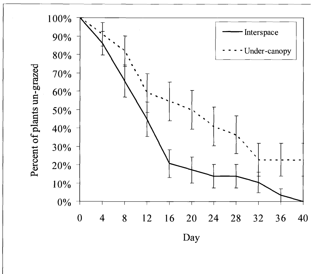
Figure 11: Life-test analysis evaluating cattle preference for interspace or under-canopy grass tussocks in an 800ha pasture on the Northern Great Basin Experimental Range, near Burns, Oregon in 2003.
