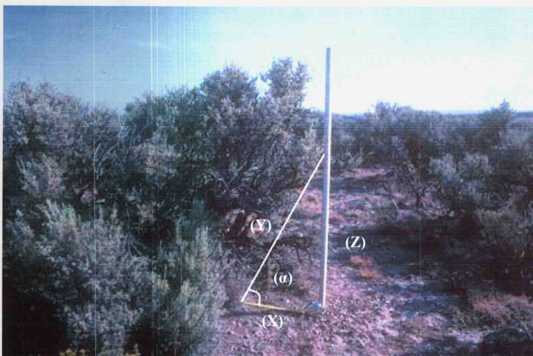
Figure 3: Angle of accessibility measurement to assess the vulnerability of under-canopy grasses to herbivory. Measurements were taken at the beginning of the trial for 2003 and 2004 at Foster Flat, Oregon.
