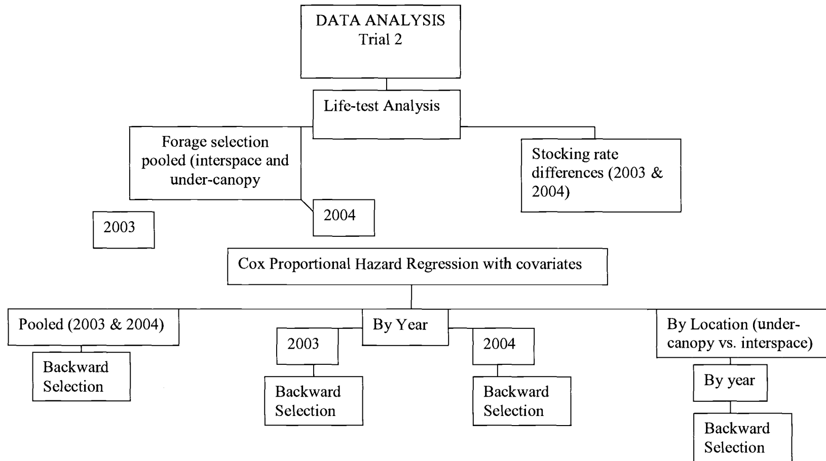
Appendix 1: Flow chart for analysis of trial 2 data, life-test analysis and survival regression analysis utilized to determine the effects of plant location, stocking density, and geo-physical variables at the Northern Great Basin Experimental Range, Oregon in 2003 and 2004.
