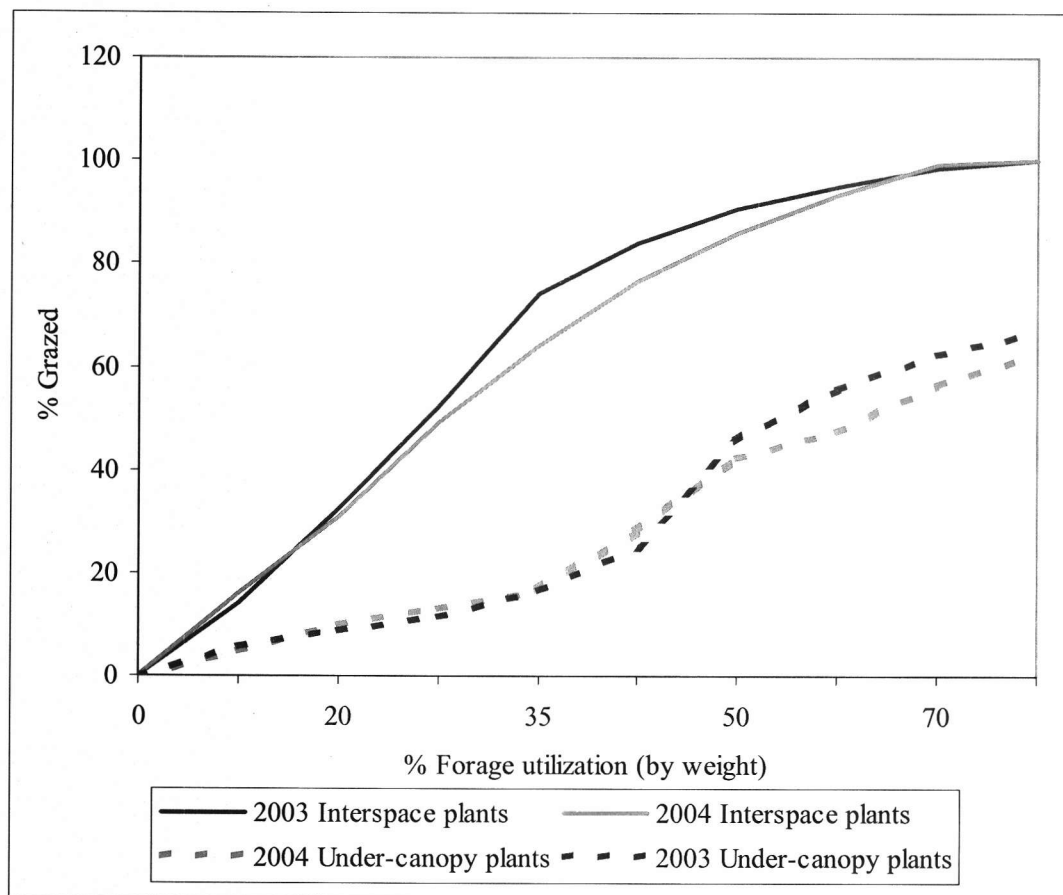
Figure 7: Percent of interspace and under-canopy plants grazed across pasture utilization for 2003 and 2004 at Foster Flat, Oregon for trial 1.
