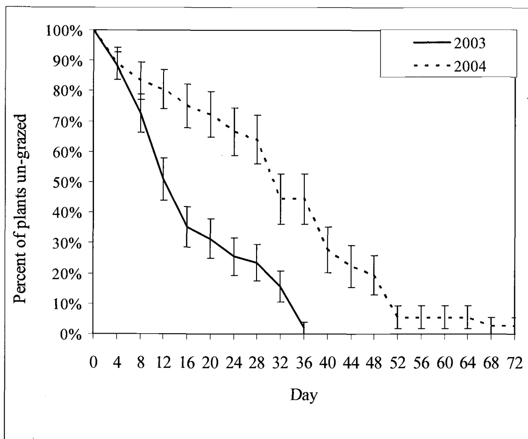
Figure 10: Life-test analysis of grass plants for trial 2 with different stocking rates (2003 180-cows, 2004 60-cows) at the Northern Great Basin Experimental Range, Oregon for 2003 and 2004.
