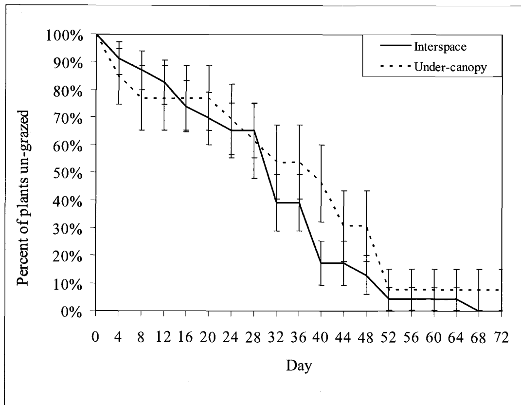
Figure 13: Life-test analysis evaluating cattle preference for interspace or under-canopy grass tussocks in an 800ha pasture on the Northern Great Basin Experimental Range, near Burns, Oregon with pooled data from 2003 and 2004.
