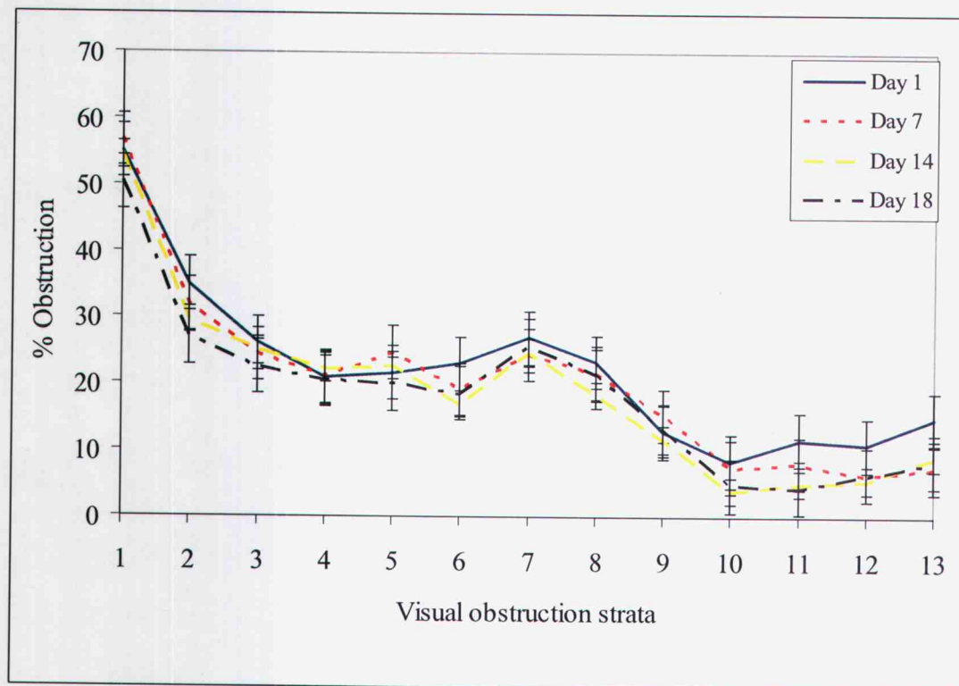
Figure 8: Percent visual obstruction for the unobstructed view for the 4 sampling times across the 13 strata (1 being the bottom and 13 being the top) of the Robel pole at Foster Flat, Oregon in 2004.
