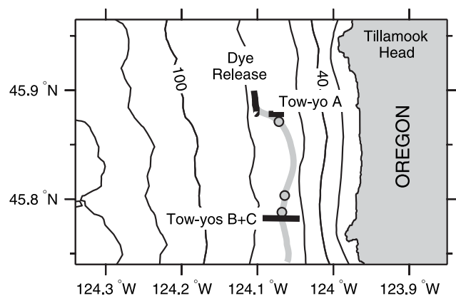
Figure 1. Bathymetry (contoured) of the northern Oregon shelf, showing (black) the location of the dye release and tow-yo lines, and (gray) the path of a 15-m drogued drifter released with the dye. Bullets show the drifter position at the mid-time of each tow-yo.
