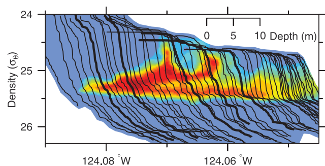
Figure 6. Stacked profiles of density against depth (inset axis) during tow-yo B. Individual profiles are offset by the ship longitude (main axis) at the time the CTD crossed \sigma_\theta = 25.29 . Homogeneous layers appear as horizontal steps. The underlying image is of dye concentration, similarly offset by depth and longitude. Bold profiles are those of Figure 4.
