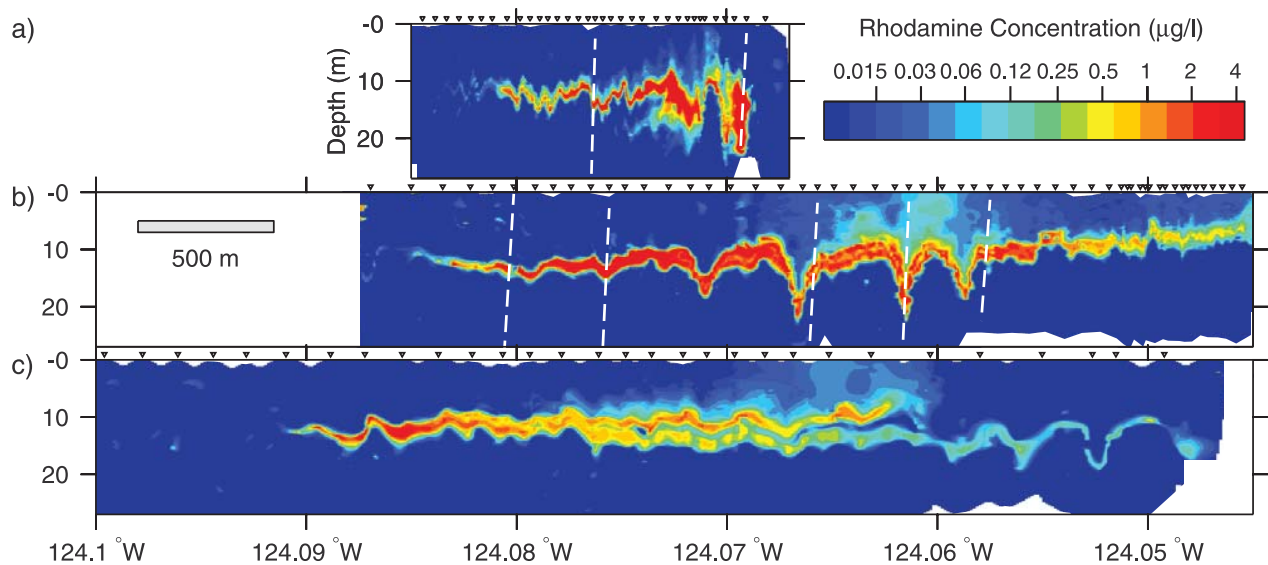
Figure 3. Cross-shelf sections of dye concentration from CTD tow-yos. Triangles on the upper axes show the start of each downcast. (a) Tow-yo A, (3.8–5.3 hours post-release), (b) Tow-yo B (12.9–14.7 hours), (c) Tow-yo C, (15.4–17.0 hours). Gridding was performed in ( x, \sigma_0 ) space then transformed to ( x, z ) space, a method that favors coherence of the gridded field along isopycnals. Dashed vertical lines show the profiles of Figure 4.
