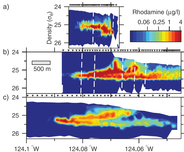
Figure 5. As Figure 3, but showing dye concentration vs density, from downcasts only.
