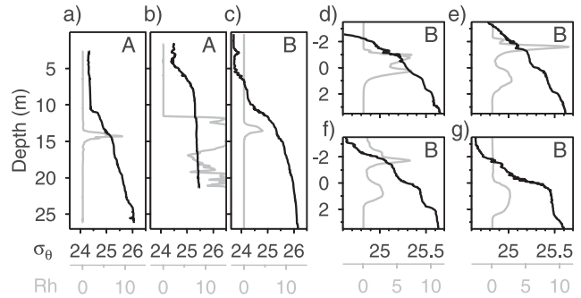
Figure 4. Profiles of potential density ( \sigma_0 ) (black) and rhodamine concentration ( \mu\text{g/l} ) (gray) from (a and b) two downcasts during tow-yo A (west-east) and (c–g) five during tow-yo B (west-east). Figures 4d–4g show an extract from the water column, with depth relative to \sigma_0 = 25.29 . Profile locations are shown in Figures 3 and 5.
