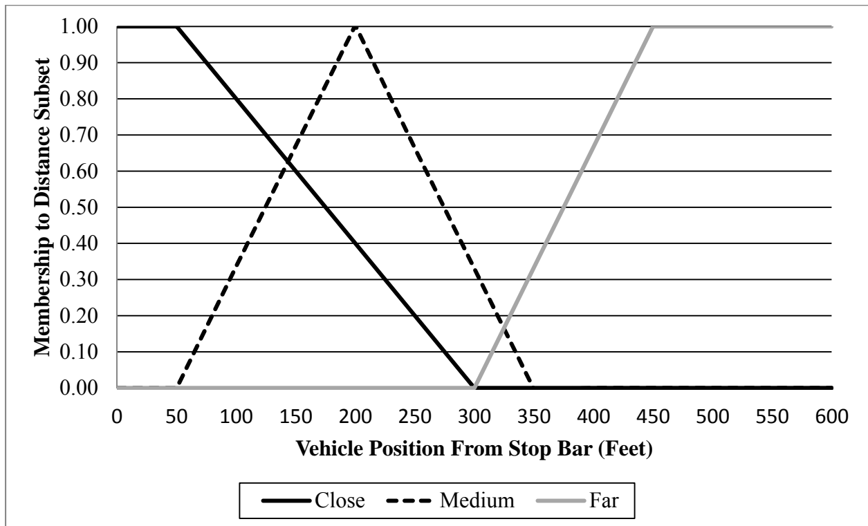
Figure 5 The Membership Function of Vehicle Position
