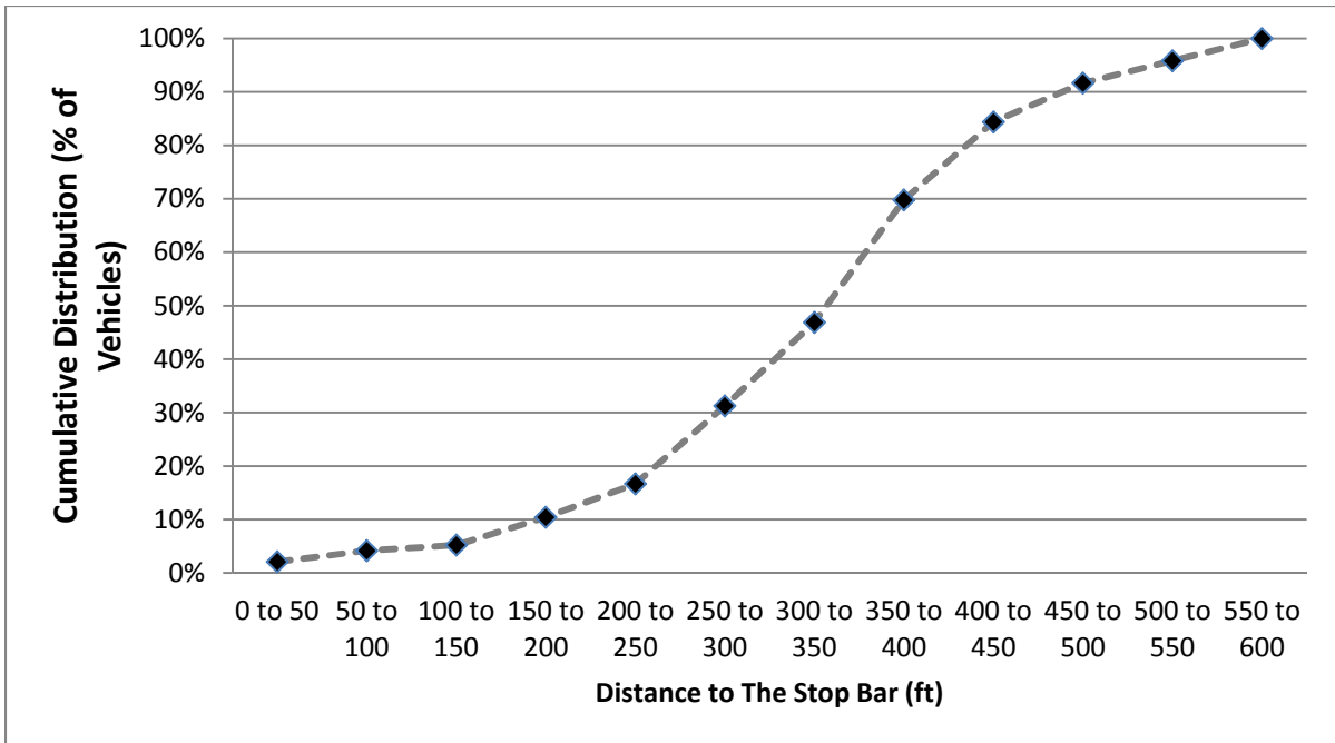
Figure 6 Cumulative Distribution of Driver Stopping Behavior: Route 7 @ North Shrewsbury (SB)
