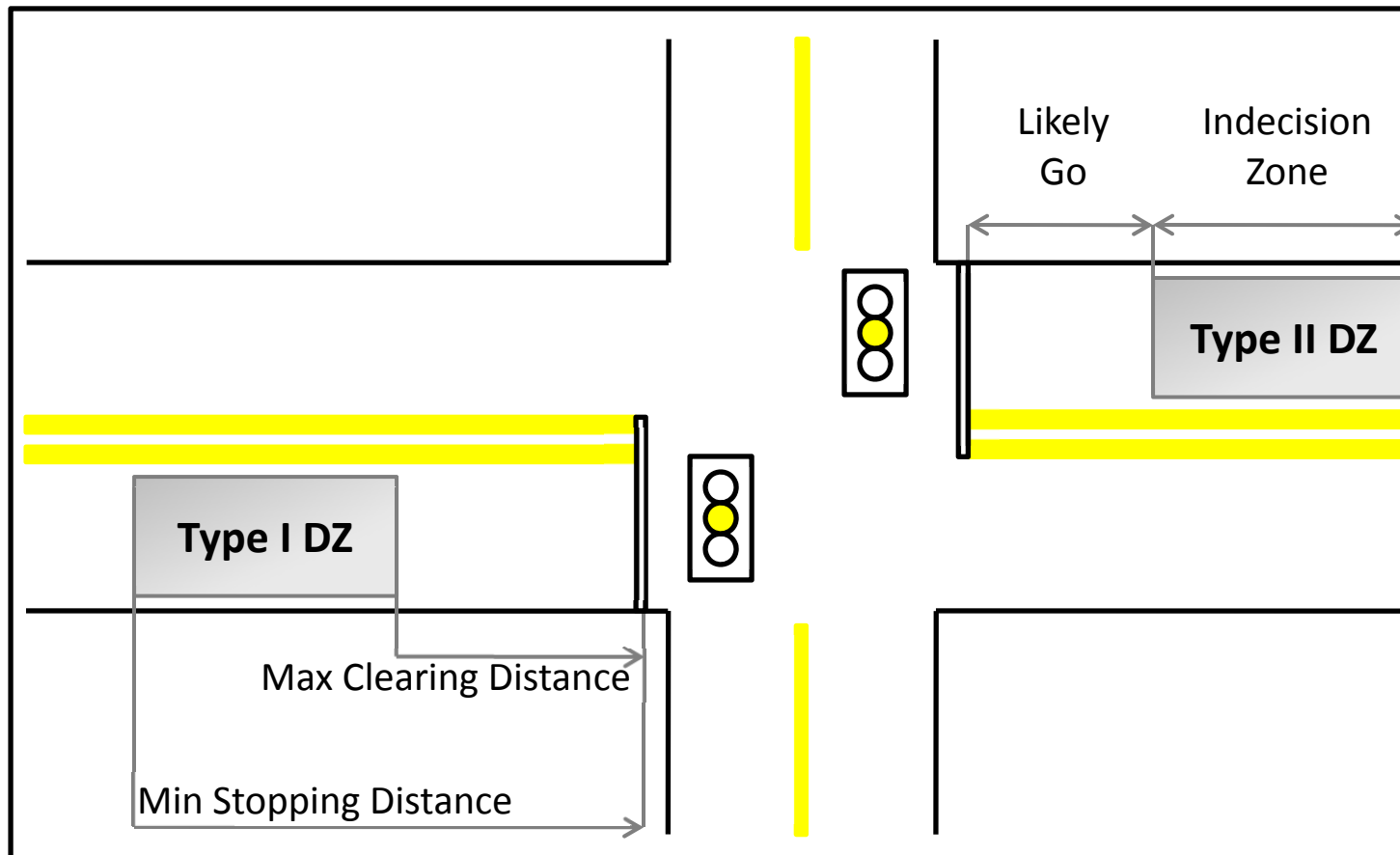
Figure 1 Type I & Type II Dilemma Zone Diagram
