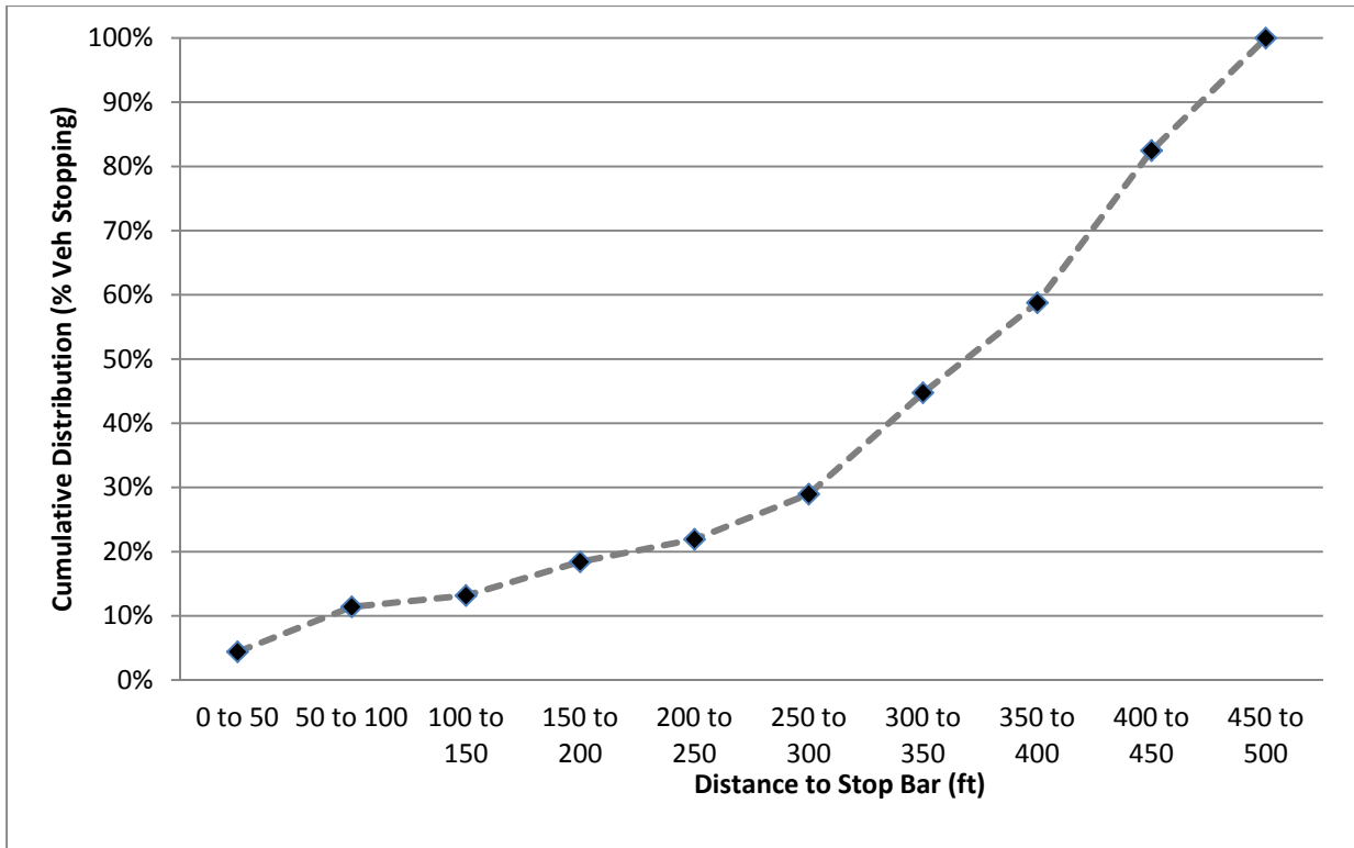
Figure 4 Cumulative Distribution of Driver Stopping Behavior: Route 62 @ Paine Turnpike (WB)
