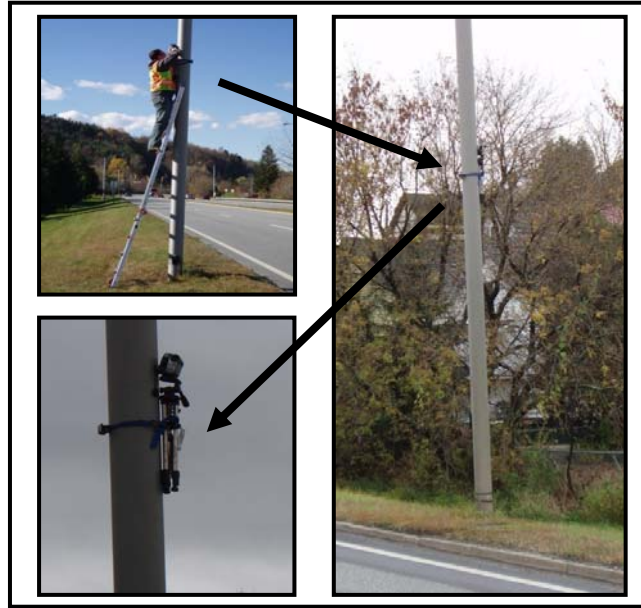
Figure 2 Example of Typical Video Camera Installation
