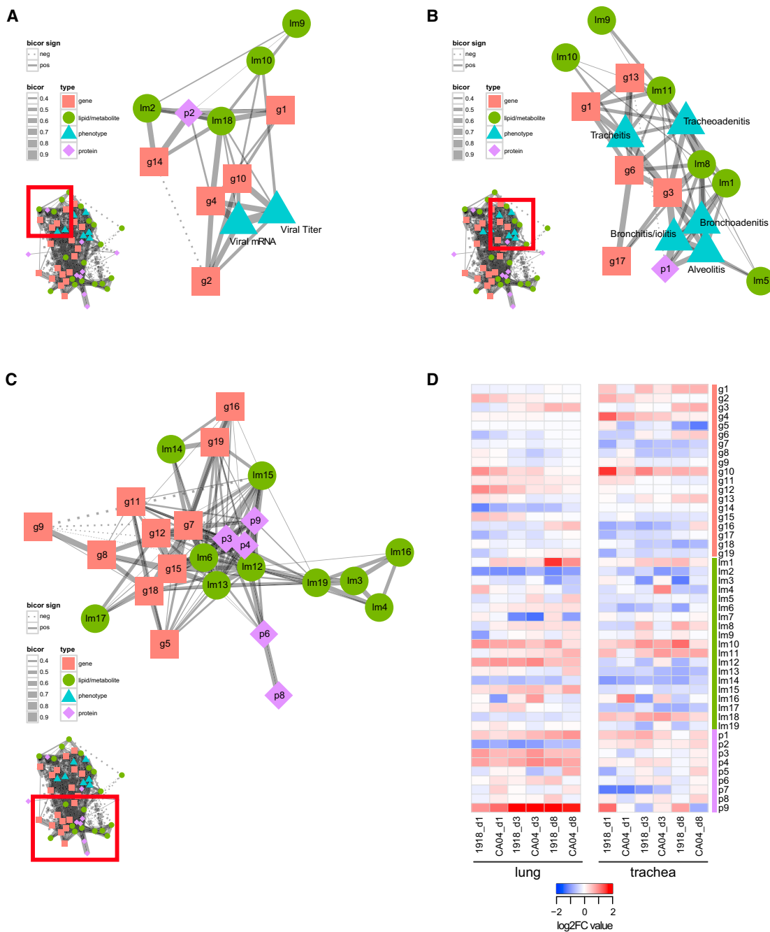
The integrated omics network related to (A) influenza virus replication, (B) respiratory disease, and (C) relationships among different molecular species. The integrated omics network was constructed by calculating pairwise correlations between modules from independent lipid and metabolite, protein, and gene networks and between all modules and phenotypic data. Nodes represent each module as a single point colored according to data type. Gene (g) modules are symbolized by pink squares. Lipid metabolite (lm) modules are symbolized by green circles. Protein (p) modules are symbolized by purple diamonds. Phenotype modules are symbolized by blue triangles. Edges between nodes signify biweight midcorrelation (bicor) coefficients between the representative expression profiles (module eigengenes, MEs) of all lipid and metabolite, gene, and protein module pairs with histopathologic and virologic phenotypes. Only significant correlations are shown ( p < 0.05 ). Positive bicor coefficients are represented by a solid line. Negative bicor coefficients are represented by a dashed line. The line thickness corresponds to the strength of the bicor coefficient (bicor 0.4–0.9). (D) Dynamics of module expression levels in different respiratory compartments (lung and trachea) and at different time points following infection with either 1918 or CA04 viruses. The heatmap depicts median log2FC values for each module across the experimental dataset. Rows are modules and columns are experimental conditions. See also Figure S3 .
