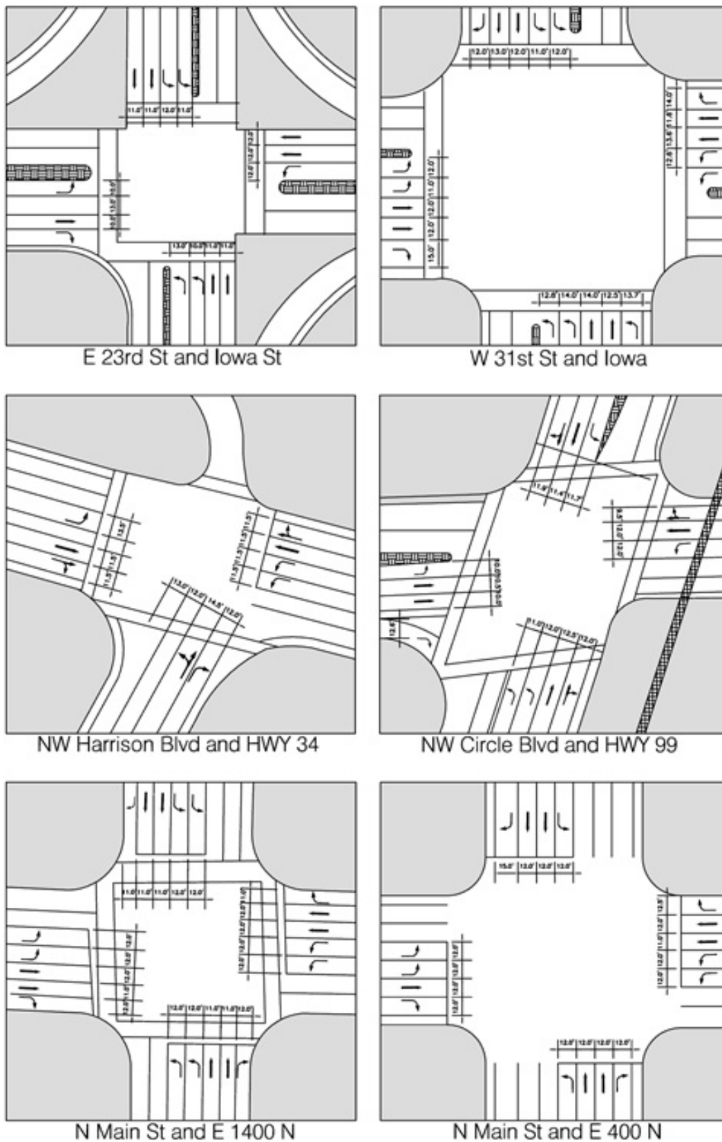
Fig. 1. Geometric Configurations of Observed Intersections
