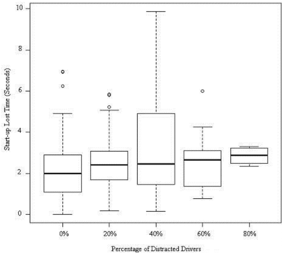
Fig. 4. Start-up lost time for 5 vehicle queues in all states
