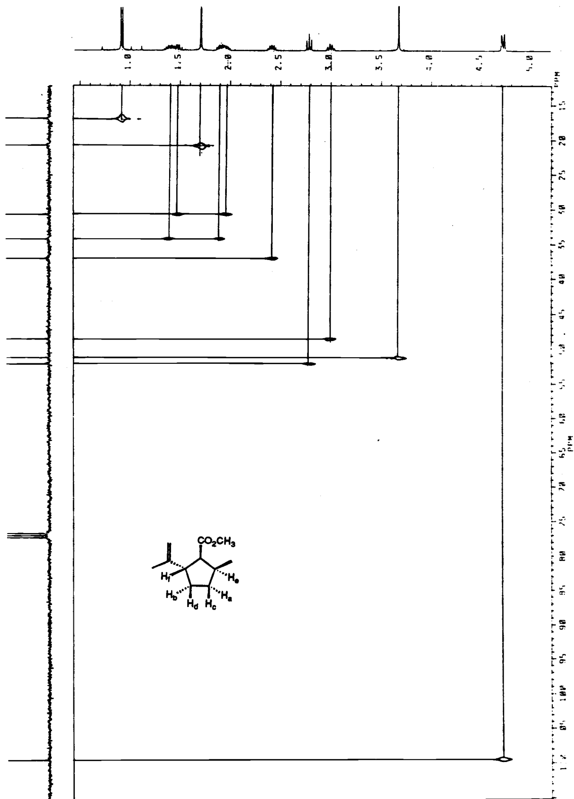
Figure 5. ^1\text{H} , ^{13}\text{C} HETCOR Spectrum of Methyl 2-isopropenyl-5-methylcyclopentanecarboxylate, 73 .
