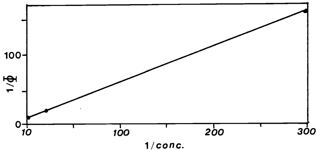
Figure 24. Quantum Yield Dependence of 97 from 71 vs [\text{conc.}]^{-1}
