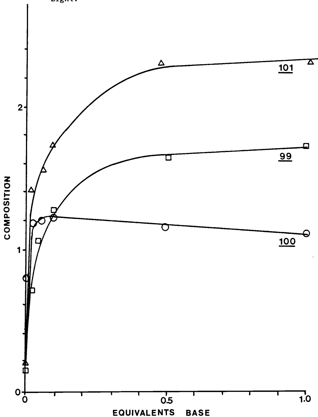
Figure 14. Equivalents of 1,2-DMI vs Relative Composition (a) for Irradiation of Methyl Geranate in Ether for 8 h with 254 nm Light.
