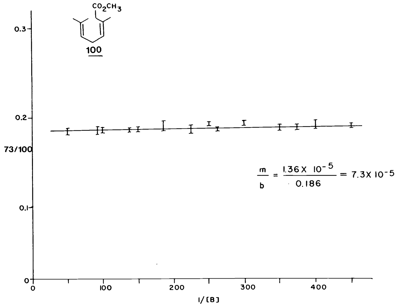
Figure 18. Relative Quantum yield of \underline{73/100} vs (1,2\text{-DMI})^{-1} .
