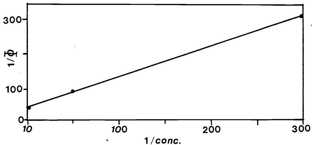
Figure 23. Quantum Yield Dependence of 92c from 92d vs [\text{conc.}]^{-1}
