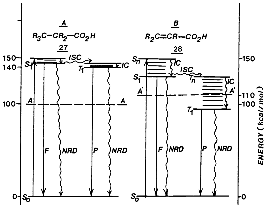
Figure 1. Energy Decay Pathways in \alpha,\beta -Unsaturated Acids and Saturated Acids.
