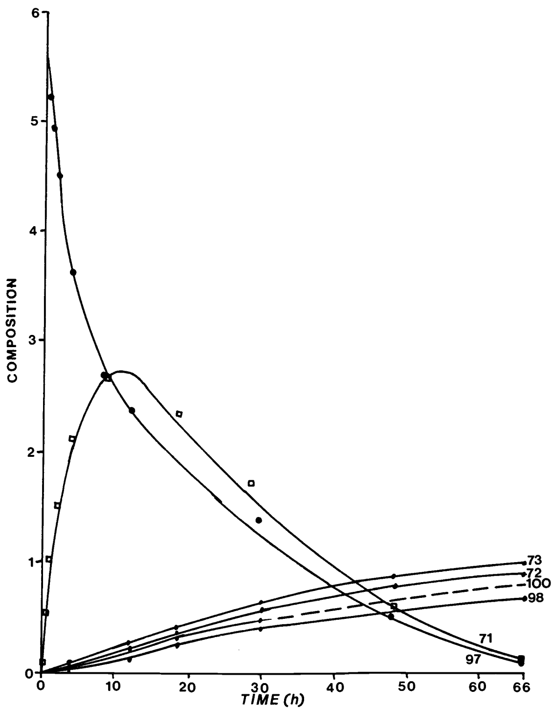
Figure 12. Irradiation Time Vs Relative Composition (a) for Methyl Geranate in Ether at 254 nm.
