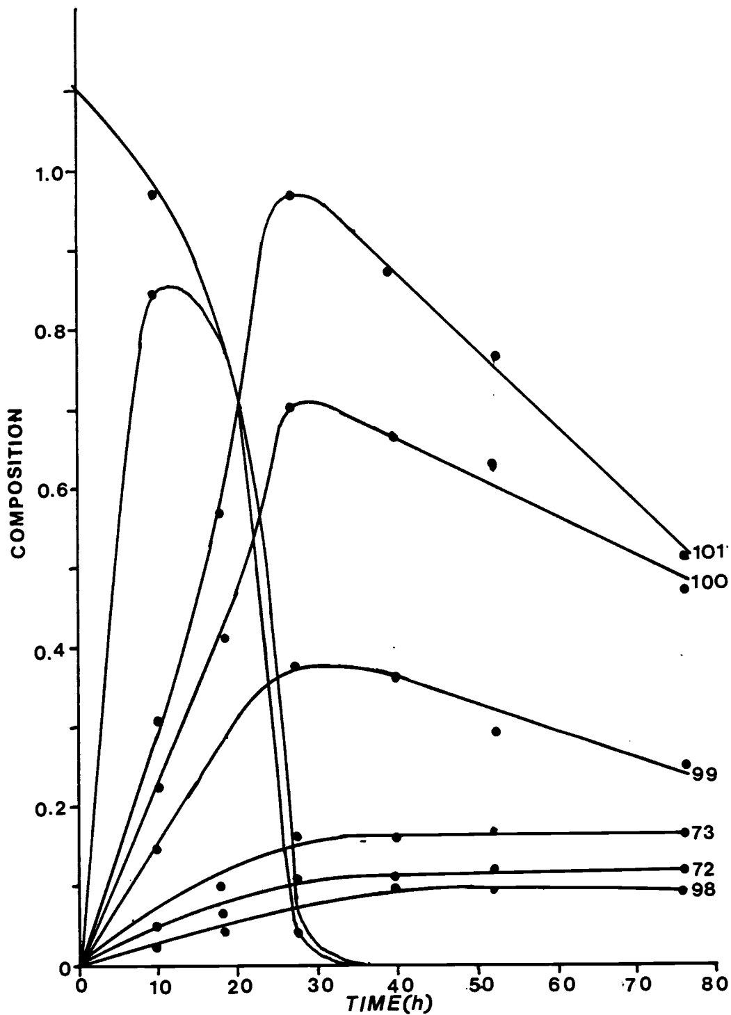
Figure 13. Irradiation Time vs Relative Composition (a) for Methyl Geranate in Ether with a Hanovia 450 Watt Medium Pressure Lamp.
