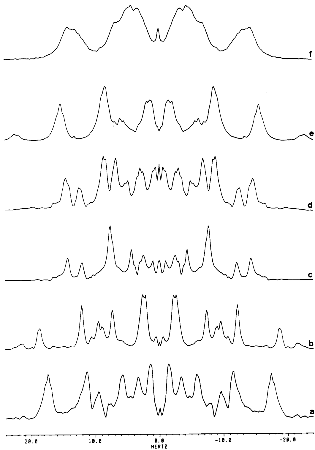
Figure 7. Projections in the f1 (Y) Axis of the JRES Spectrum of Methyl 2-isopropenyl-5-methyl cyclopentanecarboxylate, 73 .
