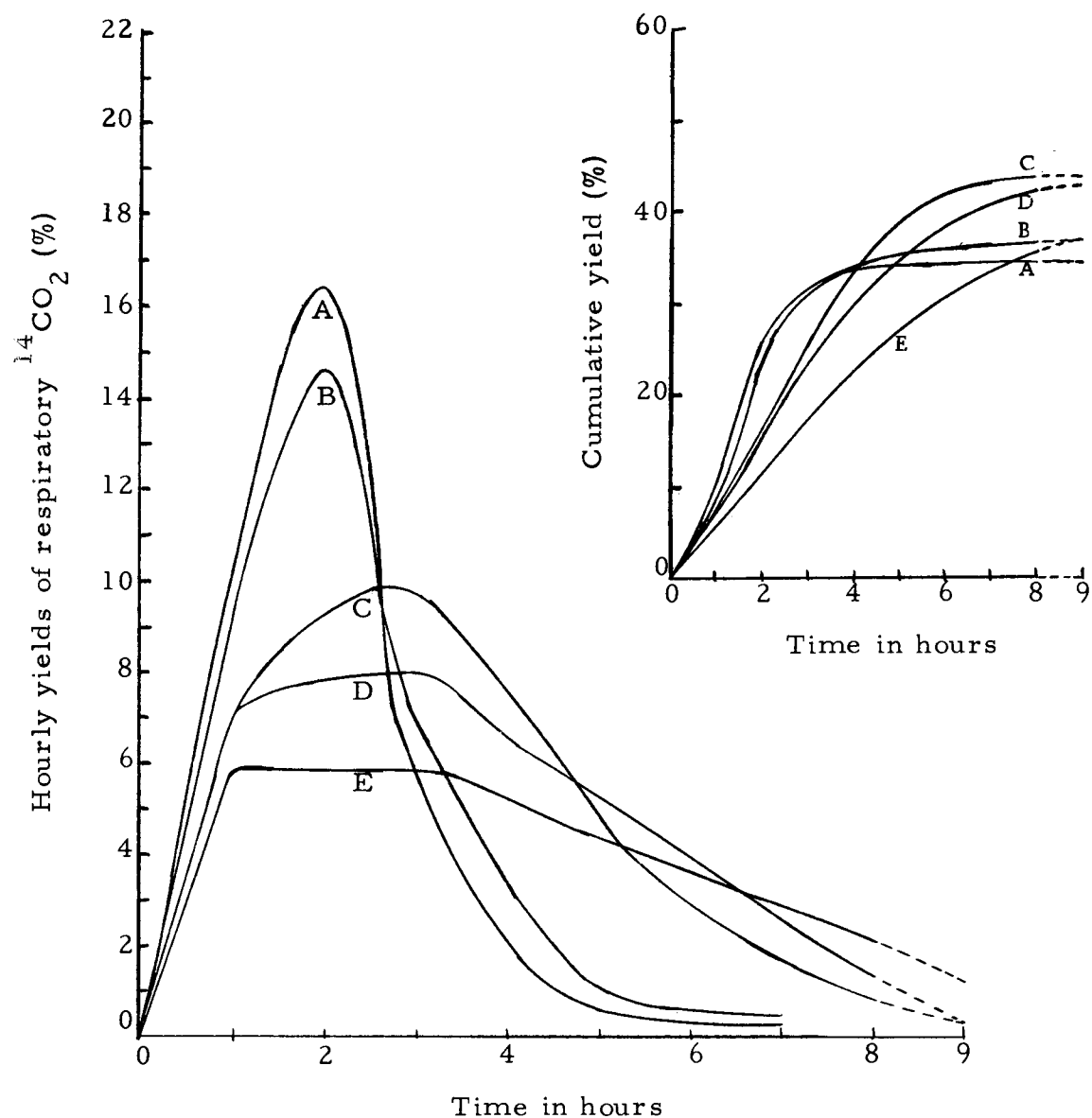
Figure 3. Radiorespirometric patterns for utilization of glucose by Saccharomyces cerevisiae cells in the presence of various amounts of 2-DG, single dose experiment. Experimental conditions: cell weight, 10 mg; volume of medium, 10 ml; substrate, 15 mg glucose-1- ^{14}\text{C} . The following amounts of 2-DG were added to the incubation medium: A -- 0.00 mg; B -- 0.16 mg (0.001 mmole); C -- 1.64 mg (0.01 mmole); D -- 8.20 mg (0.05 mmole); E -- 16.4 mg (0.10 mmole).
