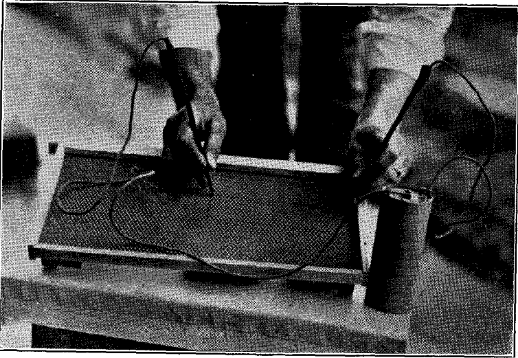
Fig. 6. A simple form of electrical imbedder. A small transformer may be used and is more economical when electrical current is at hand.
