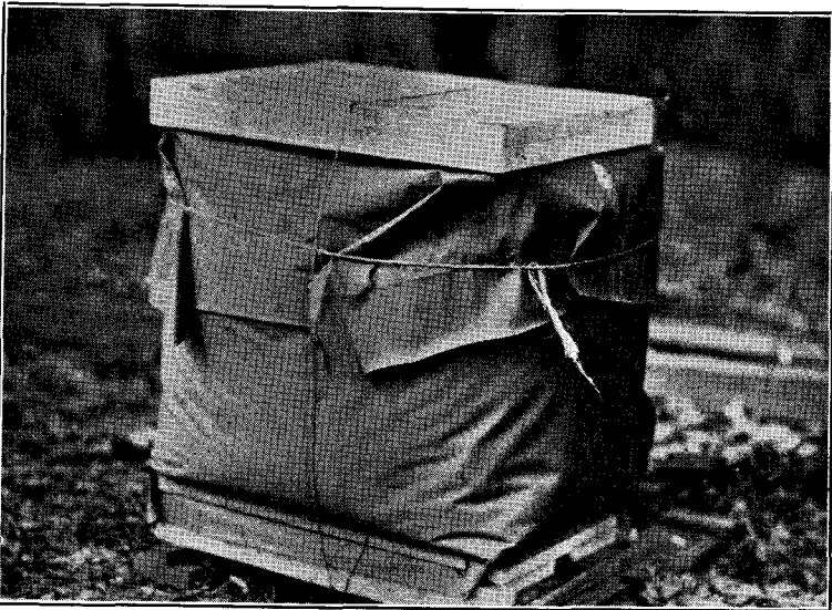
Fig. 9. A good substitute for a winter packing-case made from tarred building paper, with a packing of shavings underneath. Since the paper must be supplied new each season this method is no more economical than a good packing-case and is less convenient and efficient.
