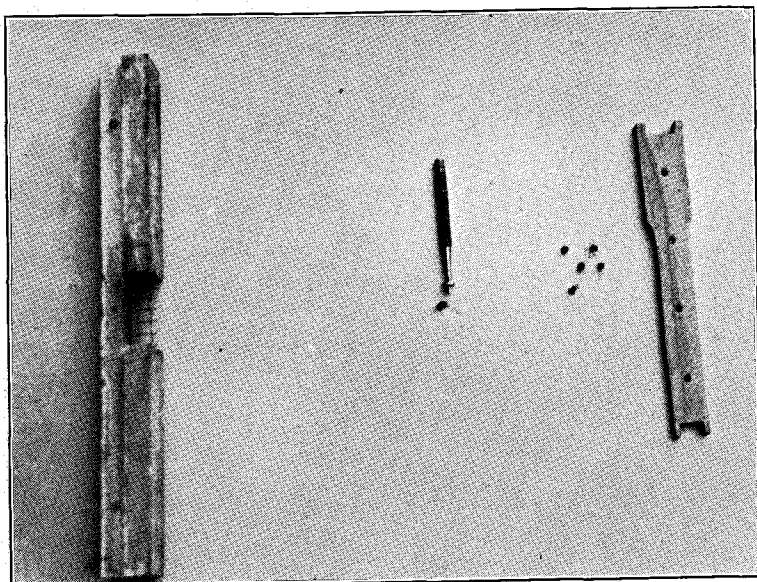
Fig. 10. To the right is shown how eyelets may be conveniently inserted in frames to prevent the wire cutting into the wood. A common nail-set with a small nut on the end is used to drive in the eyelet. To the left is shown a mouse-proof entrance guard which is important for protection against mice during the fall and winter.
