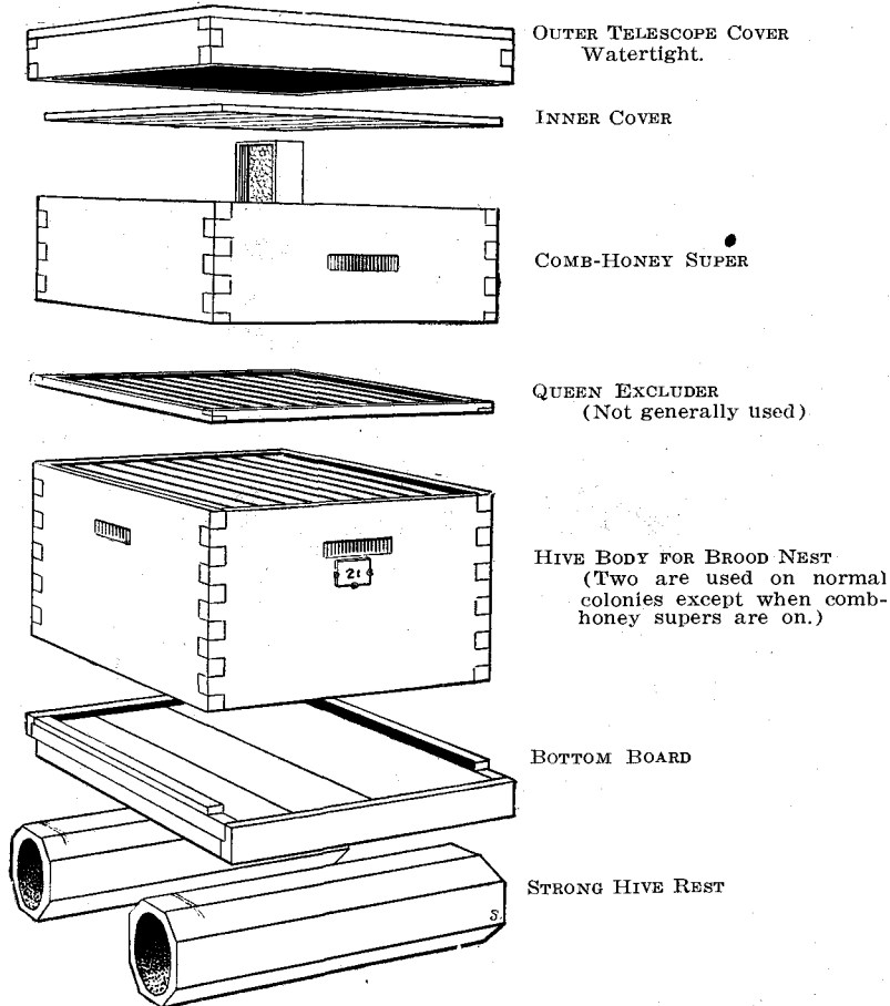
Fig. 1. A ten-frame hive with comb-honey super
