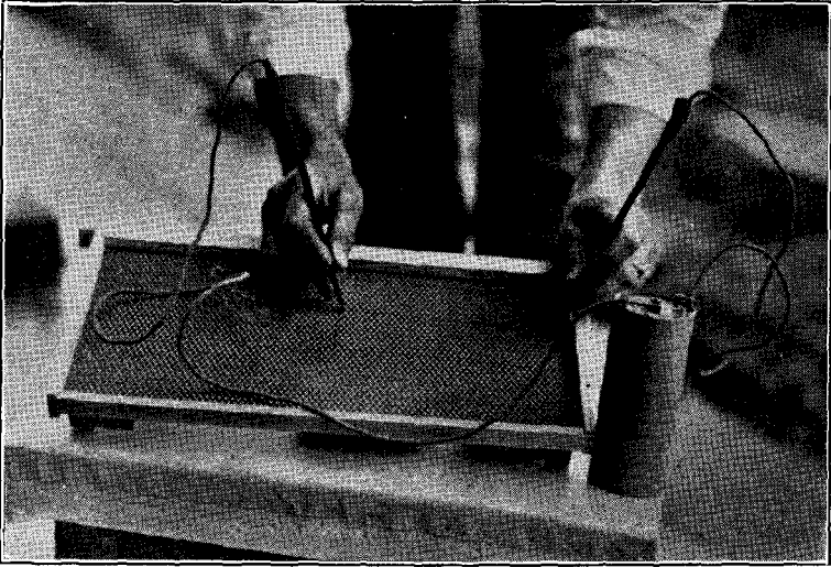
Fig. 6. A simple form of electrical imbedder. A small transformer may be used and is more economical when electrical current is at hand.
