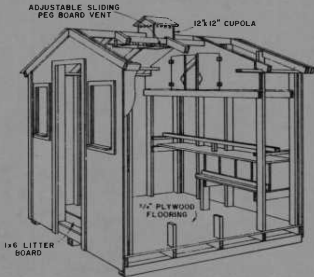
CUTAWAY VIEW OF 8'x8' LAYING HOUSE
