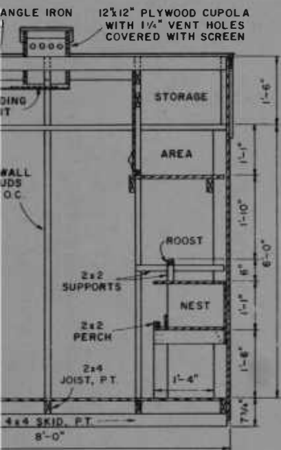
SECTION LAYING HOUSE
