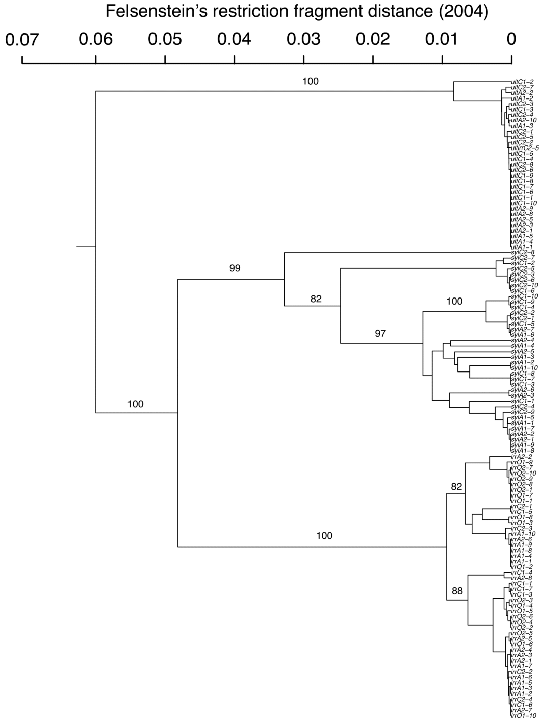
eXtra Fig. 2. UPGMA tree of P. irregulare , P. sylvaticum , and P. ultimum based on Felsenstein's restriction fragment distance of the primer AT-T. Branches with >70% bootstrap support are labeled.
