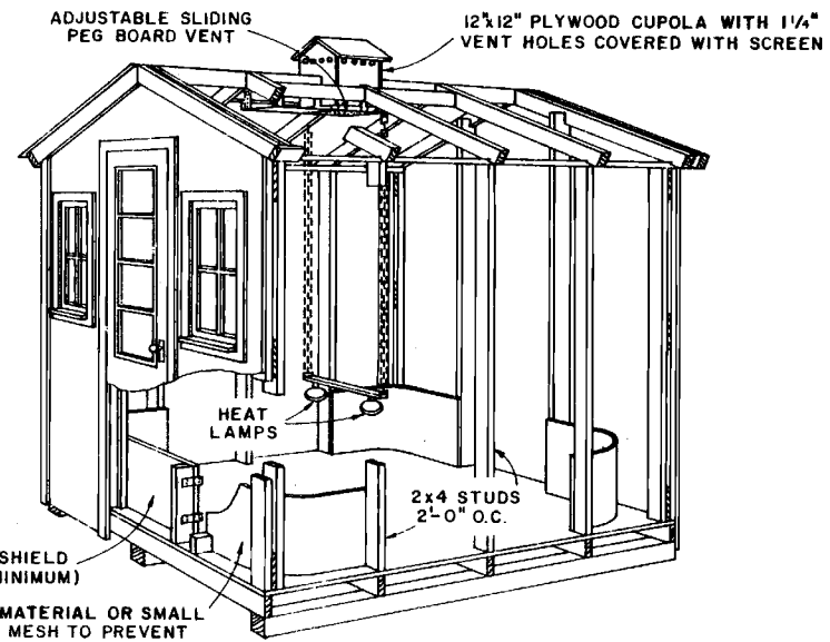
CUTAWAY VIEW OF 8x8 BROODER HOUSE
