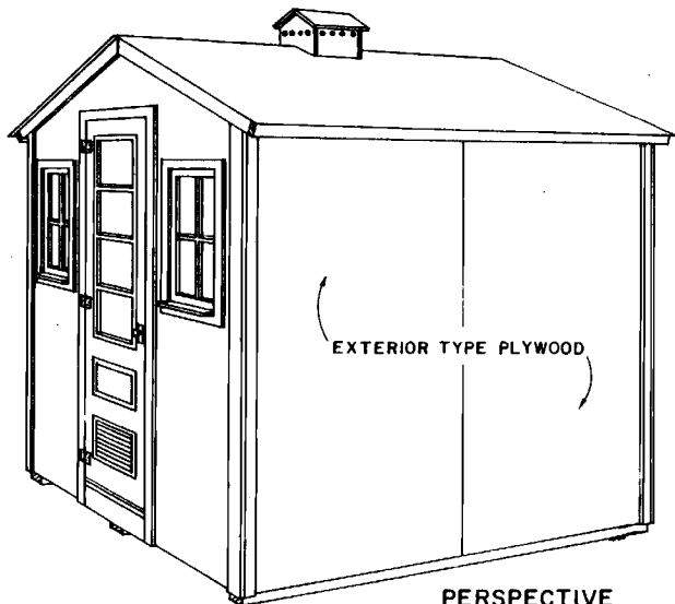
PERSPECTIVE BROODER HOUSE LAYING HOUSE
